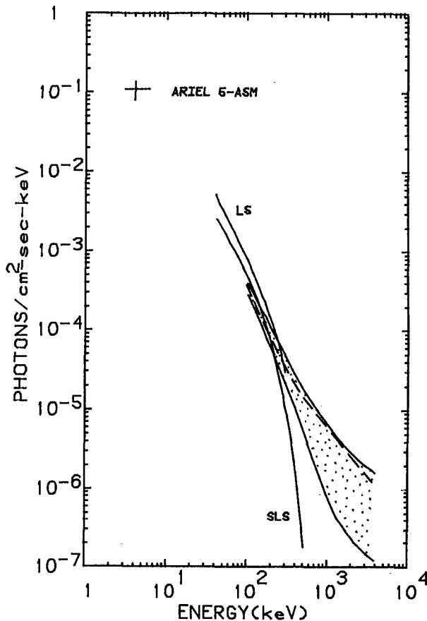
FIG. 1.—Differential photon spectrum of Cyg X-1 derived from the OPALE data (hatched area). The 3-6 keV flux measured in the contemporary Ariel 5 ASM observation (7) is also indicated, as well as the best fit Comptonization model spectrum to the LS and SLS hard X-ray data (solid line), and the best composite fit (Comptonization plus power law) spectrum to the OPALE data (broken line).
