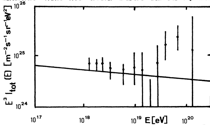
Fig. 2. The total flux (multiplied by E^3 ) calculated from \langle \sin b^{\parallel} \rangle as a function of energy.
