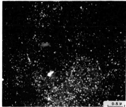
Figure 6. - Typical microcrystalline \beta -NiMo regions seen in eutectic (near wheel side) and hypereutectic (near wheel side) alloy ribbons.
