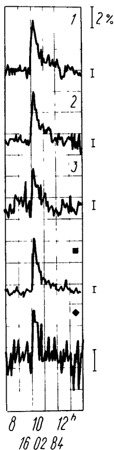
Fig.2. Results of recording the 16 February 1984 SCR flare from five-minute duration measurements with the Sayan spectrograph and the instrument 6HM-64-selector. 1, 2, 3 - neutron component as measured by standard neutron monitors at 3000, 2000 and 435 m, respectively; \blacksquare \blacklozenge - multiple neutrons as measured at 3000 m according to the discrimination criterion of m \geq 1 and m \geq 2 , respectively (measurement errors are shown at right).
