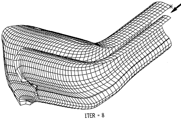
ITER = 8
