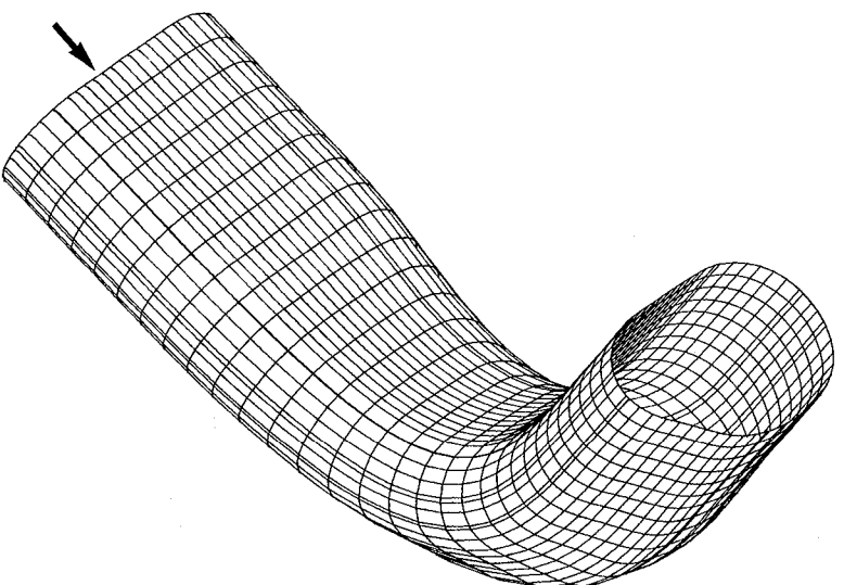
Complex (genera)
