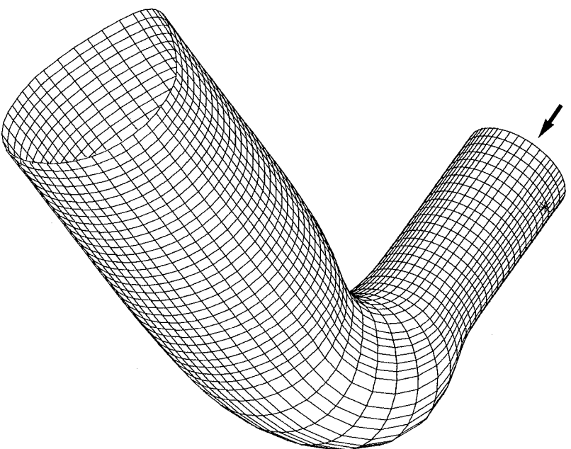
Simple (circle)
