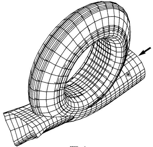
ITER = 6
