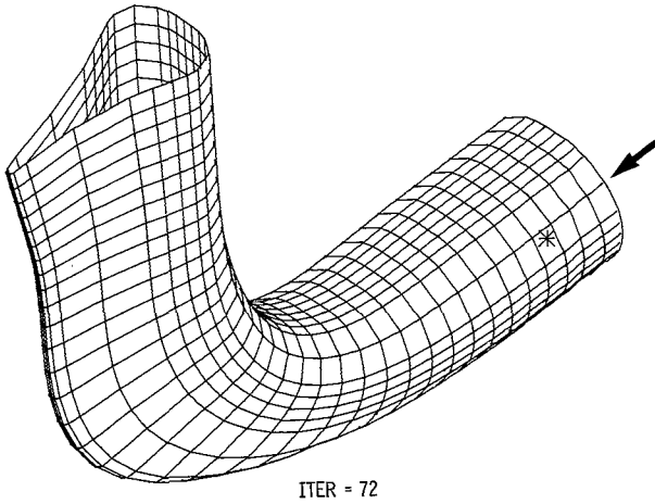
ITER = 72
