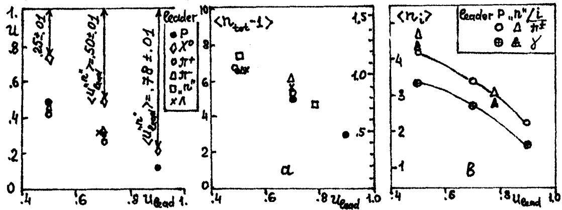
Fig.1. A fraction of the measured energy in the events with different leaders (a) and the total multiplicity of the attending particles of species i (b) for different leaders (c)
