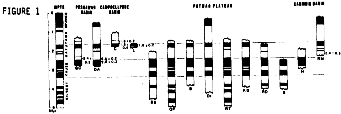
Comparisons of locally determined magnetic-polarity stratigraphies (MPSs) with the magnetic-polarity time scale 41,42 . Fission-track dates on volcanic ashes are shown with 2\sigma errors at their appropriate stratigraphical positions. The magnetostratigraphical correlations are based on recognition of identifiable chrons or subchrons and are aided by both fossil occurrences and the frequent presence of prominent ashes straddling the Gauss-Matuyama transition.
