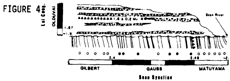
The northern limb of the Soan Syncline, where nearly vertical strata of typical Siwalik molasse sediments are truncated and overlain by the generally underformed Lei conglomerate. Only the upper portion of >3,000 m of molasse sediments is shown. \Delta , Enclosed volcanic ashes. The magnetostratigraphy 31 indicates that these strata encompass the Gauss chron and that the youngest preserved sediments extend into the lower Matuyama chron, probably to \sim 2.1 Myr. The overlying Lei conglomerate includes an ash dated at 1.6 \pm 0.2 Myr (ref. 29) on the basis of which the normal-polarity magnetozone is interpreted as the Olduvai subchron. The base of the Lei conglomerate must predate the Olduvai and is interpreted as \sim 1.9 Myr. Thus, between 2.1 and 1.9 Myr ago, >3,000 m of uplift and erosion (mean minimum rate of 15 \text{ mm yr}^{-1} ) occurred as the Soan Syncline was strongly compressed in response to thrusting along the MBT.
