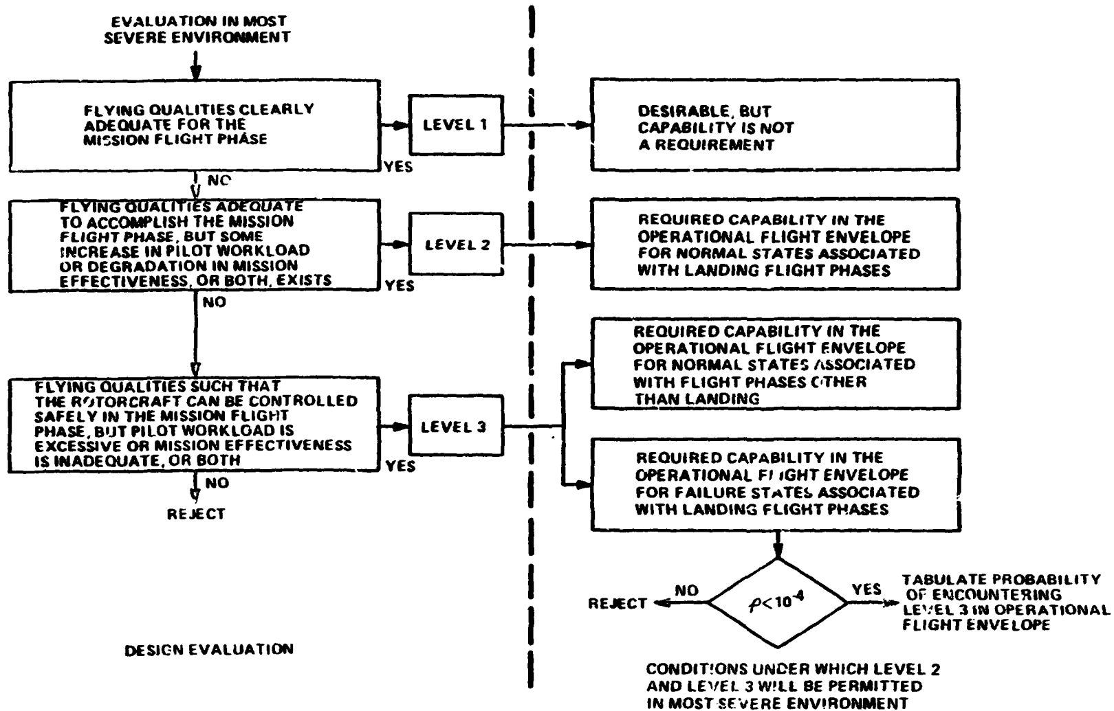
Figure 2.4-5 DEFINITION OF CONDITION UNDER WHICH LEVEL 2 AND LEVEL 3 FLYING QUALITIES WILL BE PERMITTED IN THE MOST SEVERE ENVIRONMENT
