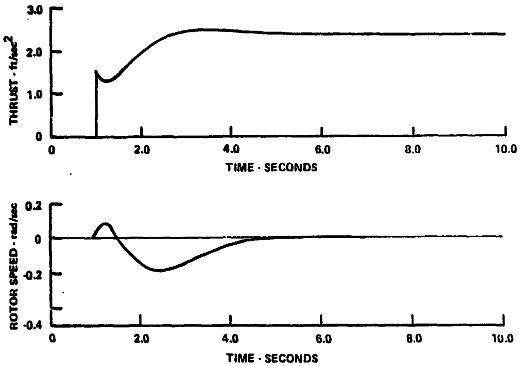
Figure 27 ROTOR THRUST SPEED RESPONSE TO COLLECTIVE COMMAND - COLLECTIVE PITCH FEEDFORWARD COMMAND EQUAL TO 67% OF "IDEAL" GAIN
