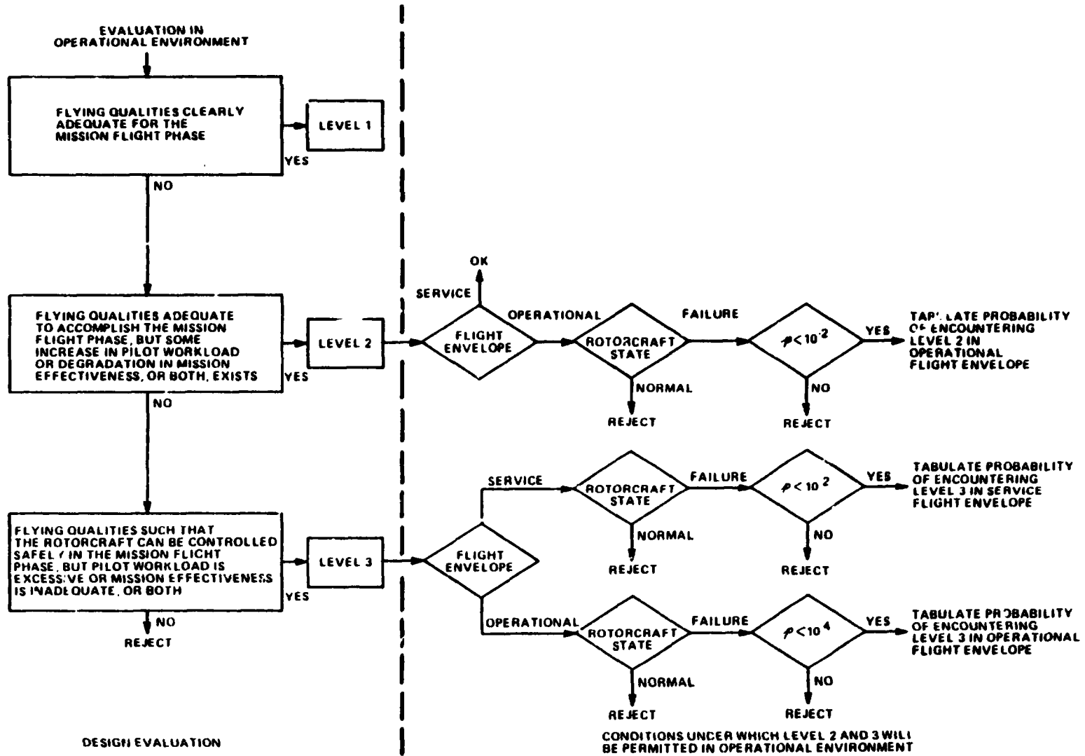
Figure 1 DEFINITION OF CONDITIONS UNDER WHICH LEVEL 2 AND LEVEL 3 FLYING QUALITIES WILL BE PERMITTED IN THE OPERATIONAL ENVIRONMENT
