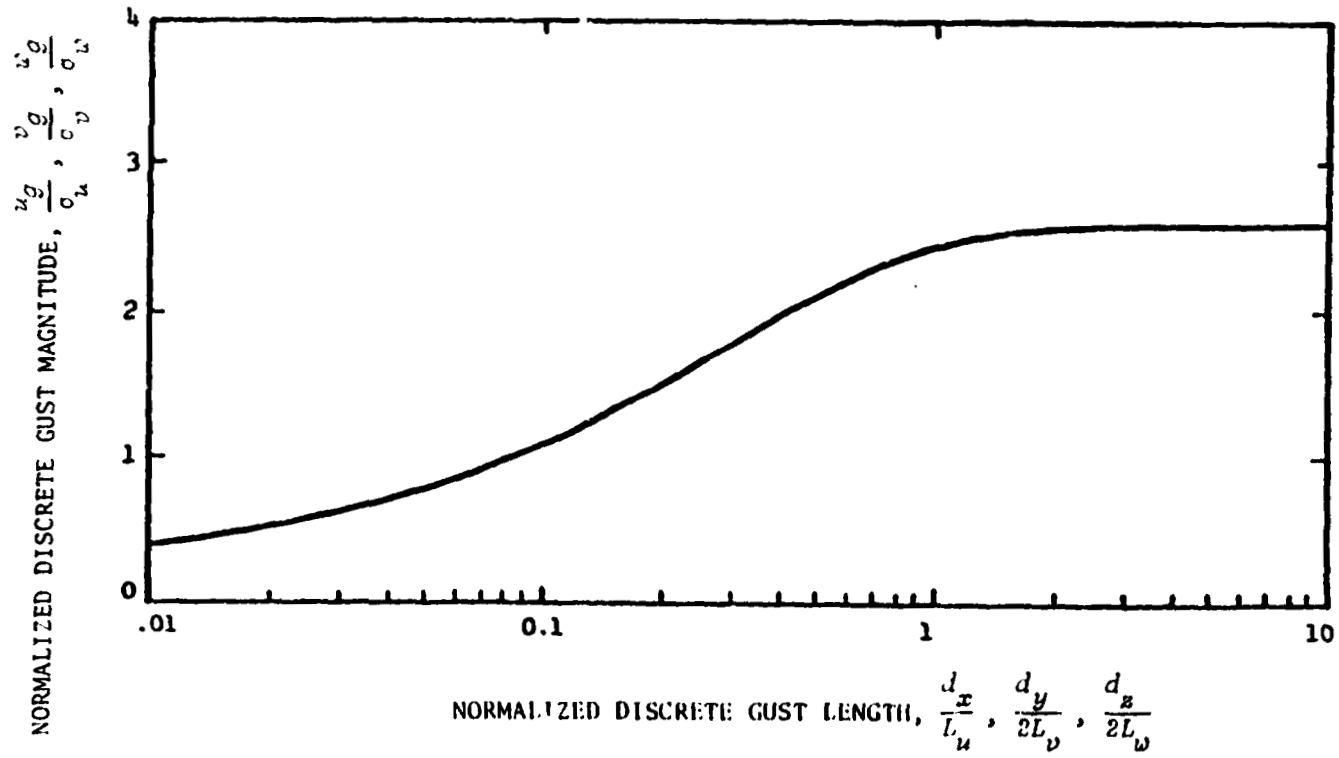
Figure 3.9-1 MAINTENANCE OF DISCRETE GUSTS
