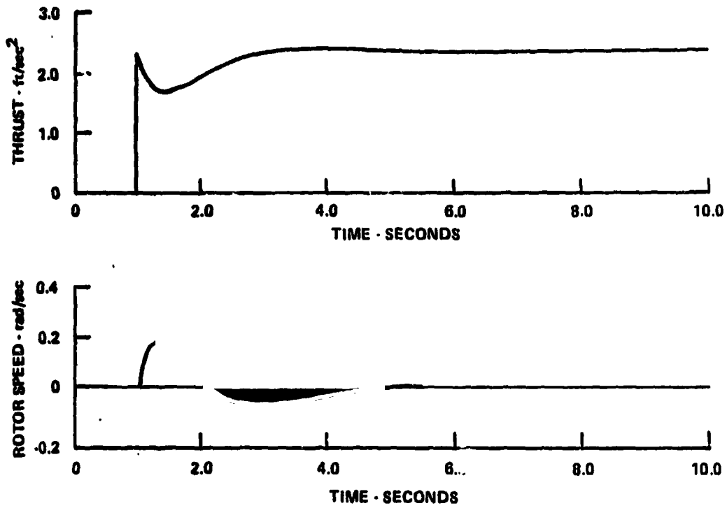
Figure 29 ROTOR THRUST AND SPEED RESPONSE TO COLLECTIVE COMMAND - COLLECTIVE FEEDFORWARD GAIN EQUAL TO "IDEAL" GAIN
