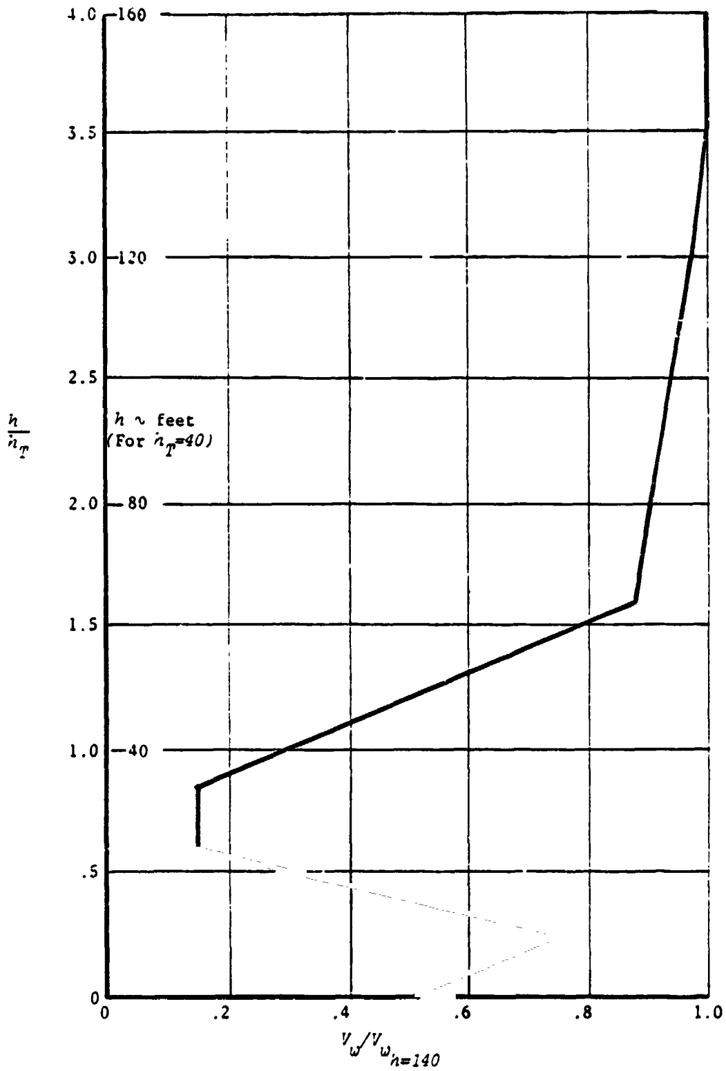
Figure 3.9-2 WIND SPEED BEHIND TREE-LINE
