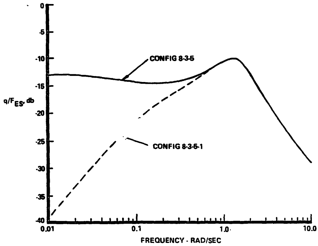
Figure 13. TIFS PITCH RATE PROGRAM-EFFECT OF COMMAND WASHOUT ON RATE RESPONSE
