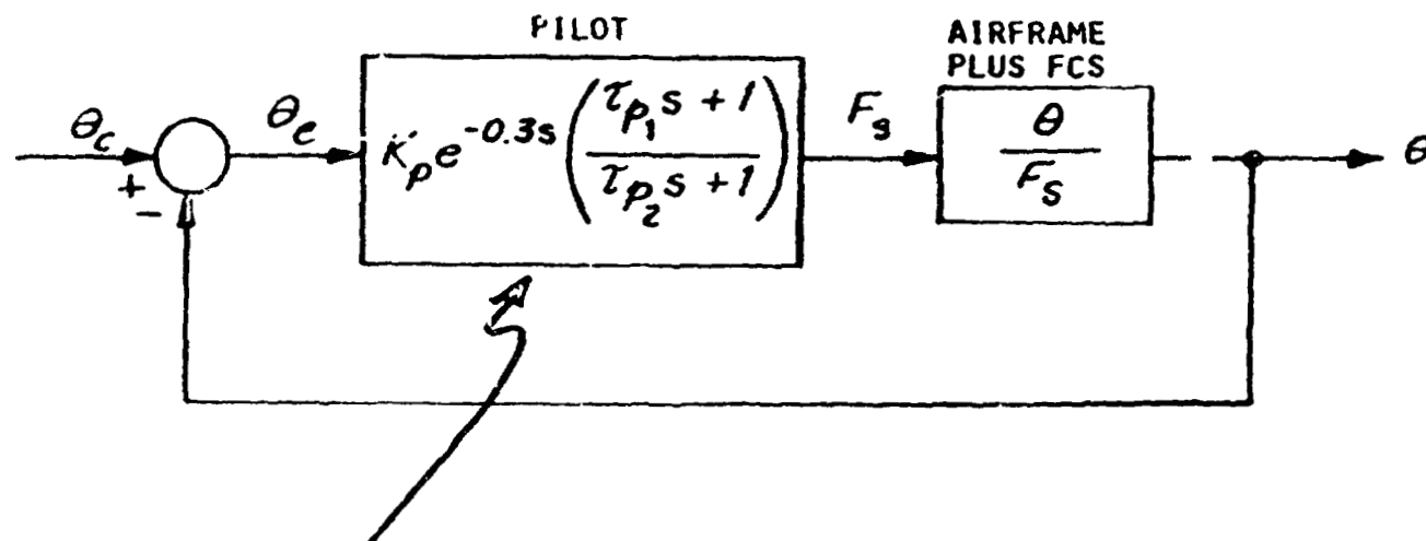
PITCH ATTITUDE COMPENSATOR (LIKE PILOT)
