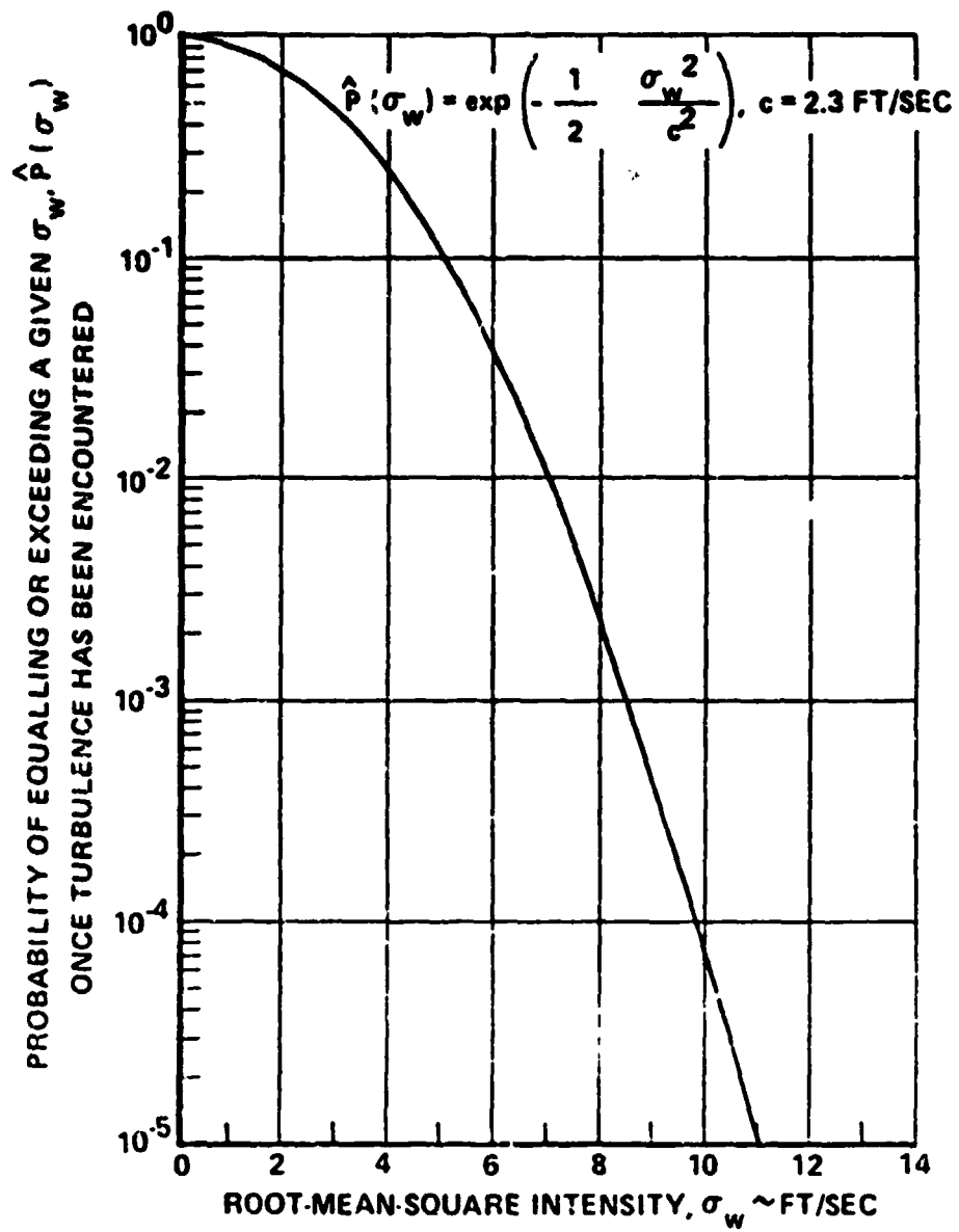
Figure B-5 EXCEEDANCE PROBABILITY
