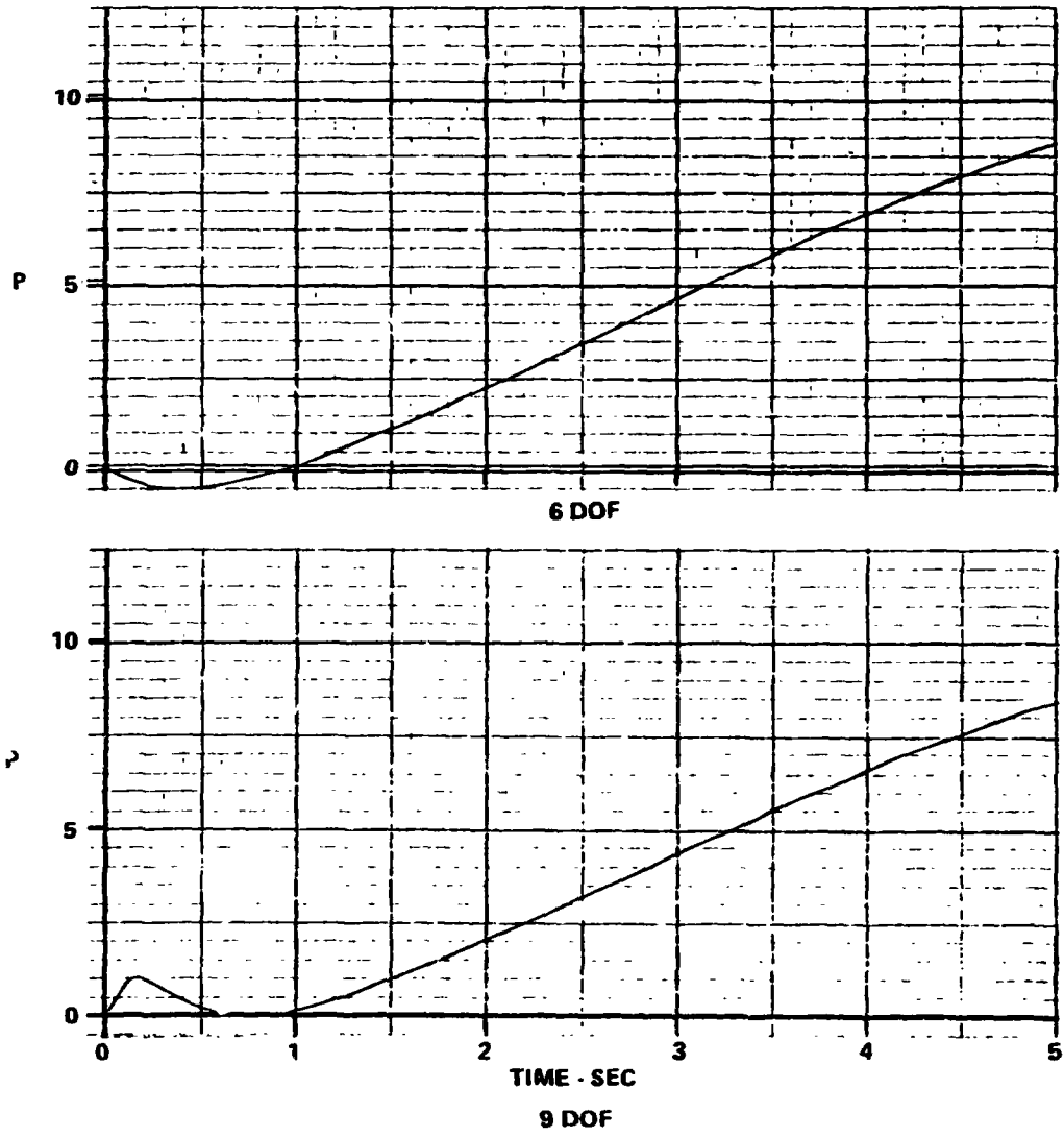
Figure 34 P RESPONSE TO B_{1s} STEP (CH-53, 100 KT)
