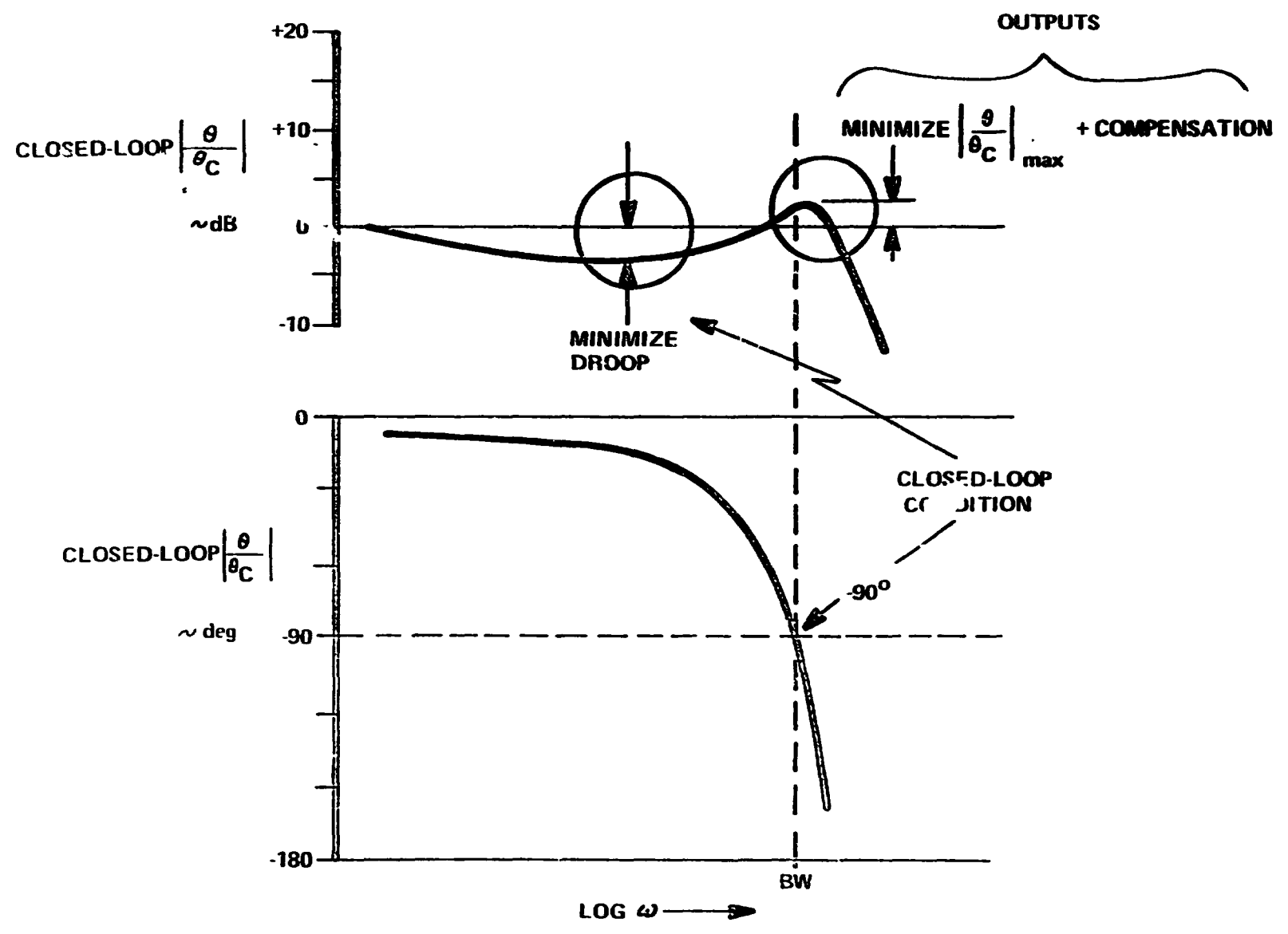
Figure 5. CLOSED LOOP PERFORMANCE PARAMETERS
