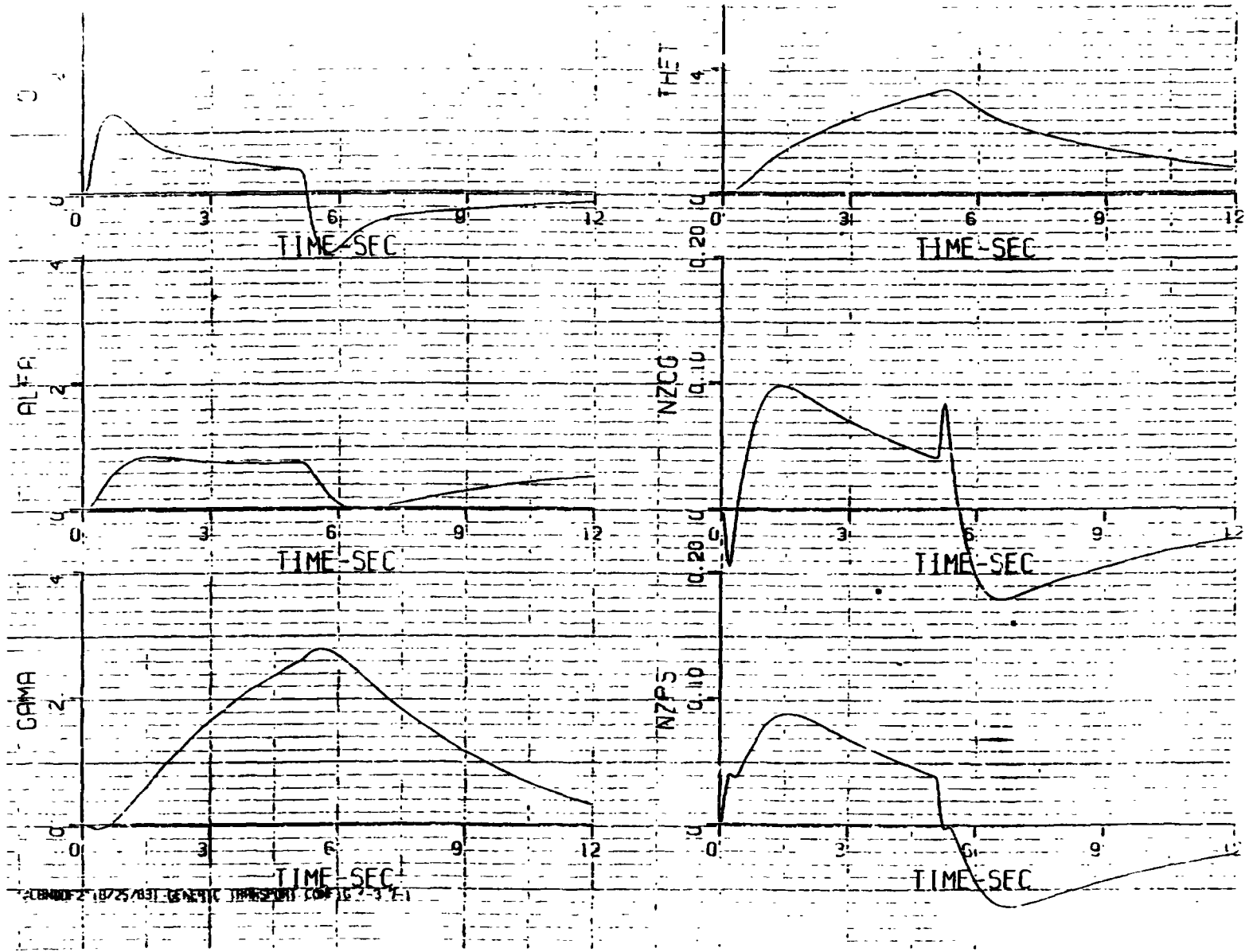
Figure 15. TIFS PITCH RATE PROGRAM - CONFIGURATION 4-3-7-1 CHPR=4
