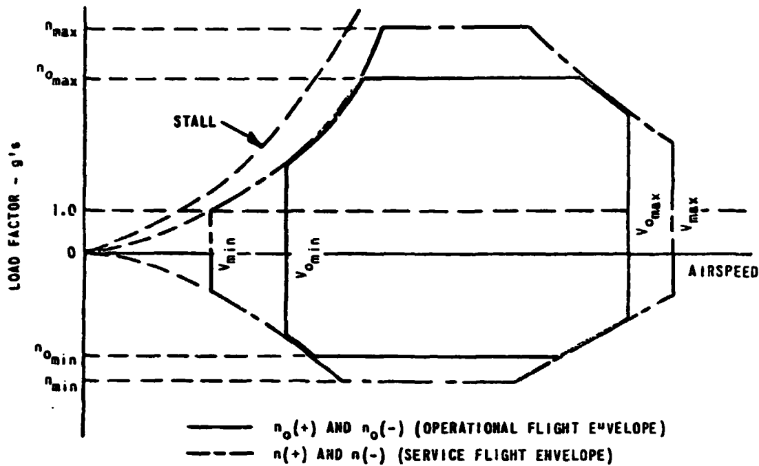
Figure 2.2-1 DEFINITION OF FLIGHT ENVELOPE TERMS
