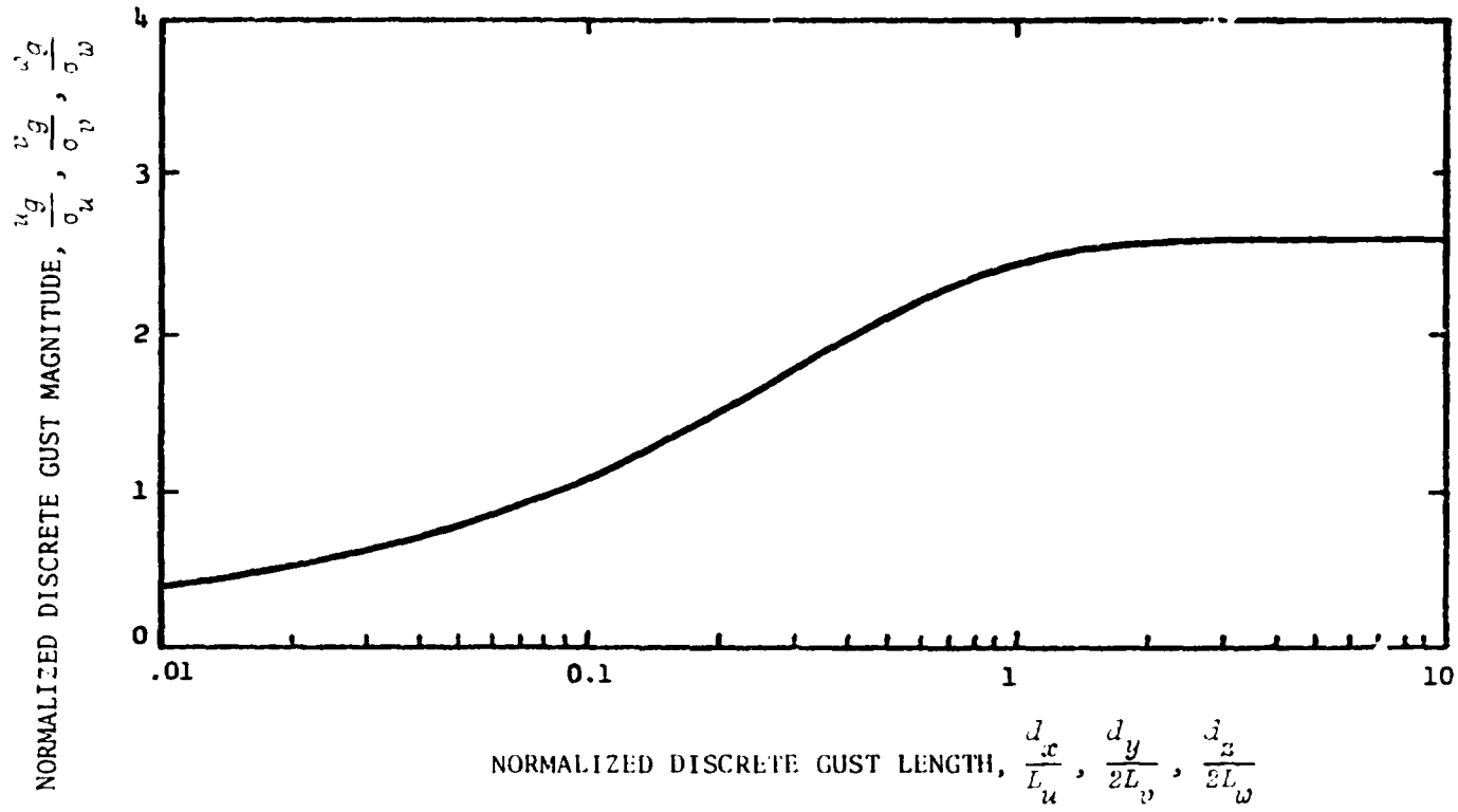
Figure 3.9-1 MAINTENANCE OF DISCRETE GUSTS
