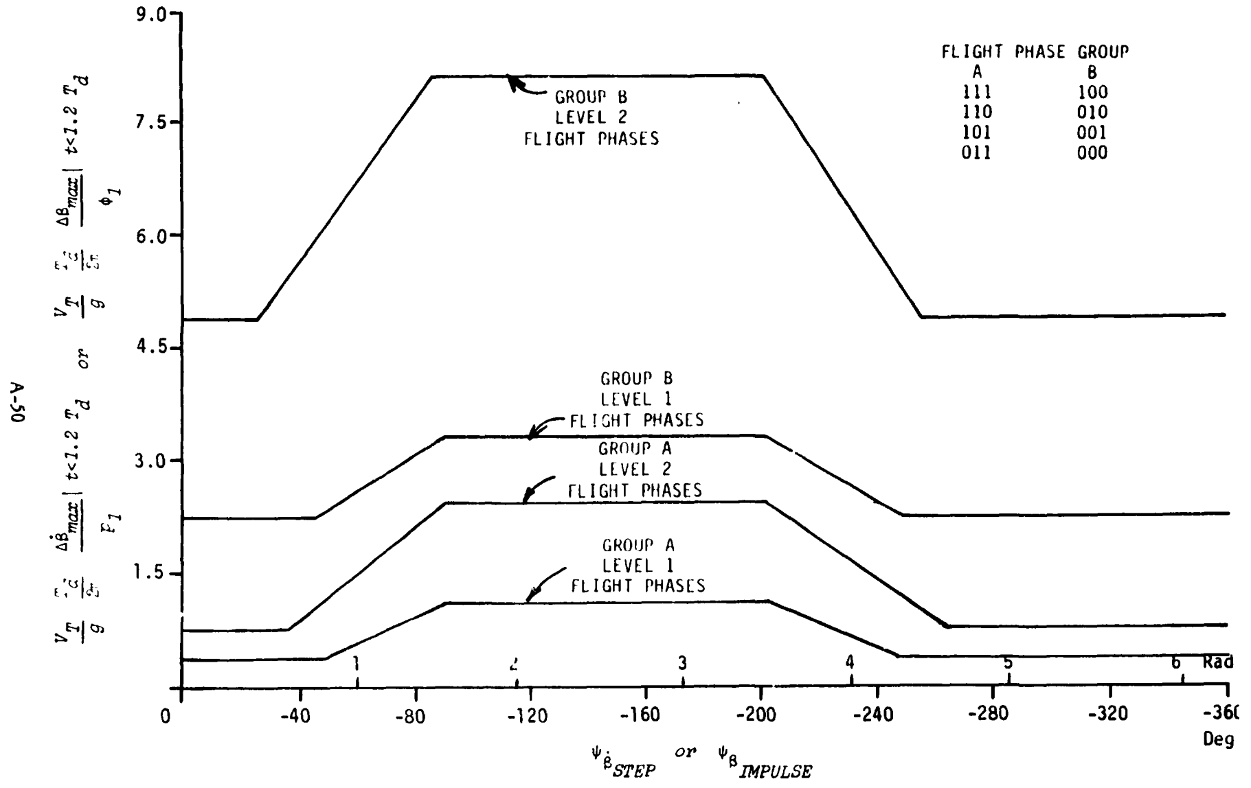
Figure 3.2-2. SIDESLIP EXCURSION LIMITATIONS
