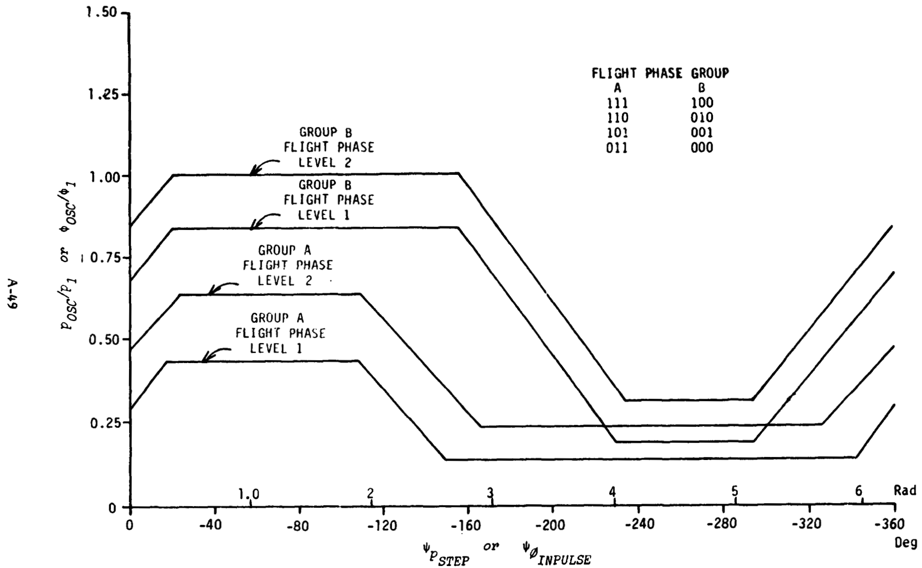
Figure 3.2-1. ROLL RATE AND BANK ANGLE OSCILLATION LIMITATIONS
