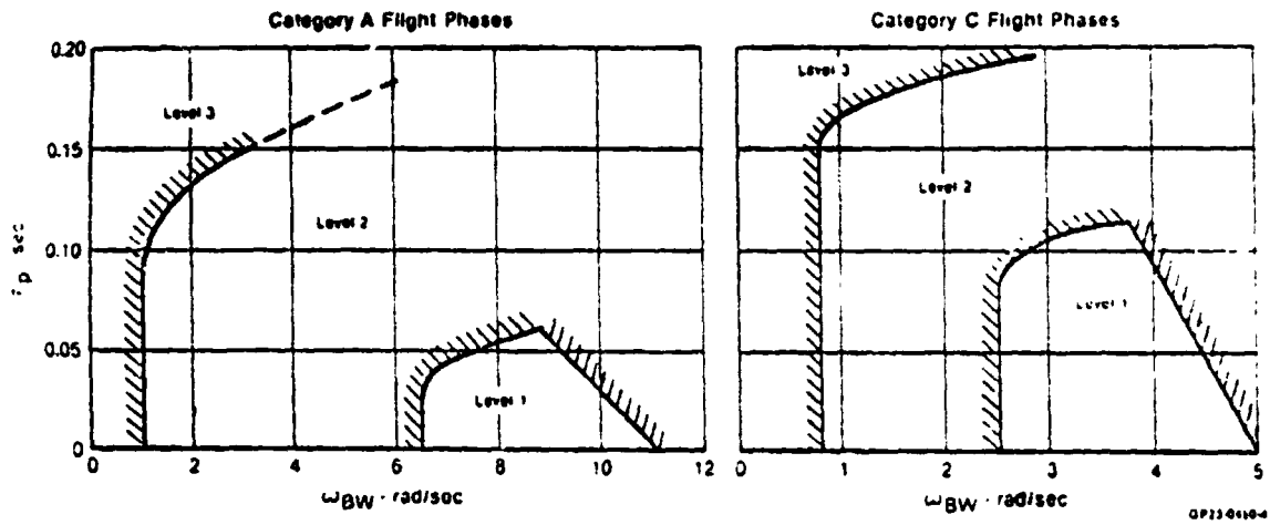
10(b). BANDWIDTH REQUIREMENTS FROM PROPOSED MIL HANDBOOK
