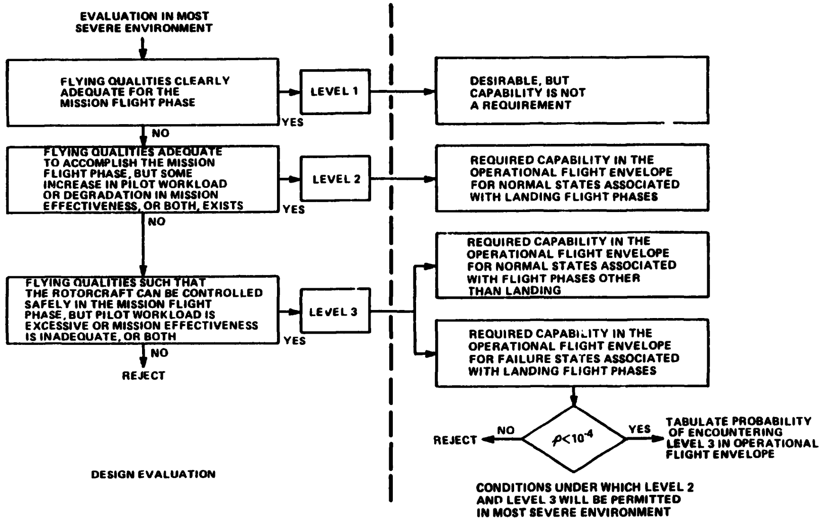
Figure 2 DEFINITION OF CONDITIONS UNDER WHICH LEVEL 2 AND LEVEL 3 FLYING QUALITIES WILL BE PERMITTED IN THE MOST SEVERE ENVIRONMENT
