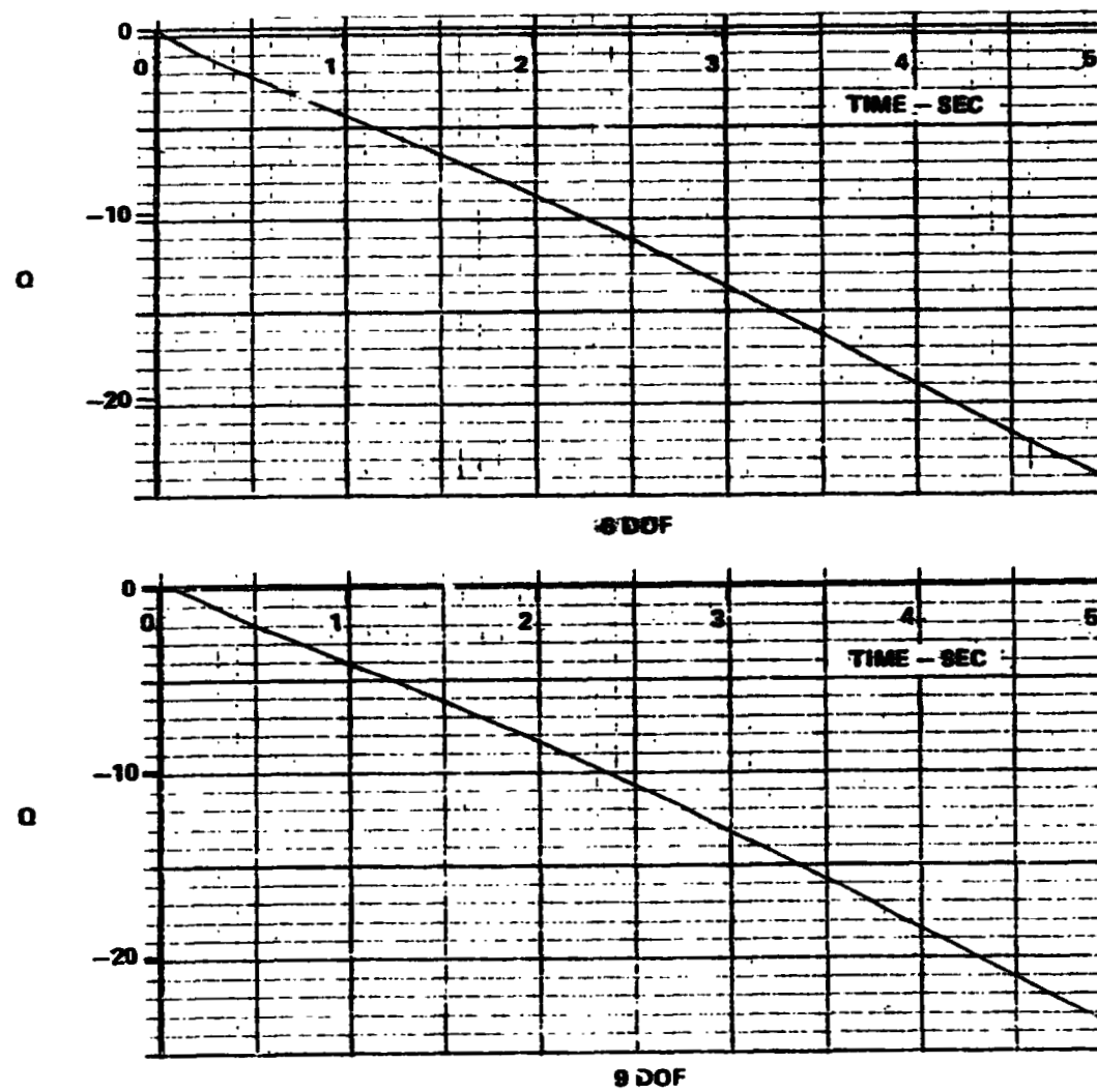
Figure 33 Q RESPONSE TO B_{1S} STEP (CH-53, 100)
