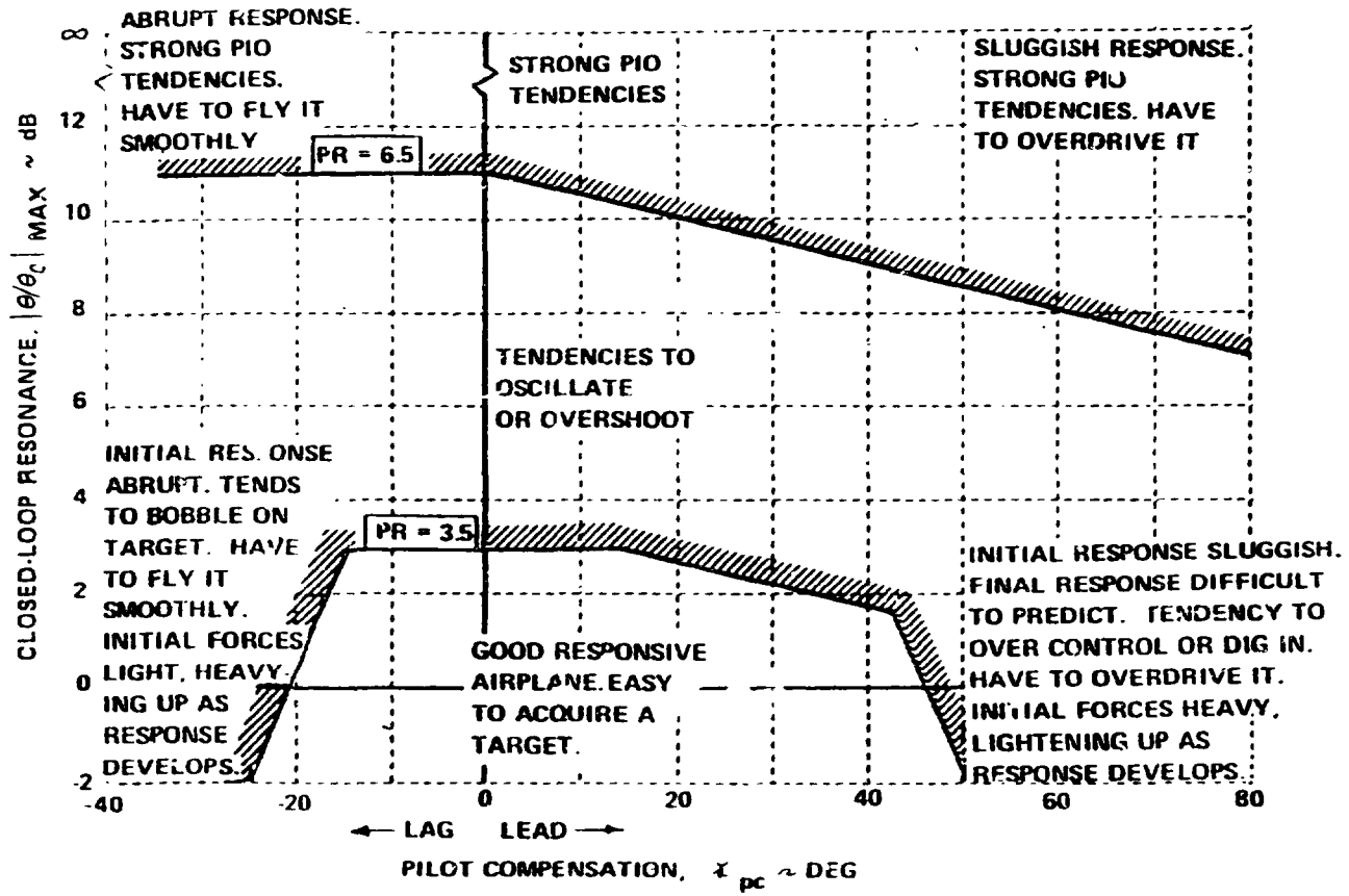
Figure 6. PROPOSED CRITERION FOR FIGHTER MANEUVERING DYNAMICS
