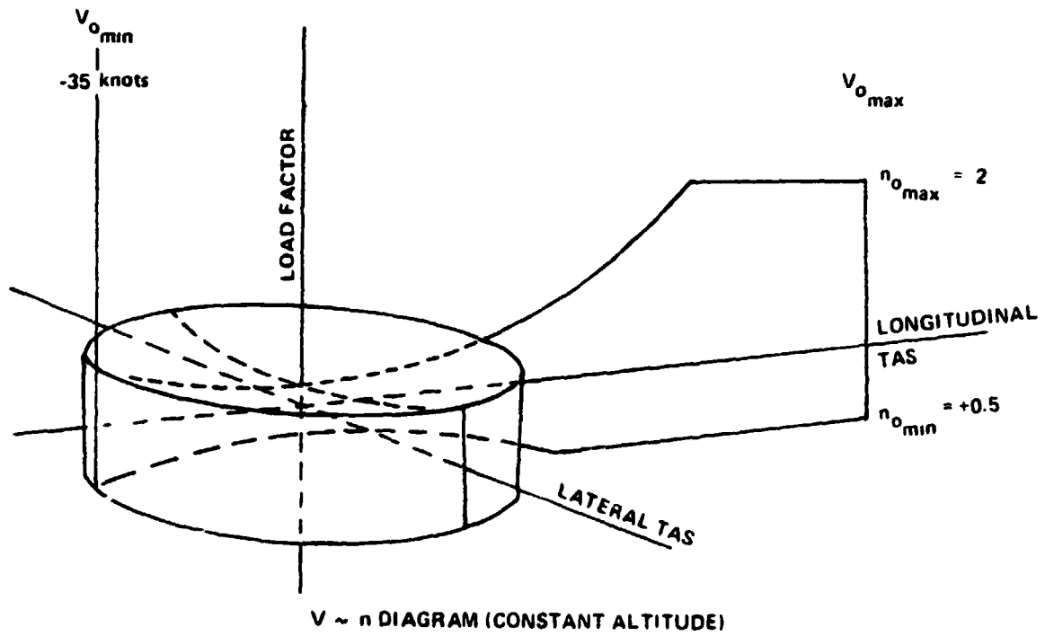
Figure 2.2-2 TYPICAL OPERATIONAL FLIGHT ENVELOPES FOR A FLIGHT PHASE IN THE HOVER AND LOW SPEED FLIGHT REGION AND A FLIGHT PHASE IN THE FORWARD FLIGHT REGION
