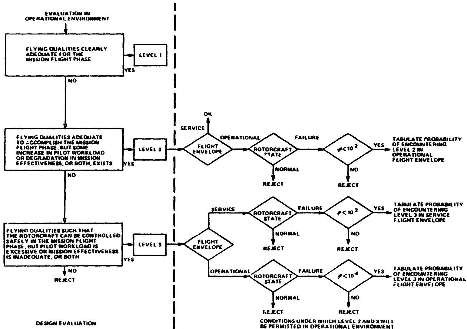
Figure 2.4-4 DEFINITION OF CONDITION UNDER WHICH LEVEL 2 AND 3 FLYING QUALITIES WILL BE PERMITTED IN THE OPERATIONAL ENVIRONMENT
