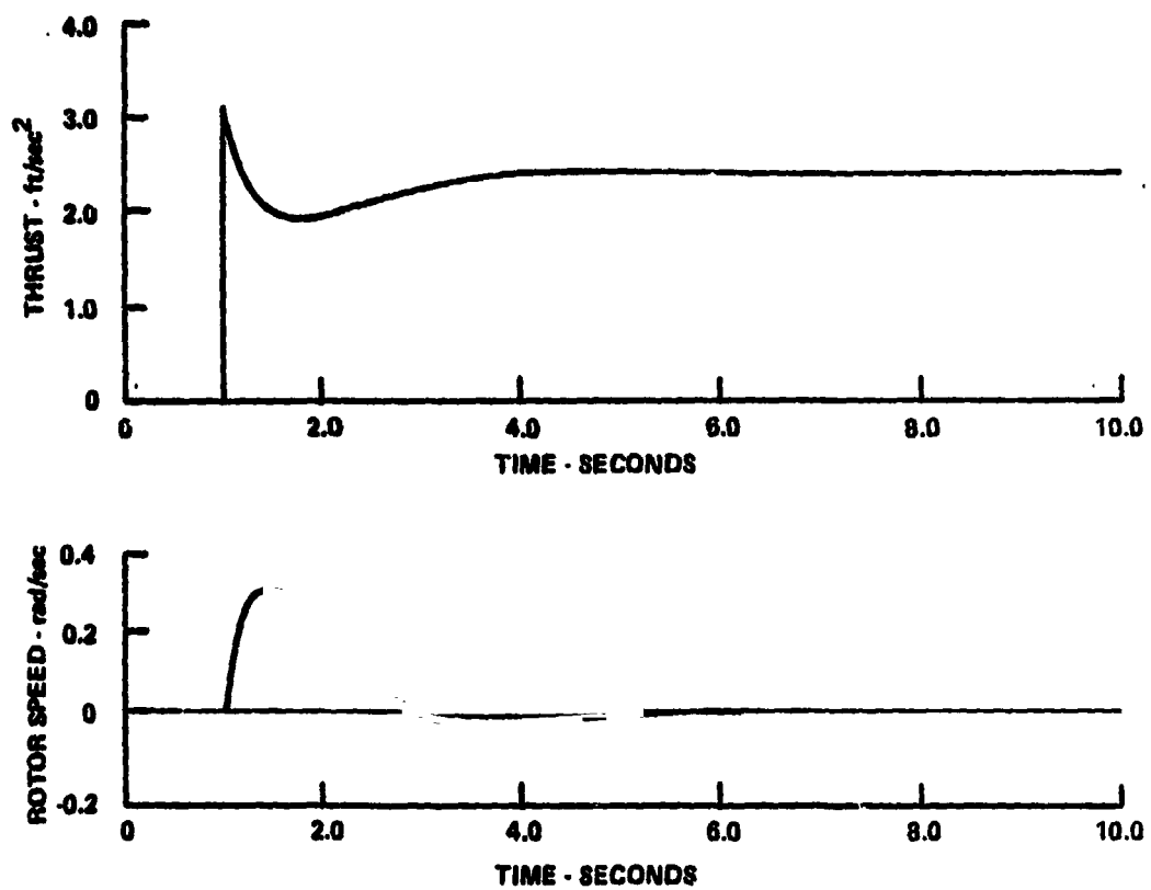
Figure 28 ROTOR THRUST AND SPEED RESPONSE TO COLLECTIVE PITCH COMMAND COLLECTIVE FEEDFORWARD GAIN EQUAL TO 133% OF "IDEAL" GAIN
