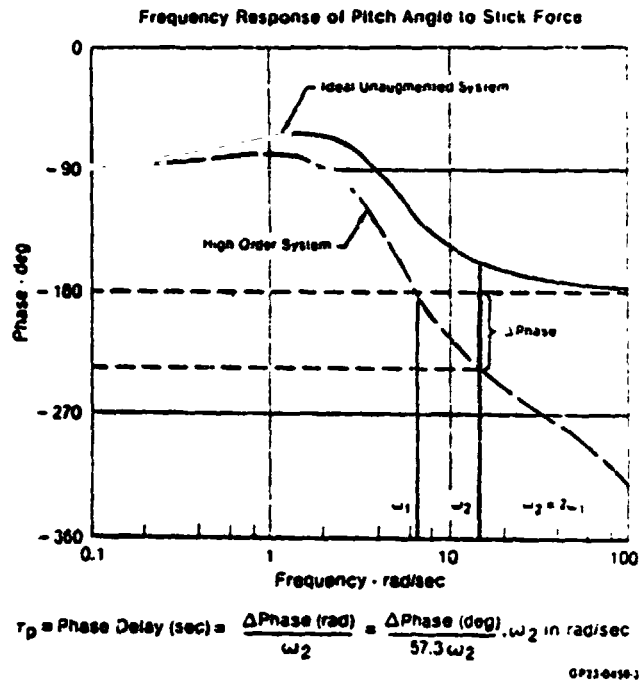
10(a). DEFINITION OF PHASE DELAY, \tau_p
