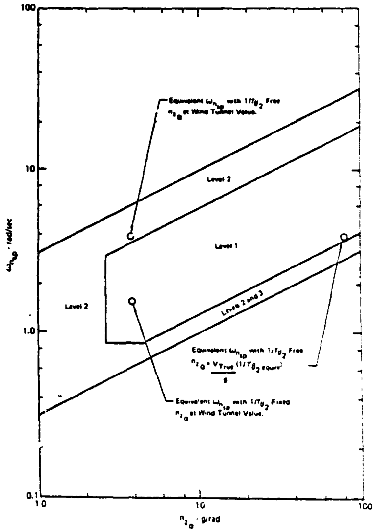
Figure 8. MAPPING OF EQUIVALENT SYSTEMS ON \omega_{h10} VS n_{z0} PLANE
