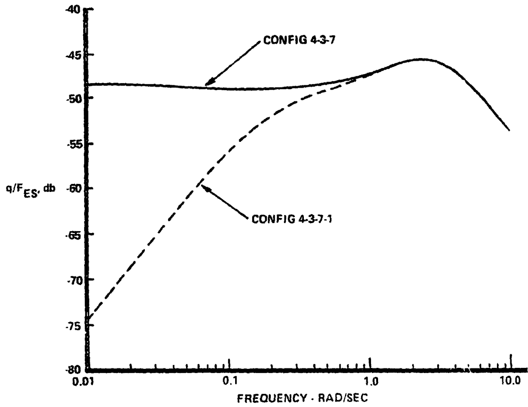
Figure 12. TIFS PITCH RATE PROGRAM-EFFECT OF COMMAND WASHOUT ON RATE RESPONSE
