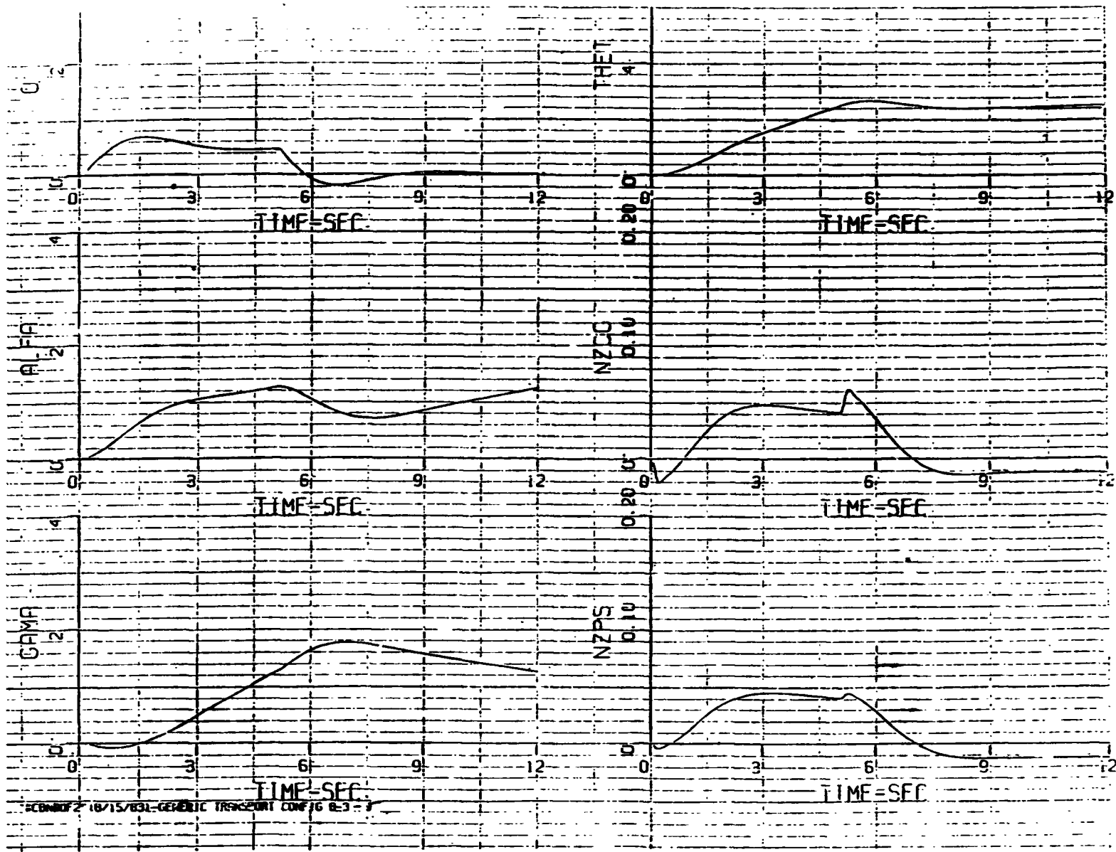
Figure 16. TIFS PITCH RATE PROGRAM - CONFIGURATION 8-3-5 CHPR=7, 8
