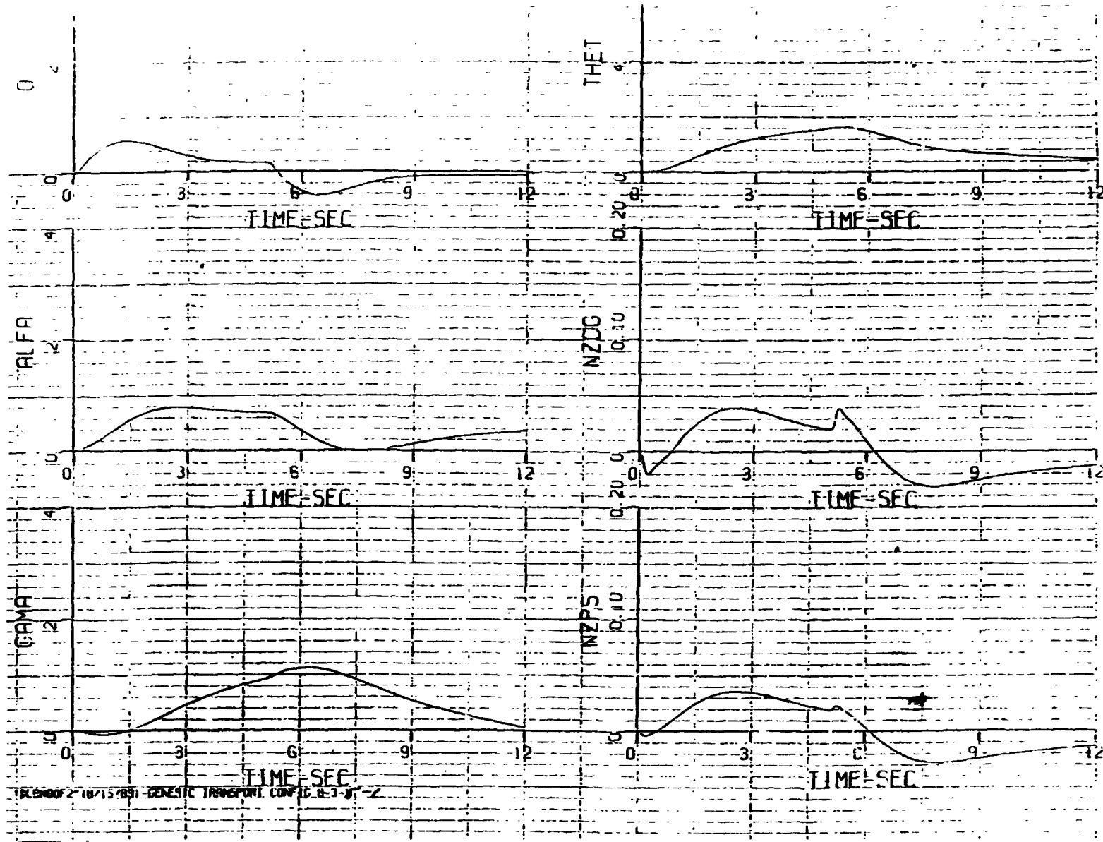
Figure 17. TIFS PITCH RATE PROGRAM - CONFIGURATION 8-3-5-1 CHPR=3, 3
