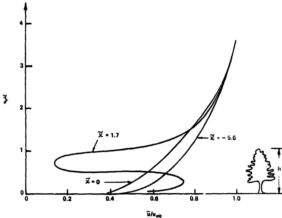
Figure B-6 NORMALIZED VELOCITY PROFILES NEAR THE EDGE OF A FOREST SHOWING THE JETTING ACTION IN THE REGION OF THE TRUNKS TREE SPACING \approx h
