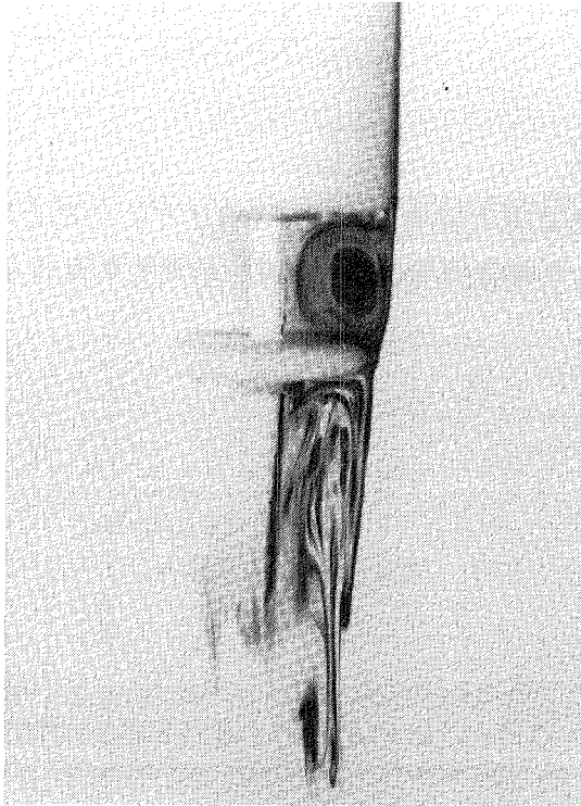
Injected dye technique
