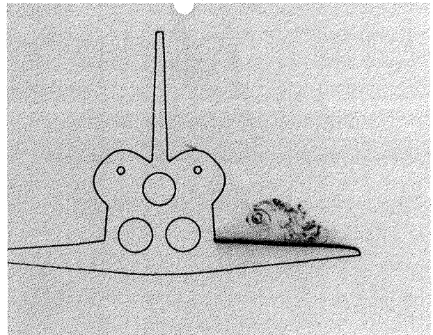
LEV cross-plane result with model outline superimposed
