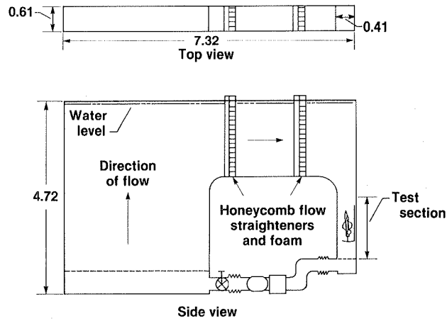
Water tunnel schematic (dimensions in meters)
