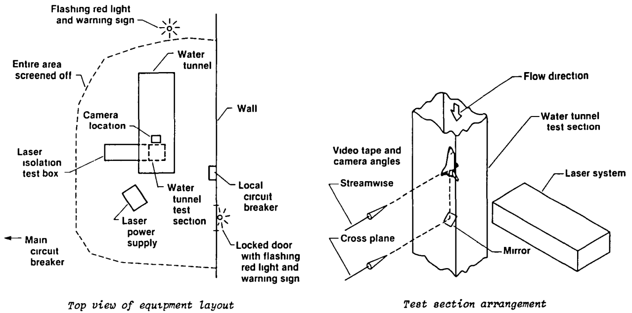
Fig. 2 Schematic of water tunnel test setup.
