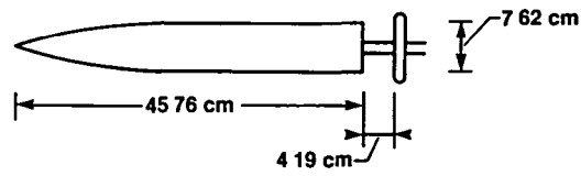
Trailing disk model
