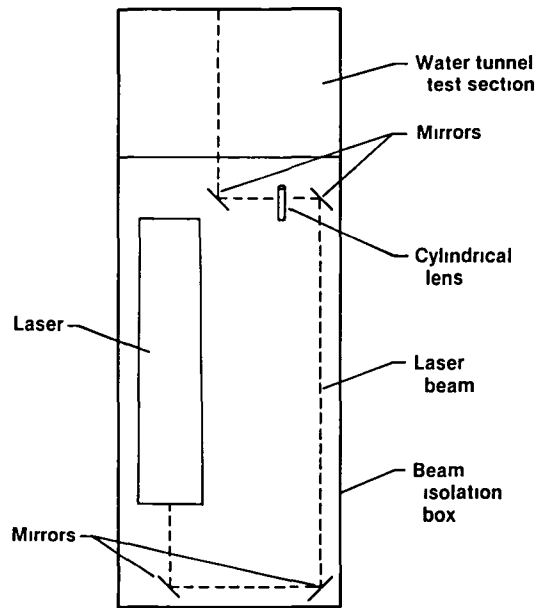
Fig. 3 Schematic of laser system.
