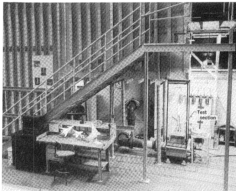
Photograph of water tunnel showing conventional test setup
