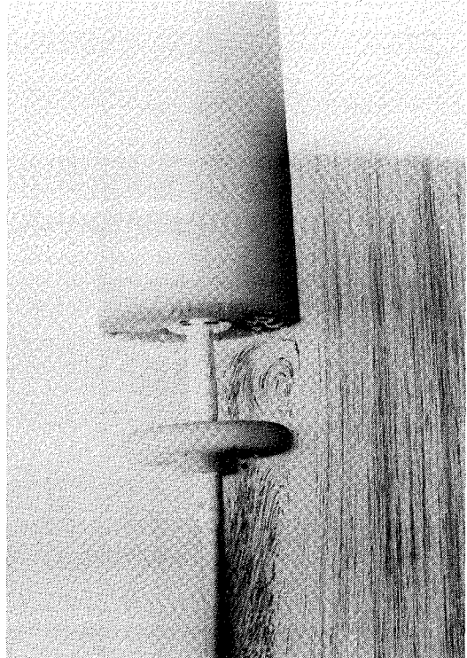
Embedded particulates technique
