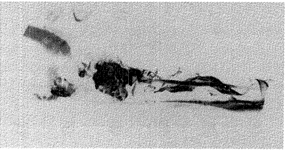
Fig. 5 Variation of flourescein sodium concentration, 750 mW laser power.
