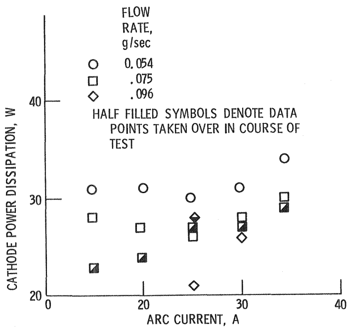
Figure 8. - Cathode power loss versus current ; test number 84.
