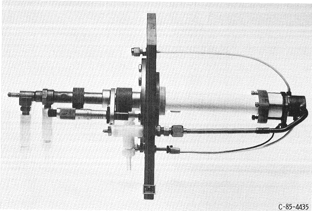
(b) Photograph of thruster simulator.
