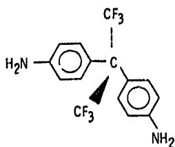
p, p'-6FDAM 2,2-bis(4-Aminophenyl)Hexafluoropropane
