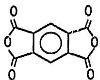
PMDA Pyromellitic Dianhydride
