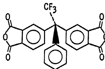
3FDA 4,4'-(1-Phenyl-2,2,2-Trifluoro- ethylidene) Bis(Phthalic Anhydride)
