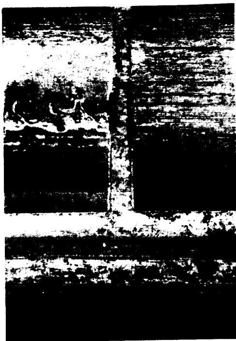
Figure 8.—Typical fatigue spall for VIM-VAR EX-53 gears.
