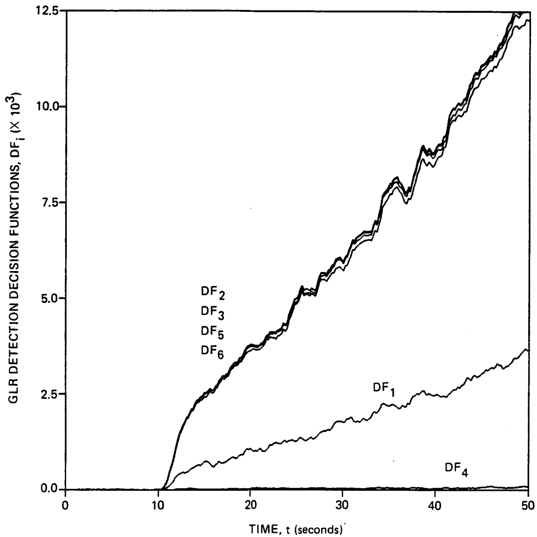
Figure 5.10. GLR detection decision functions for the linear simulation with a 0.01745 \text{ rad} ( 1^\circ ) bias failure of the right aileron at time t = 10 \text{ s} . A 100 sample (2 s) data window was used.
