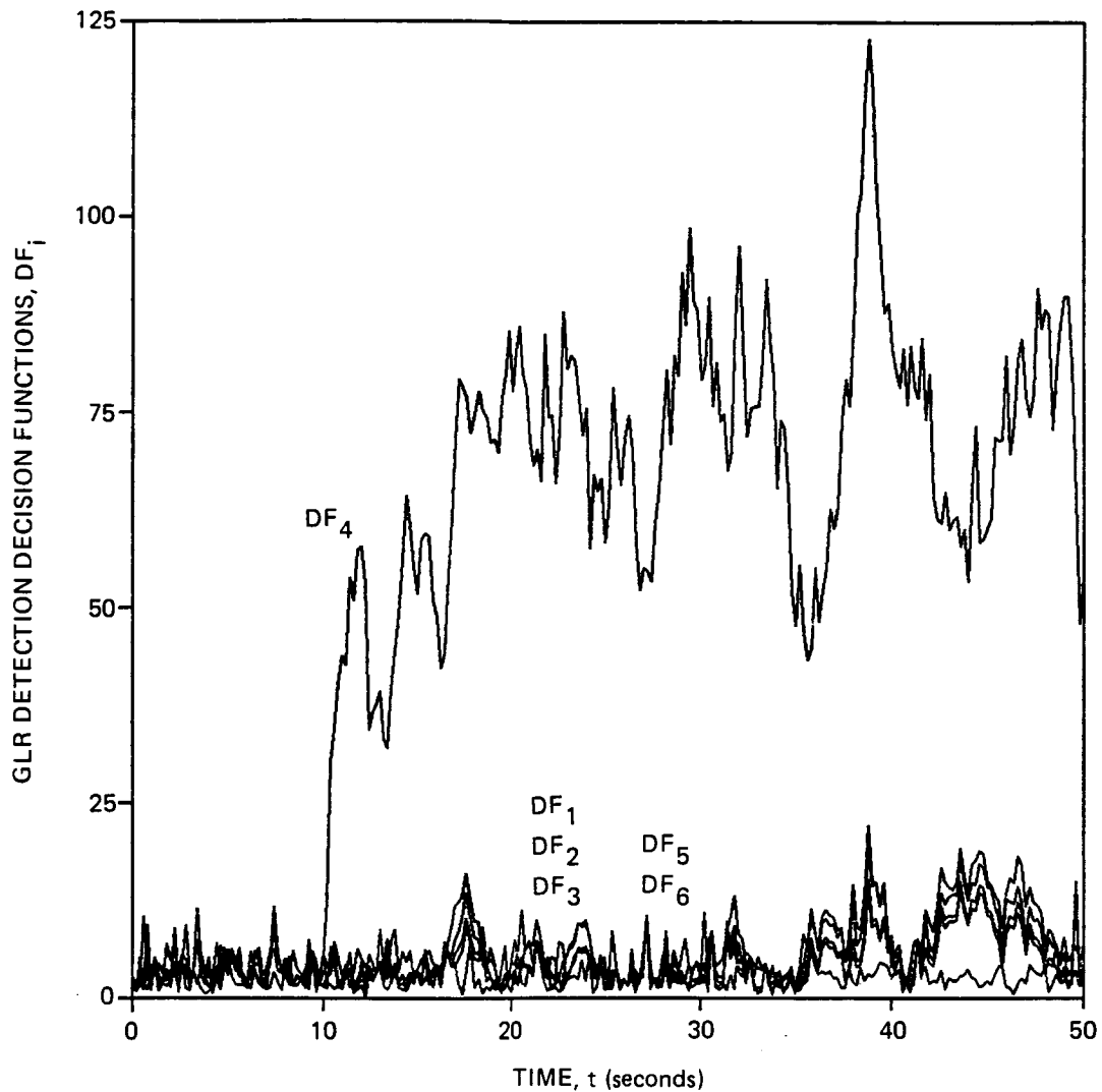
Figure 5.7. GLR detection decision functions for the linear simulation with a 0.0349 rad ( 2^\circ ) bias failure of the rudder at time = 10 s. A sample (2 s) data window was used.
