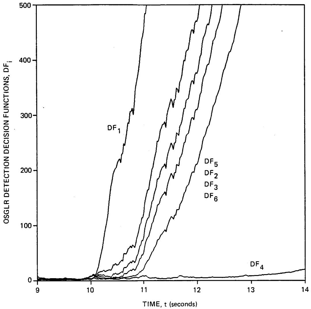
Figure 5.4. OSGLR detection decision functions for the linear simulation with a -0.01745 rad ( -1^\circ ) bias failure of the elevator at time t = 10 s (Cont.)
