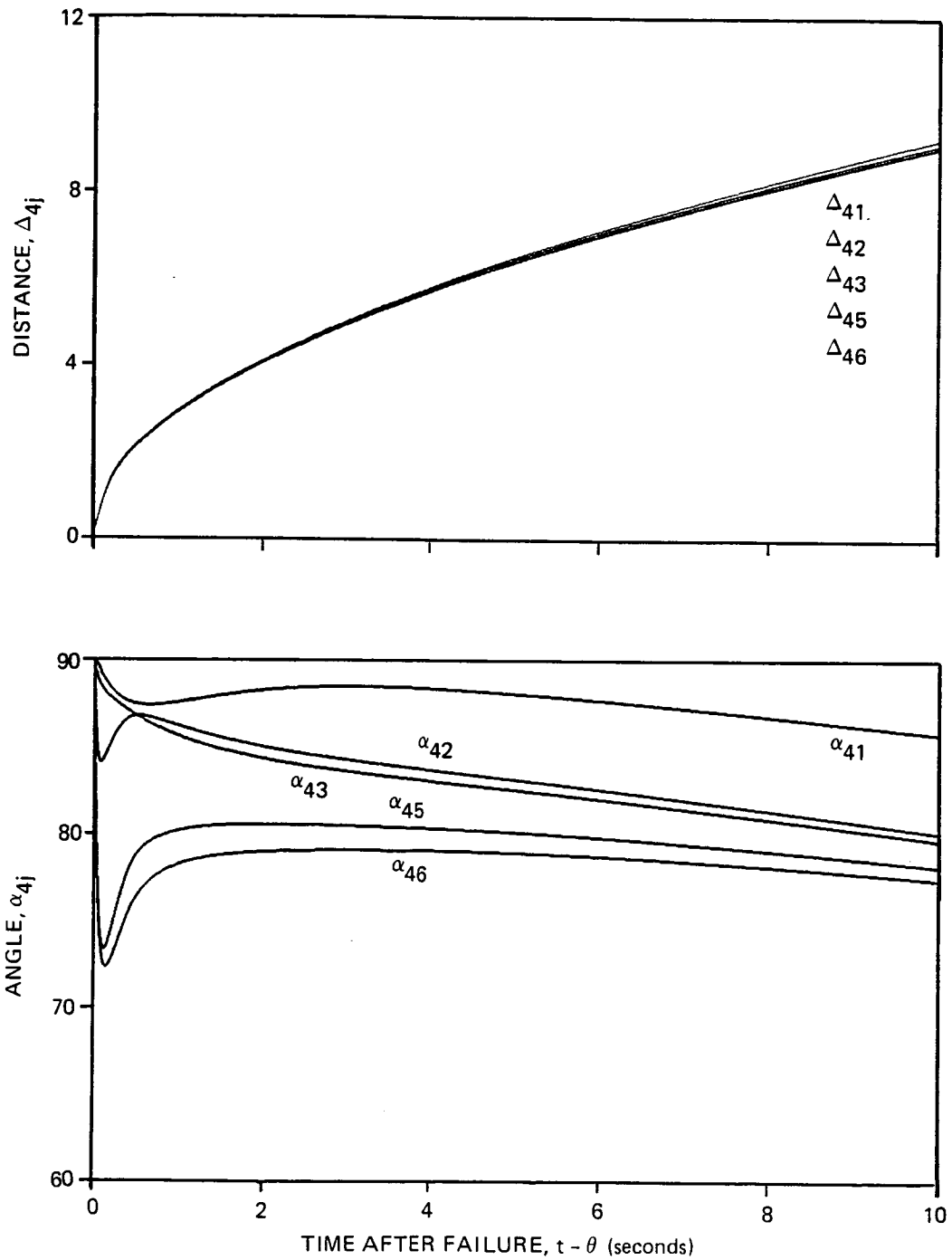
Figure 6.3. Distinguishability measures for a 0.01745 \text{ rad } (1^\circ) bias failure of the rudder
