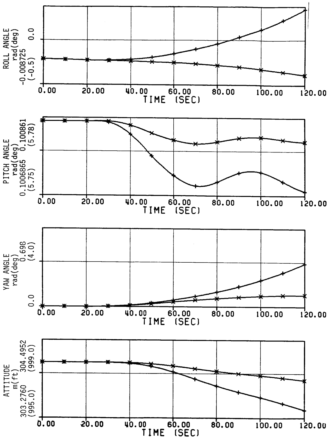
Figure A.2. Linear and nonlinear responses for a perturbation in rudder (Cont.)
