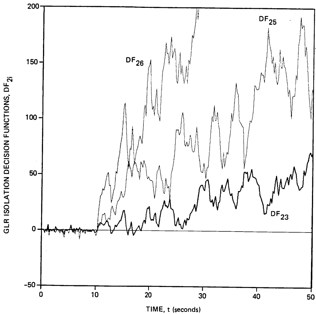
Figure 5.11. GLR isolation decision functions for the linear simulation with a 0.01745 rad ( 1^\circ ) bias failure of the right aileron at time t = 10 s.
