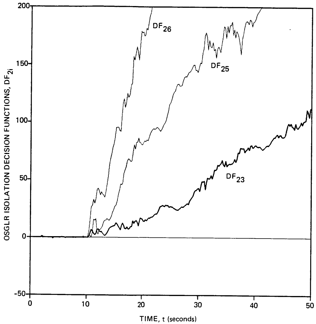
Figure 5.9. OSGLR isolation decision functions for the linear simulation with a 0.01745 rad ( 1^\circ ) bias failure of the right aileron at time t = 10 s
