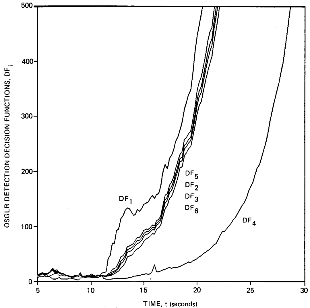
Figure 5.19. OSGLR detection decision functions for the nonlinear simulation with a stuck elevator at time t = 10 s. Note the expanded time scale in the vicinity of t = 10 s (Cont.)
