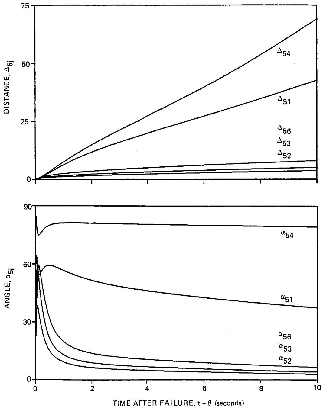
Figure 6.5. Distinguishability measures for a 0.01745 rad ( 1^\circ ) bias failure of the right flap
