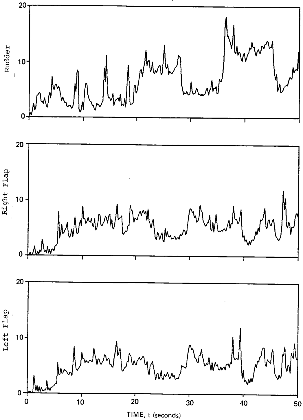
Figure 5.2. OSGLR detection decision functions for the linear simulation with no failures (Cont.)
