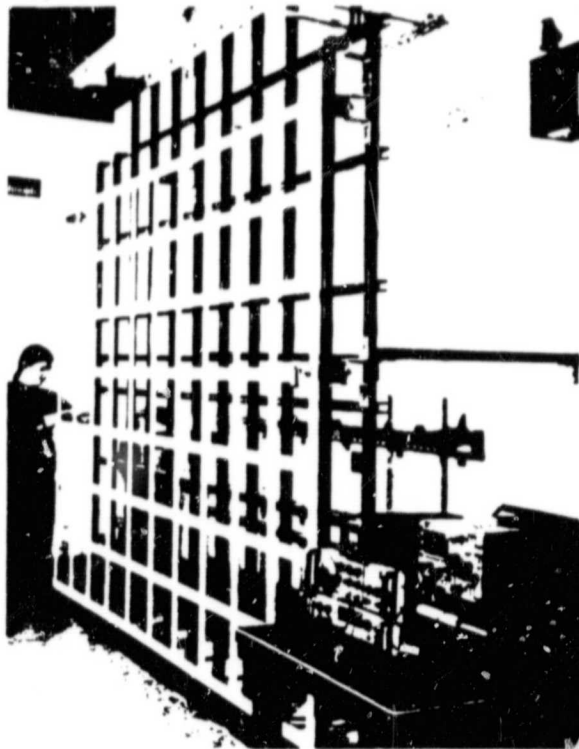
Fig. 6 A photograph of the flexible grid apparatus.
