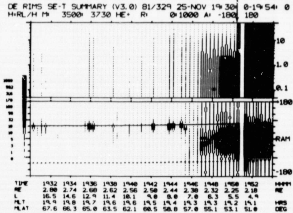
Figure 22. Retarding potential and spin spectrograms for H + and He + showing the failure of the radial head RPA sweep.
