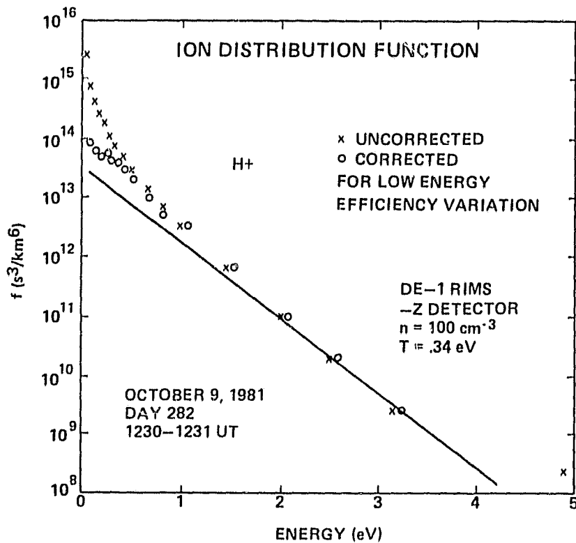
Figure 16. Comparison of derived phase space densities and Maxwellian fits.
