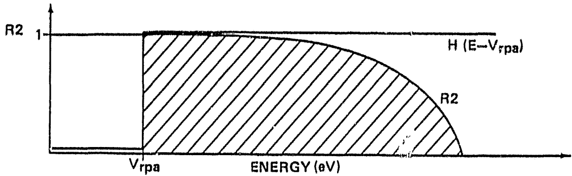
Figure 1. Energy response function with fixed R3, sliding V_{rpa} .
