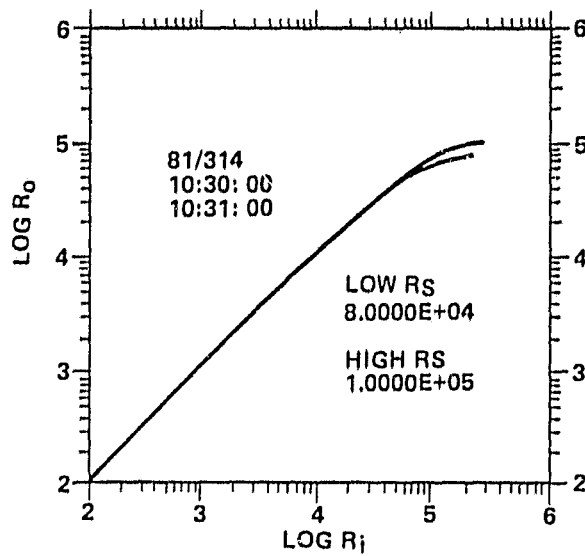
Figure 9. Calibration summary for day 314 of 1981. (a) spin curves, H + , O + , electrometer. (b) Spin curves He + . (c) Saturation curves.
