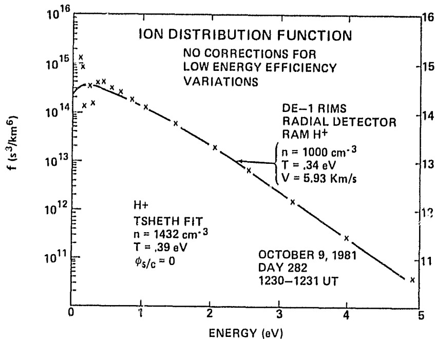
Figure 14. Comparison of derived phase space density and a Maxwellian fit.
