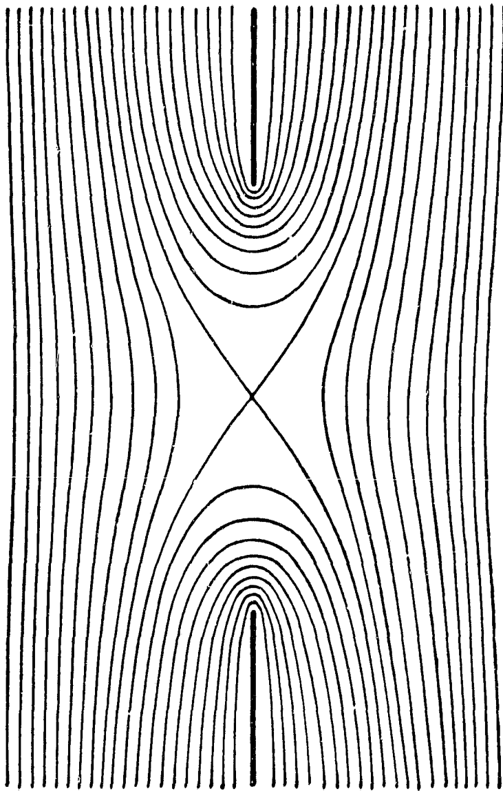
Figure 17. Aperture midway between plates at the same potential.
