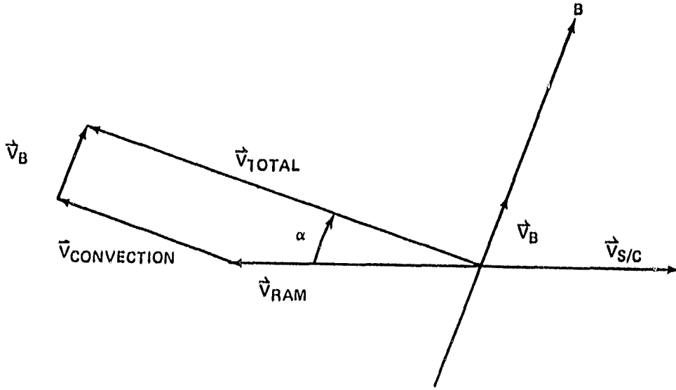
Figure 8. Geometry for derivation of bulk flow from integral flux spin curves.
