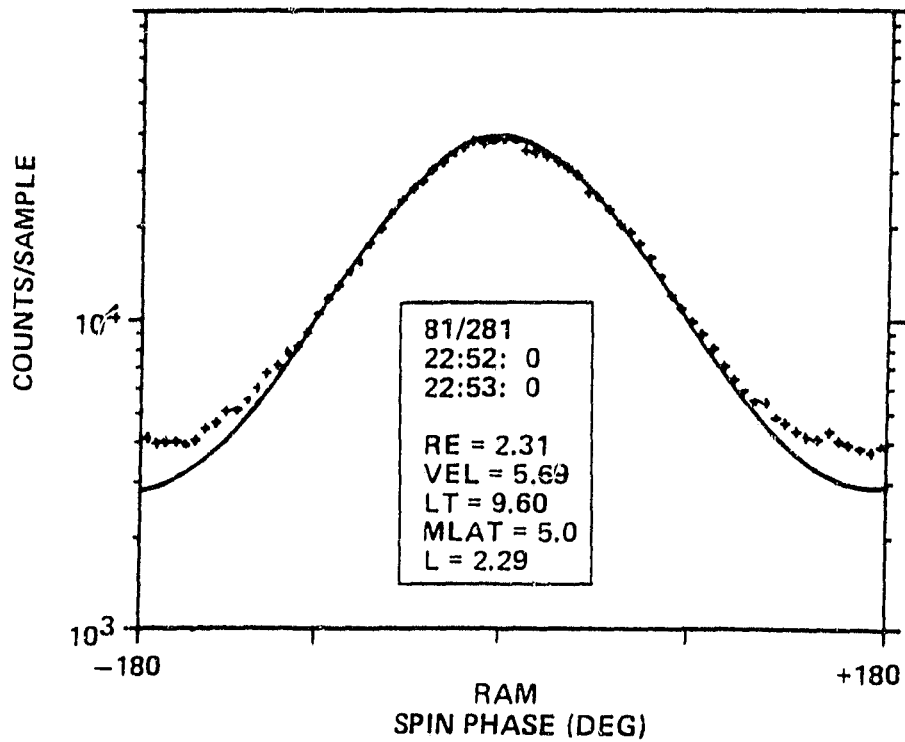
Figure 7. Sample RPA and spin curves showing Maxwellian fits to the data.
