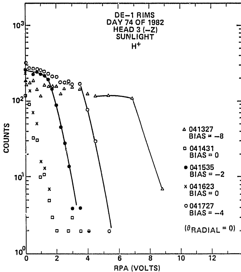
Figure 24. Examples of RPA curves showing abnormal dependence on aperture plane bias.
