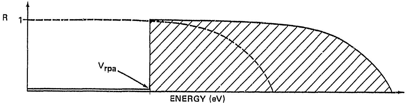
Figure 2. Energy response with sliding R3, V_{rpa} .
