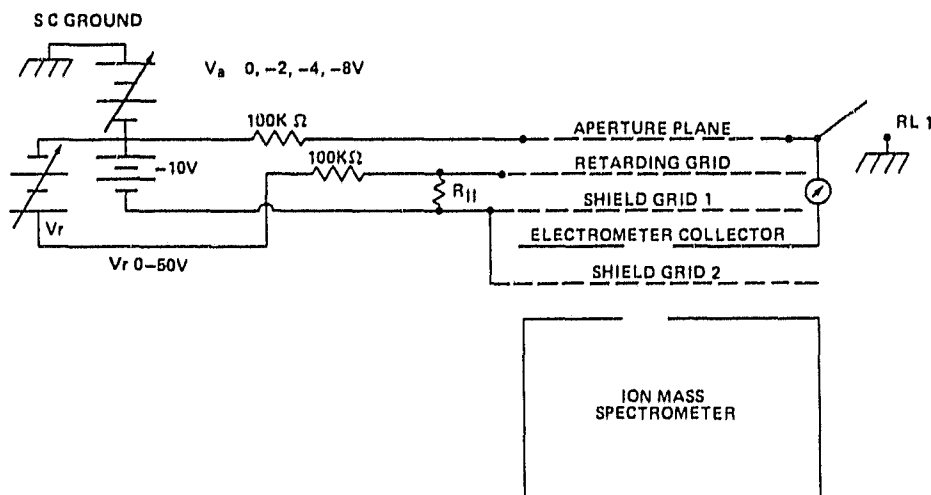
Figure 20. Schematic diagram of RPA and aperture biasing of the RIMS sensor heads.
