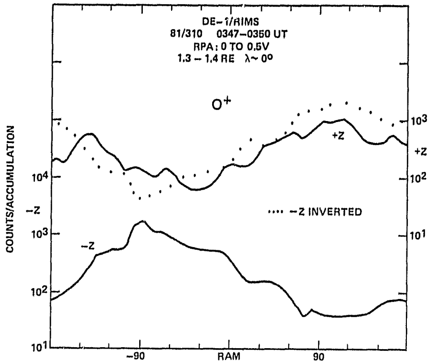
Figure 18. Example of spin modulation of axial head count rates.
