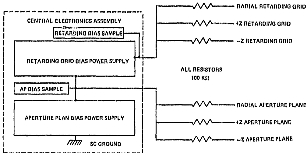
Figure 21. Functional diagram of RIMS aperture and RPA biasing electronics.
