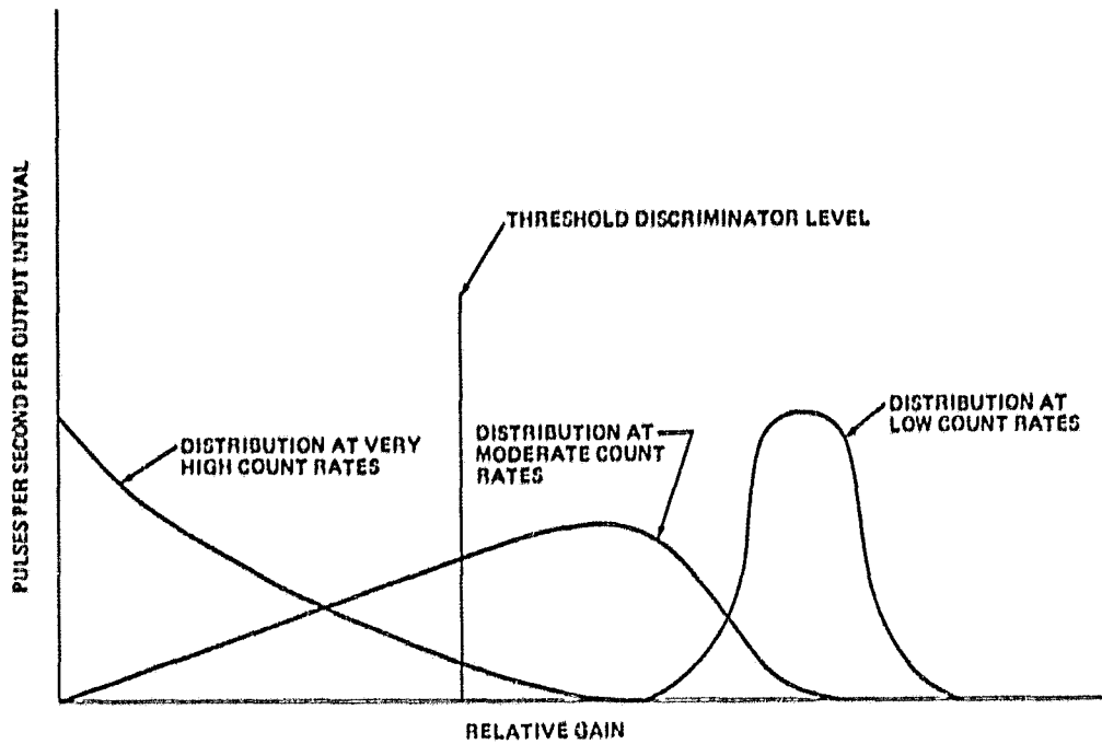
Figure 12. Schematic dependence of channel flow pulse height distribution on total count rate.
