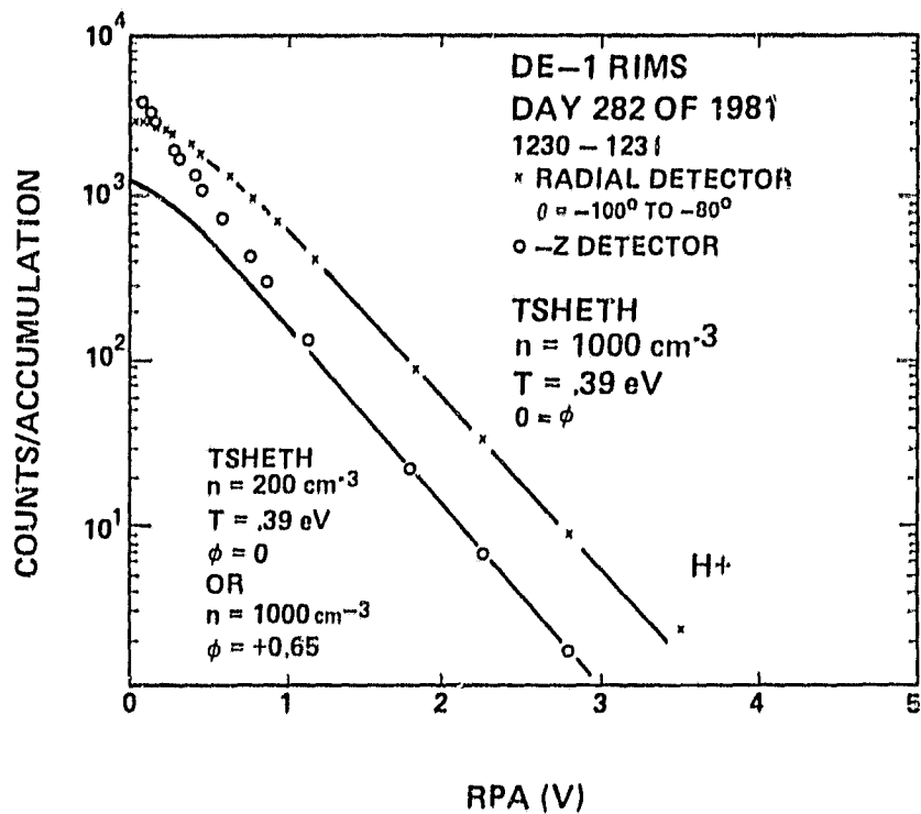
Figure 15. Comparison of raw data and Maxwellian fits.
