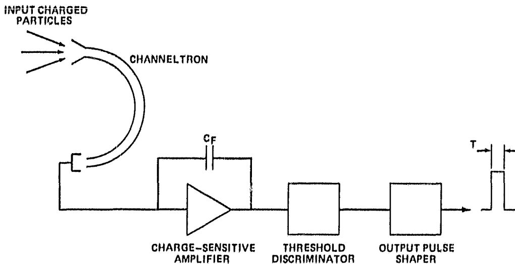
Figure 11. Functional representation of the RIMS detector pulse shaping electronics.
