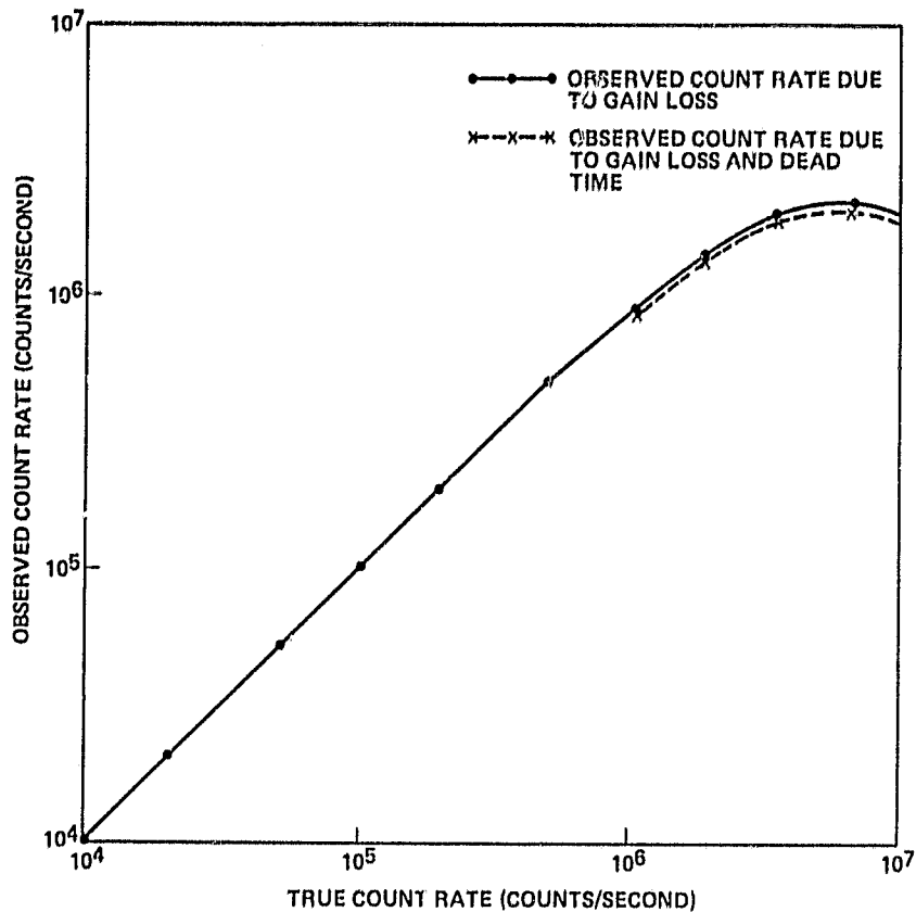
Figure 13. Saturation model for R_s = 7 \times 10^6 Hz, T = 50 ns.
