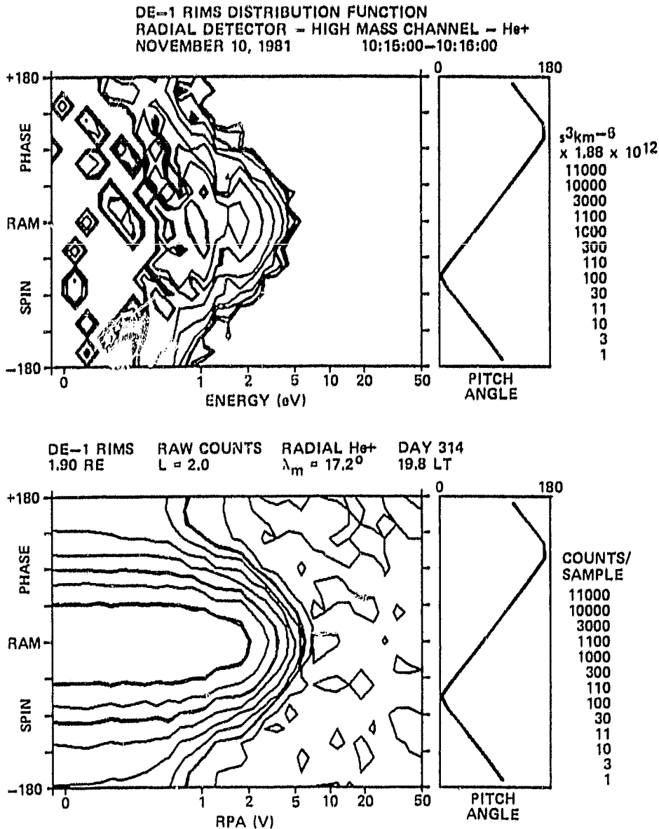
Figure 4. Direct reduction of \text{He}^+ count rates (lower panel) to phase space densities (upper panel) by the differencing technique.
