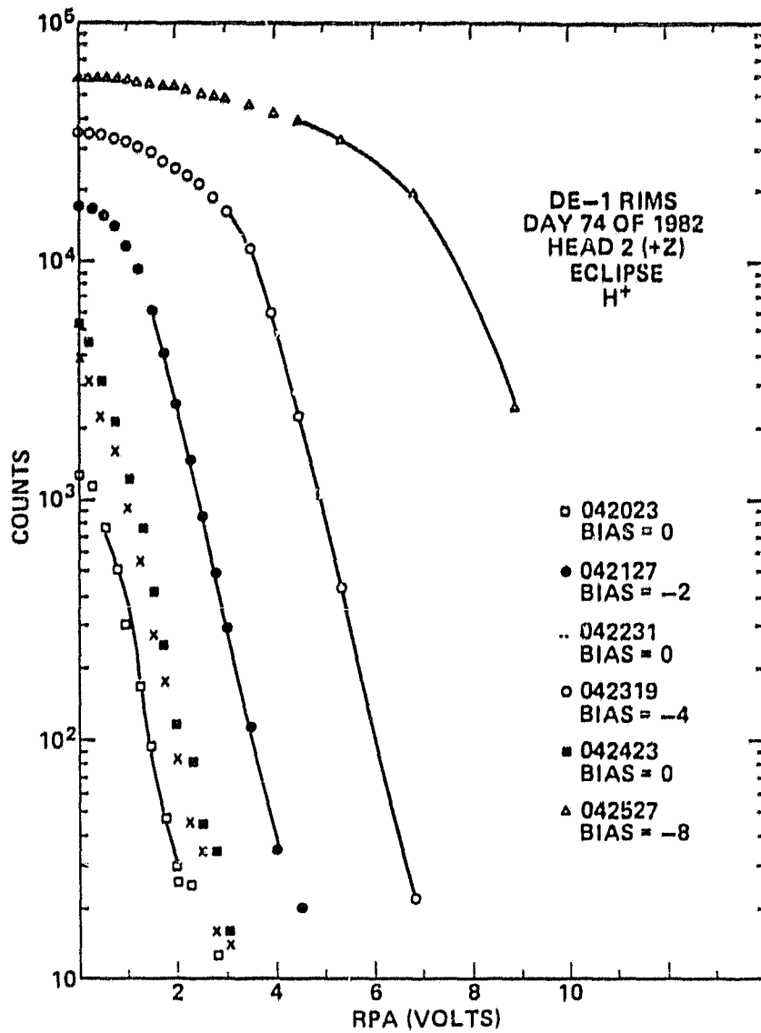
Figure 23. Examples of RPA curves showing the normal effect of increasing aperture plane bias.
