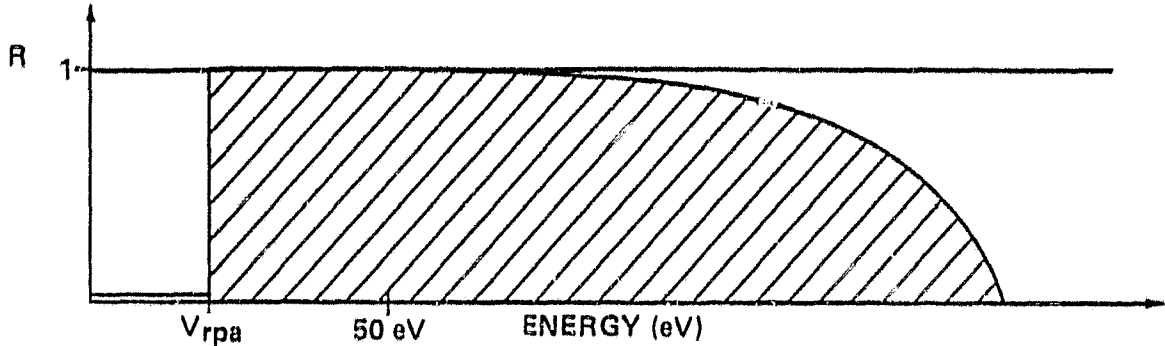
Figure 3. Similar to Figure 1 with width larger than 50 V V_{rpa} limit. It is then possible to derive I(E) using a simple differencing technique:
