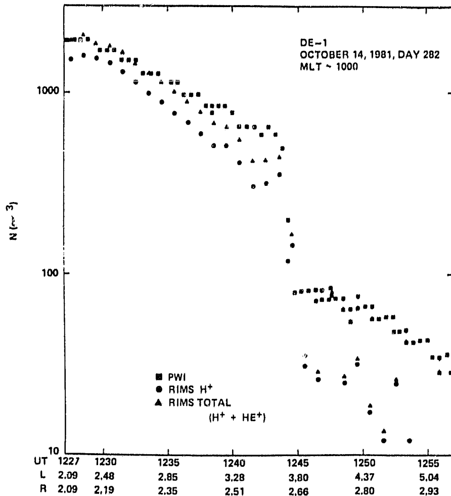
Figure 10. Comparison of RIMS ion density measurements and electron densities derived from the DE 1 Plasma Wave Instrument.
