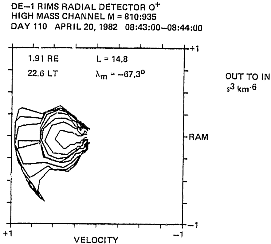
Figure 5. Cold rammed O^+ distribution function in space velocity coordinates with full scale velocity corresponding to 50 eV O^+ (24 km/s). Contours are separated by a factor of approximately 2.0.
