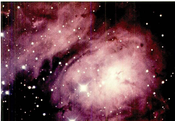
Figure 33. Interstellar Medium
