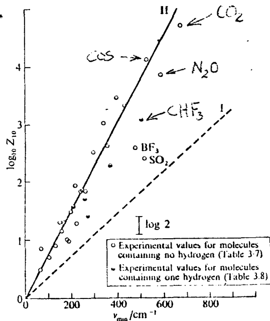
Lambert-Salter plot for molecules containing \leq 1 hydrogen atom
