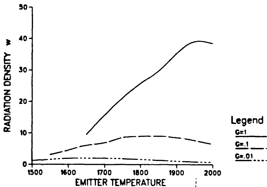
Figure 9. Radiation output vs. emitter temperature.
