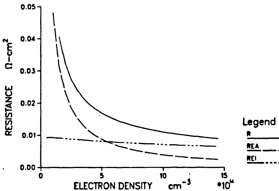
Figure 3. Plasma resistance vs. electron density.
