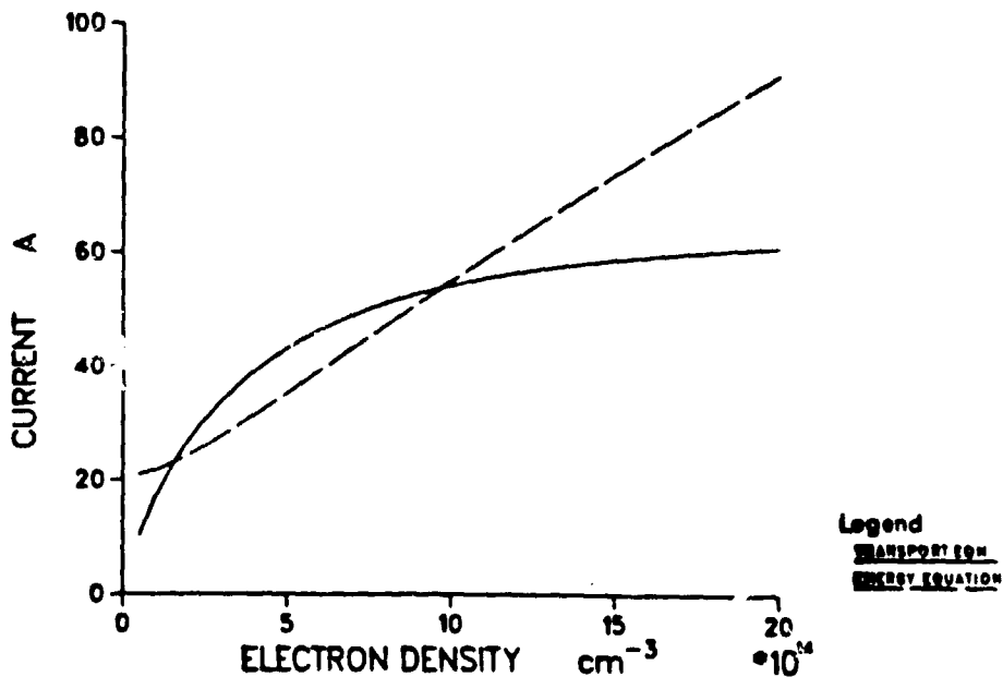
Figure 6. Solutions to the transport and energy equations.
