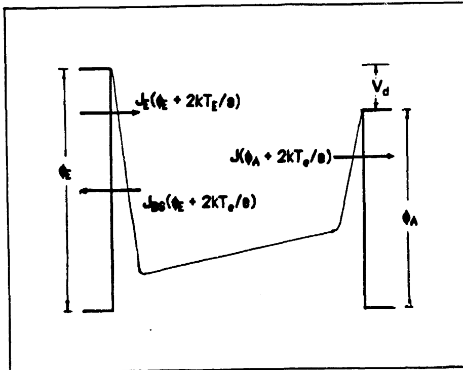
Figure 4. Energy fluxes for emitted electrons.
