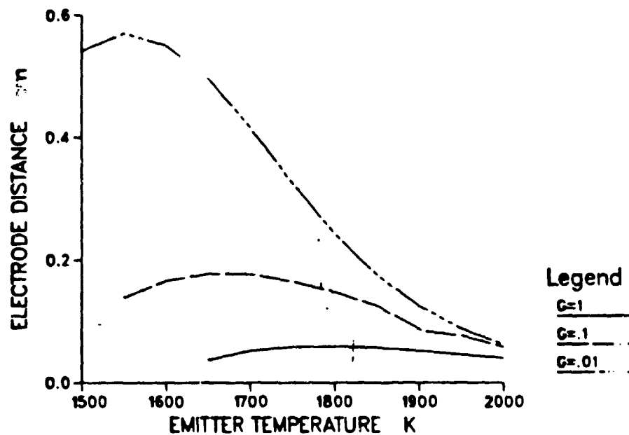
Figure 11. Maximum Inter-electrode spacing vs. emitter temperature.
