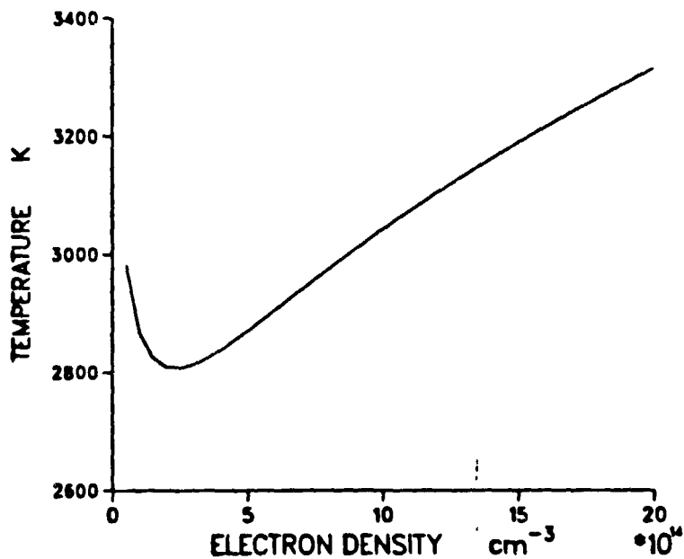
Figure 5. Solution to the ambipolar diffusion equation.
