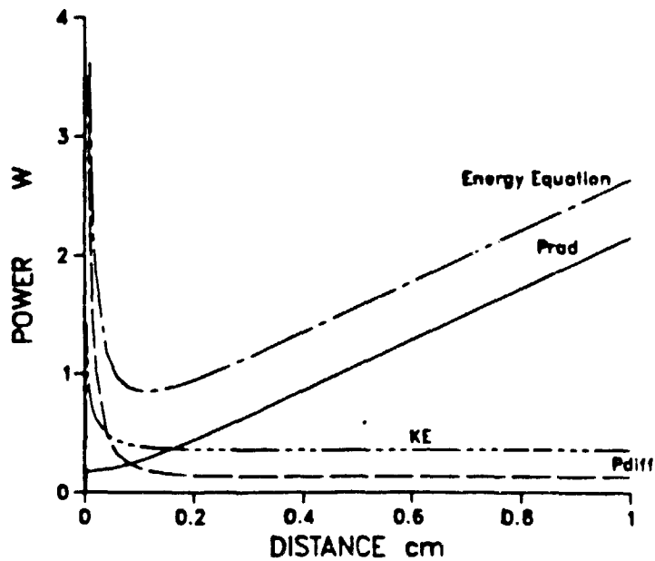
Figure 10. Energy losses as a function of inter-electrode spacing.
