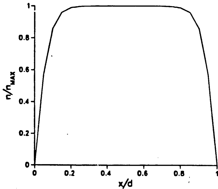
Figure 2. Electron distribution under Saha conditions.
