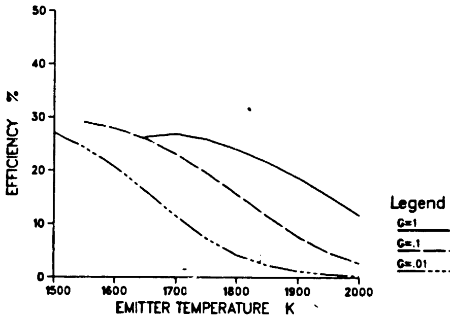
Figure 7. Efficiency vs. emitter temperature.
