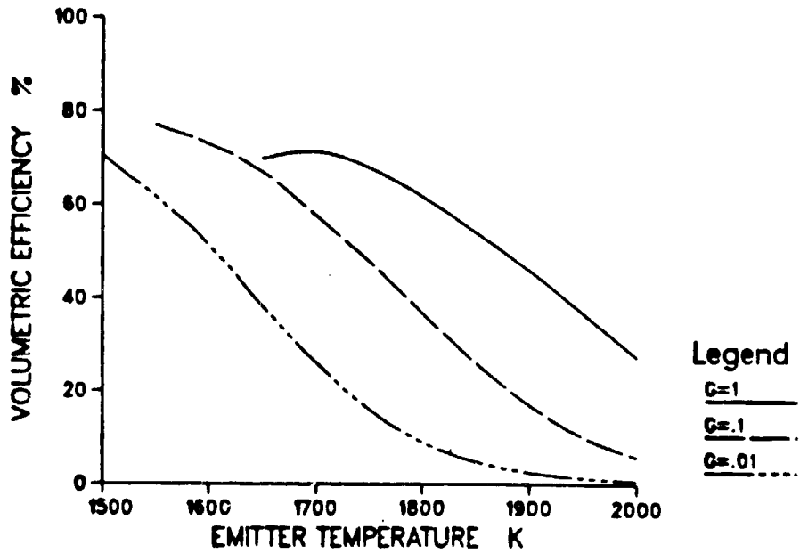
Figure 8. Volumetric efficiency vs. emitter temperature.
