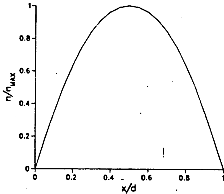
Figure 1. Electron distribution under non-Saha conditions.
