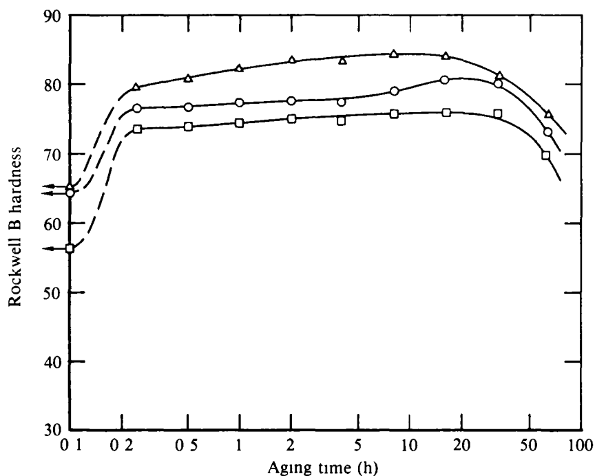
Figure 29. Aging behavior at 190°C of non-Li-containing VA extrusions: (○, □) Al-4.4Cu-1.5Mg-1Fe-1Ni-0.2Zr; (○) solution-treated 530°C/1 h, (□) solution-treated 500°C/1 h, (Δ) Al-4.4Cu-1.5Mg-2Fe-2Ni-0.2 Zr, solution-treated 530°C/1 h.
