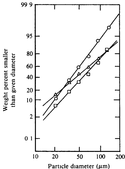
Figure 6. Particle size distributions of Al-4.4Cu-1.5Mg-1Fe-1Ni-0.2Zr powders: (○) Vacuum atomized, (□) argon ultrasonically atomized, and (△) helium ultrasonically atomized.
