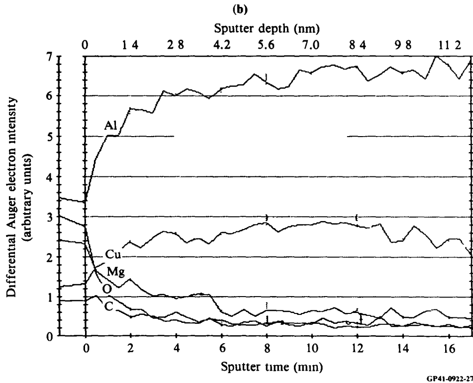
Figure 17. Scanning Auger Microscope (SAM) results for as-vacuum-atomized Al-4.4Cu-1.5Mg-1Fe-1Ni-0.2Zr particle: (a) Auger electron spectrum of as-received particle, (b) depth profile of Al, Cu, Mg, O, and C concentrations, sputtering rate 0.7 nm/min, and (c) Auger electron spectrum of underlying matrix.
