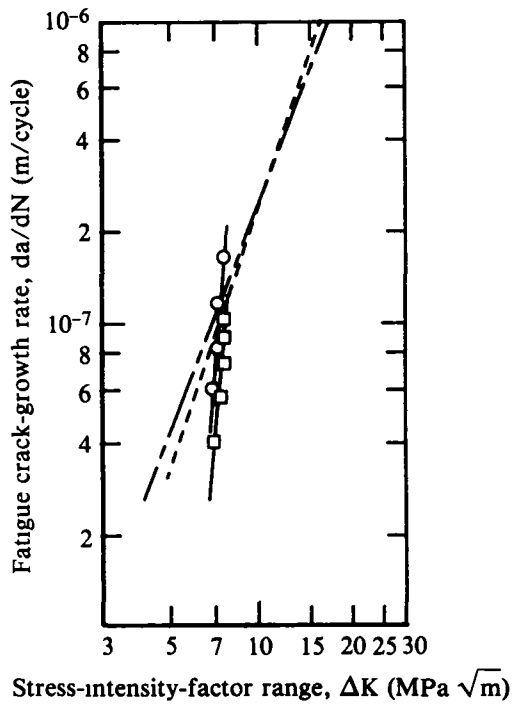
Figure 59. FCGR results on Al-3Li-1.5Cu-1Mg-0.5Co-0.2Zr VA forgings, T851/530 temper: (○) LT orientation, (□) TL orientation, (---) typical results for 7075-T651 (24), and (-.-) typical results for 7091-T7E69(24).
