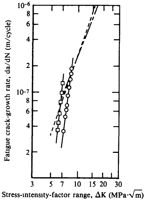
Figure 58. FCGR results on Al-3Li-1.5Cu-1Mg-0.5Co-0.2Zr VA extrusions, T851/530 temper: (○) LT orientation, (□) TL orientation, (---) typical results for 7075-T651 (24), and (-.-) typical results for 7091-T7E69(24).
