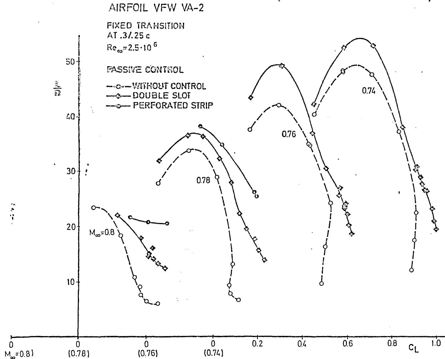
Fig. 13: EFFECTS OF THE PASSIVE BL CONTROL ON L/D NUMBER
