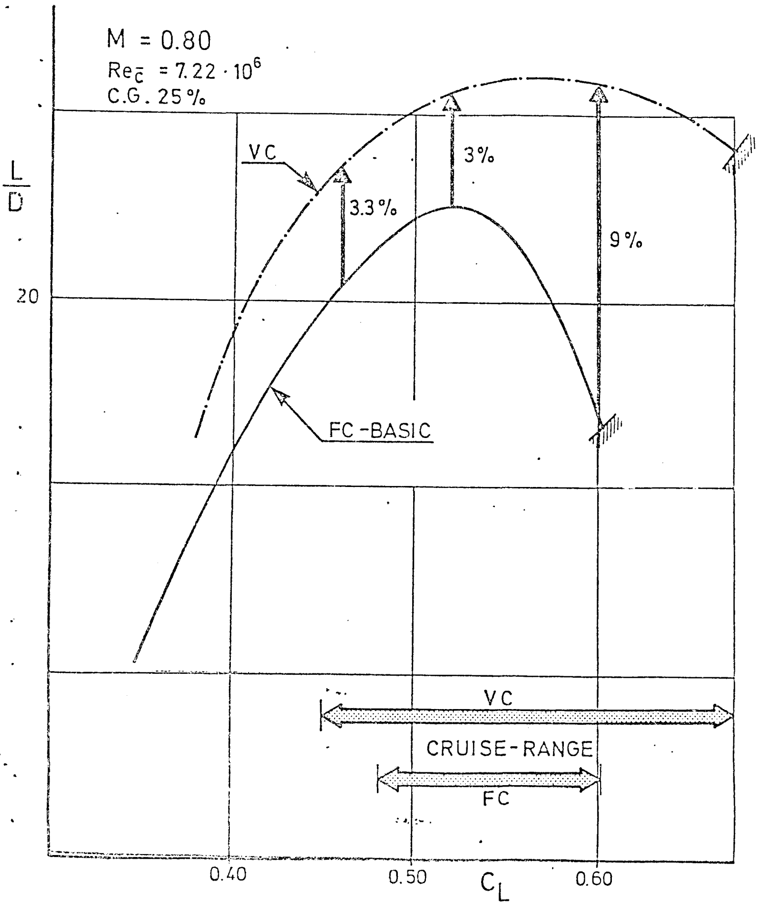
Fig.5 : INFLUENCE OF THE VARIABLE CAMBER ON THE LIFT DRAG RATIO
