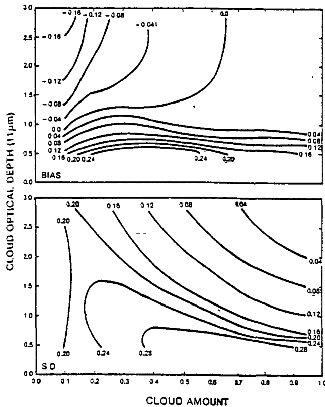
Fig. 7d Bias and Standard Deviation of Computed Cloud Emissivity for Various Assumed Cloud Amounts and Optical Depths (cloud heights assumed at 300 mb)
