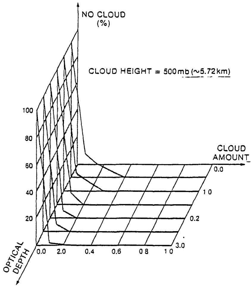
Fig. 8a. Cloud Amount versus Optical Depth (restrictive criterion used ) for Cloud Ht at 500 mb.
