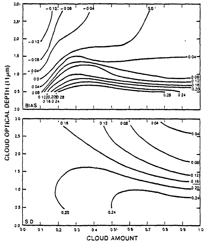
Fig. 9d. Bias and Standard Deviation of Computed Cloud Emissivity for Various Assumed Cloud Amounts and Optical Depths (cloud heights assumed at 700 mb)
