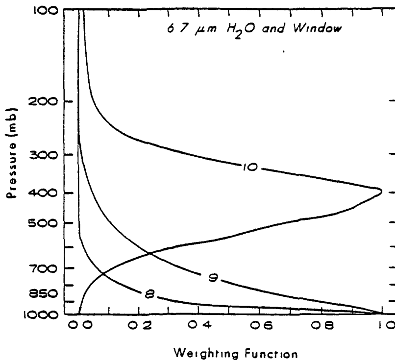
FIG 1. HIRS/2 Weighting Functions: Weighting functions of the HIRS/2 15 \mu\text{m CO}_2 , 6.7 \mu\text{m H}_2\text{O} and window channels.
