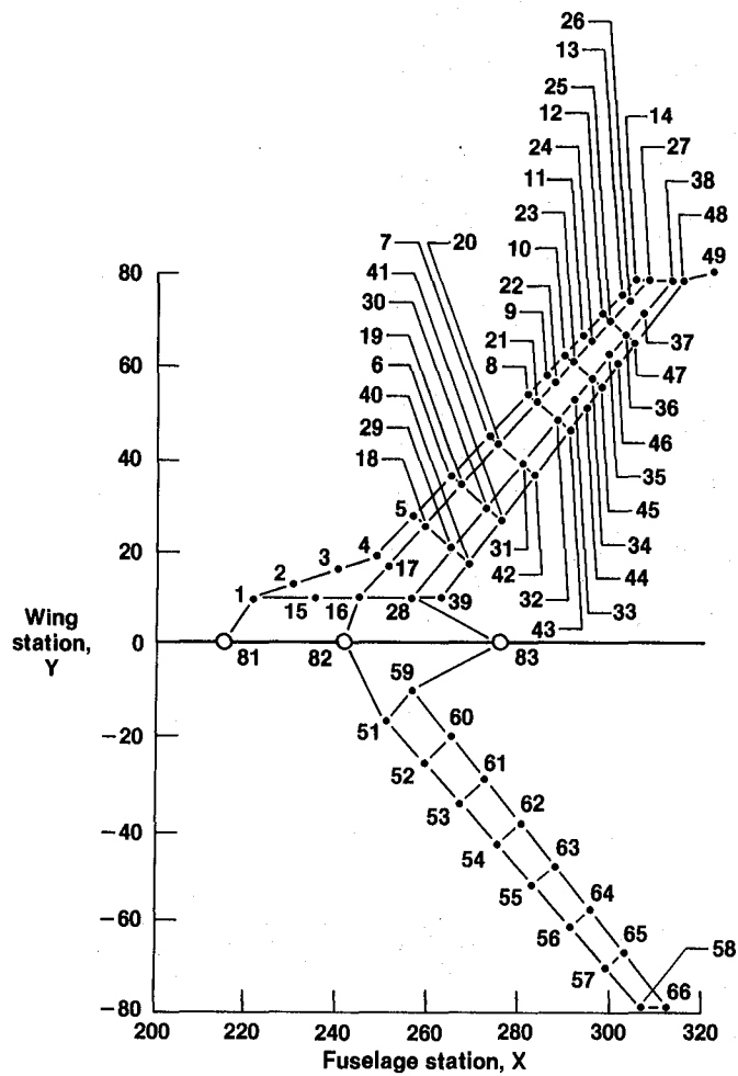
Figure 9. Test coordinates of right and left wings.
