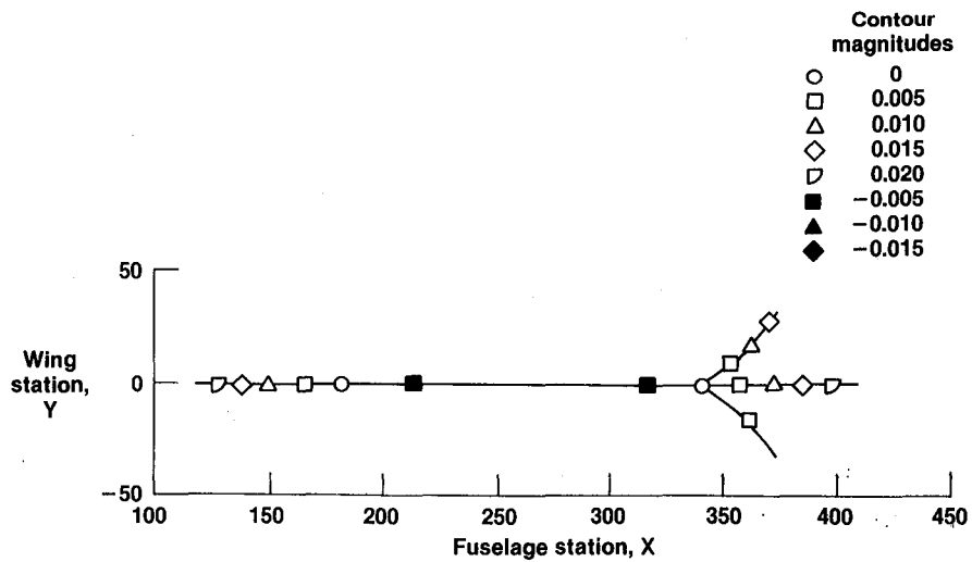
Figure 15. First symmetric vertical fuselage bending mode.
