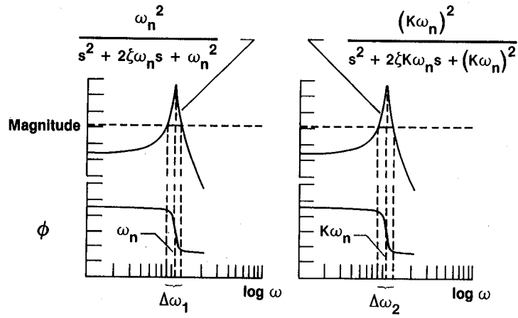
Figure 24. Effect of natural frequency on amount of data available for analysis.
