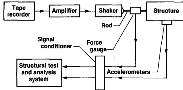
Figure 12. Data collection process.
