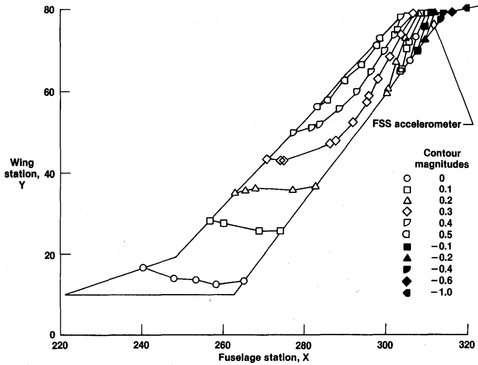
Figure 14. Second symmetric wing bending/torsion mode.
