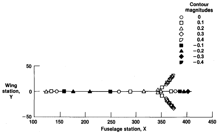
Figure 16. Second symmetric vertical fuselage bending mode.
