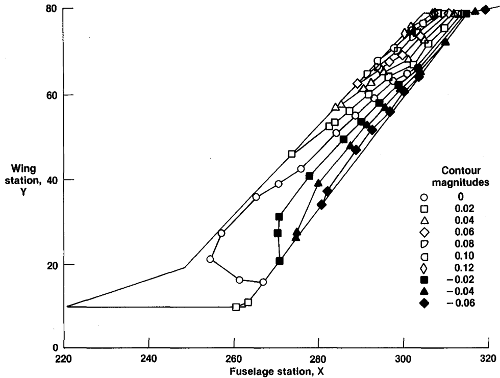
Figure 17. Unidentified symmetric mode (significant wing torsion).
