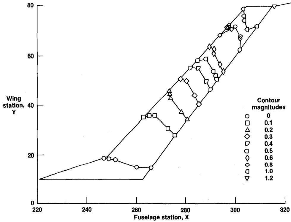
Figure 13. First symmetric wing bending mode.
