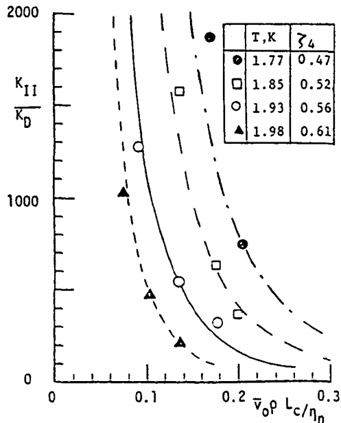
Fig. 3. Permeability ratio for various bath temperatures [6] of a 1 μm plug with K_D = 2.5 \cdot 10^{-12} \text{ cm}^2 .
