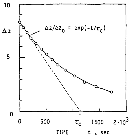
Figure 3. Example of outflow run: Liquid level difference vs t; (liquid N 2 , 1 atm ).
