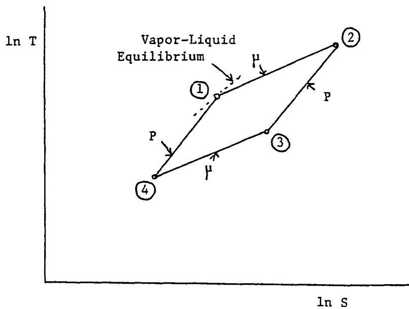
Fig. D.1 . Cycle in the \ln T vs \ln S diagram, schematically; S entropy
