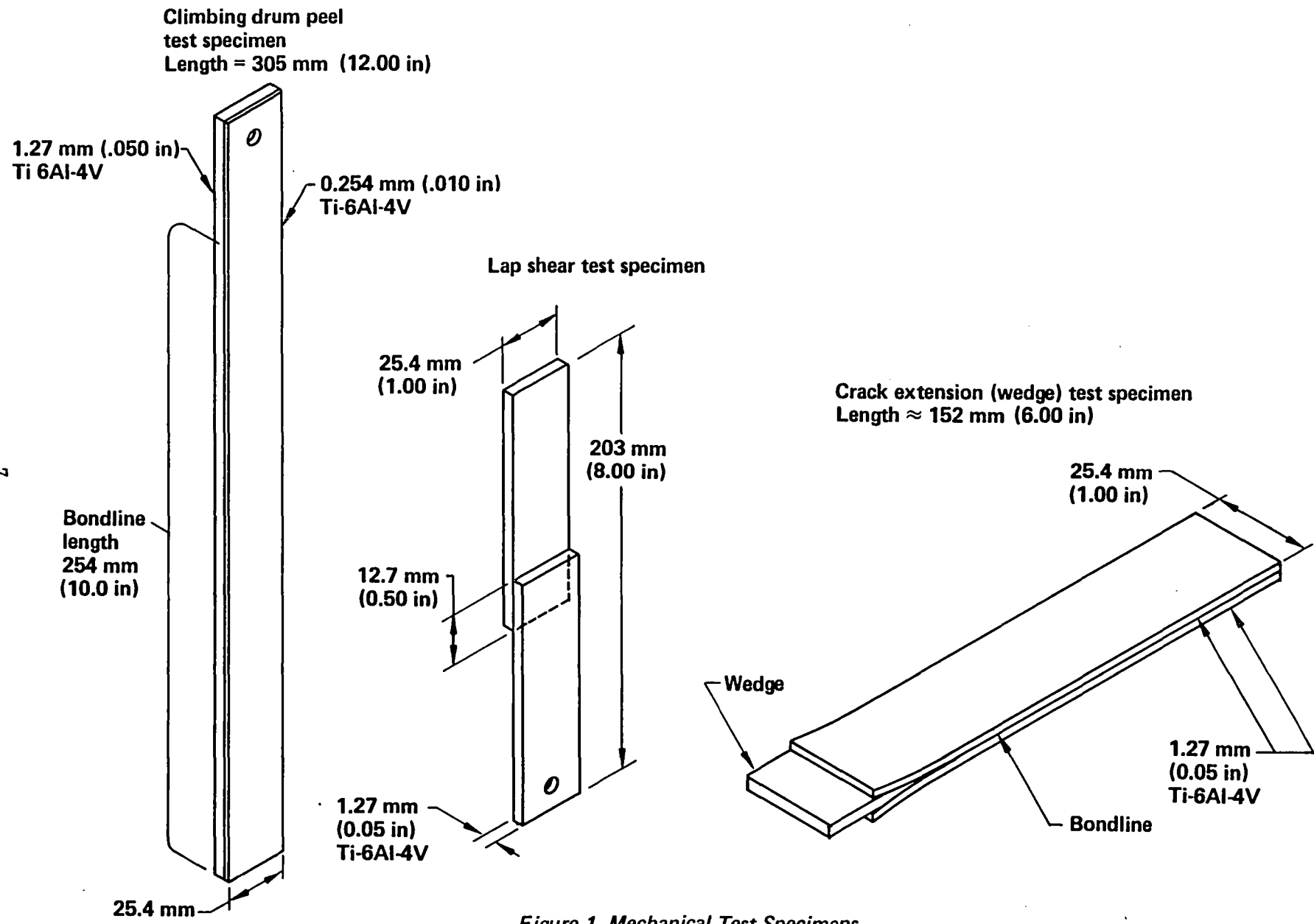
Figure 1. Mechanical Test Specimens
