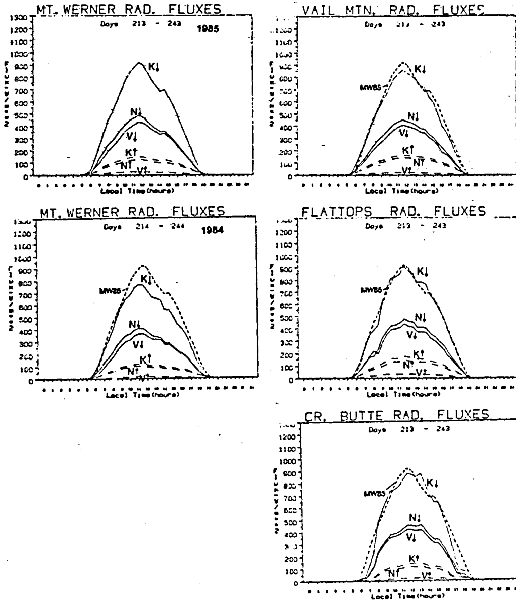
Fig. 14. Diurnal average values for incoming and reflected components of solar radiation during August 1984 at Mt. Werner and at the 1985 ROMPEX sites. Label designations are total solar (K), near infrared (N), and visible (V). The dashed curve labeled mw 85 in several of the plots represents the K + value for the Mt. Werner site for August 1985.
