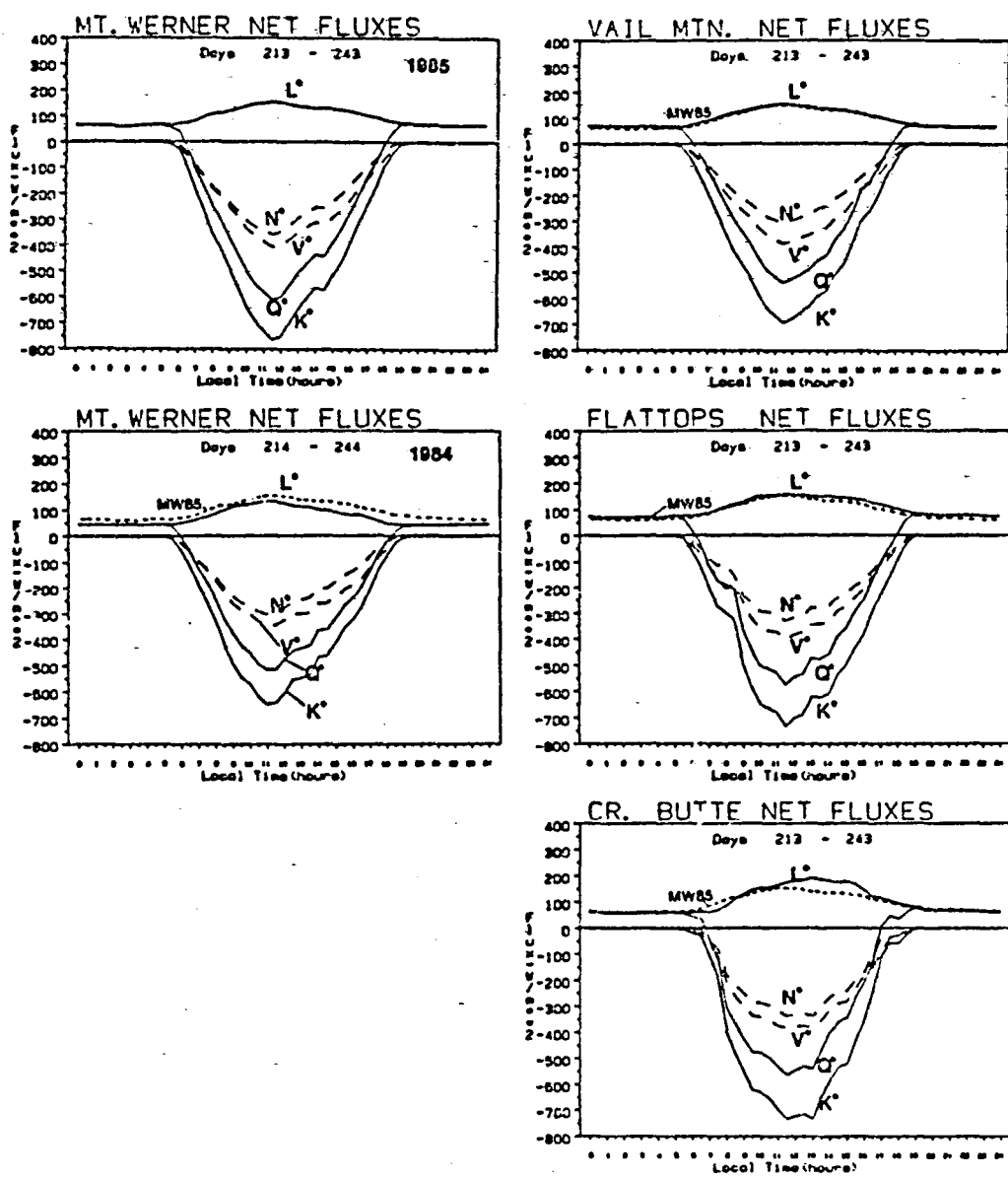
Fig. 16. As in Fig. 14 but for the net radiative fluxes. The 1985 L^* value for Mt. Werner has been added to some of the plots.
