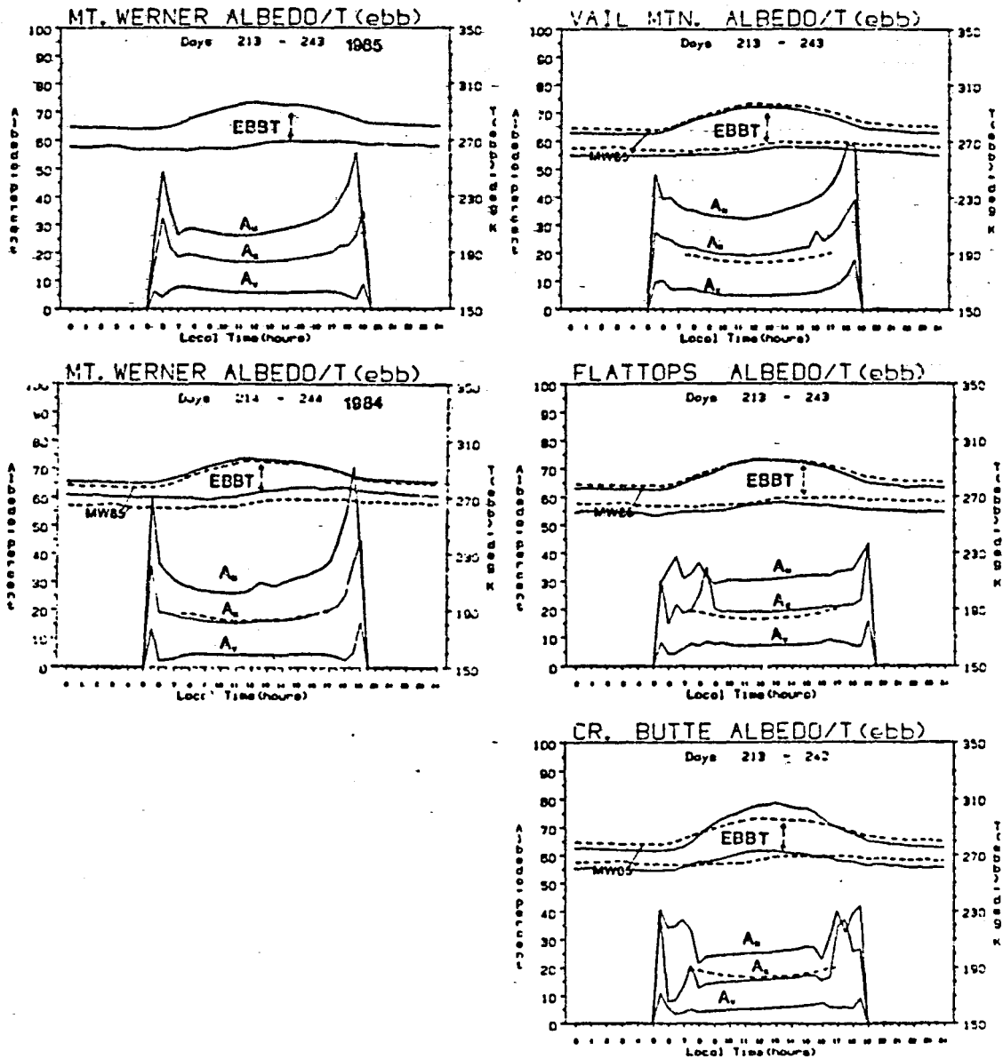
Fig. 17. As in Fig. 14 but for the surface albedo and EBBT values for each site. The 1985 EBBT curves and a portion of the A_K (total solar albedo) curve for Mt. Werner have been included in some plots.
