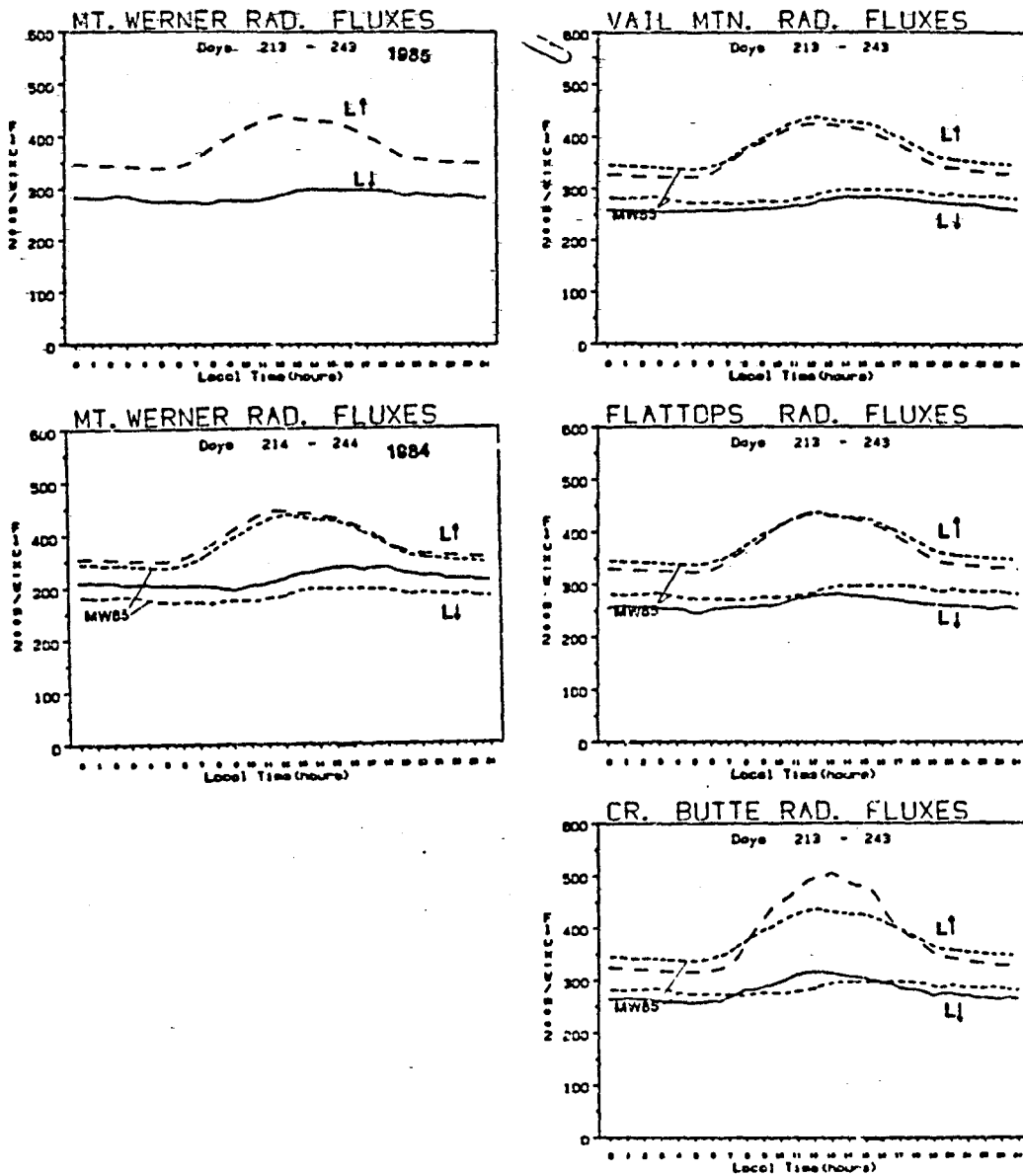
Fig. 15. As in Fig. 14 but for atmospheric (L+) and surface (L+) emitted infrared radiation. The 1985 Mt. Werner data are again included for comparison.
