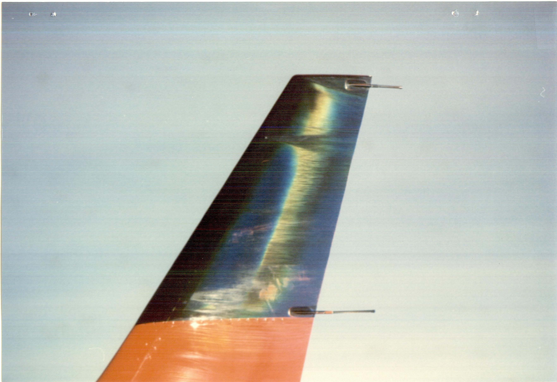
Figure 1. - Transition visualization using liquid crystals on winglet of Lear 28/29 Airplane. Pressure altitude = 48,000 ft., M = 0.8 ; leading edge sweep = 31^\circ .
