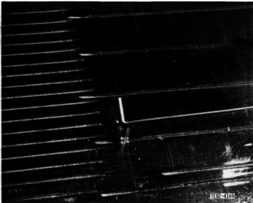
Figure 9. Installation of vane surface static pressure taps.
