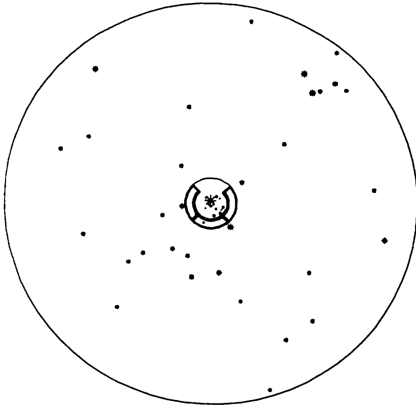
Figure 5c. Telescope's FOV and nearby stars. (Note Polaris in the center and Ursa Minor in the lower half of the disk.)
