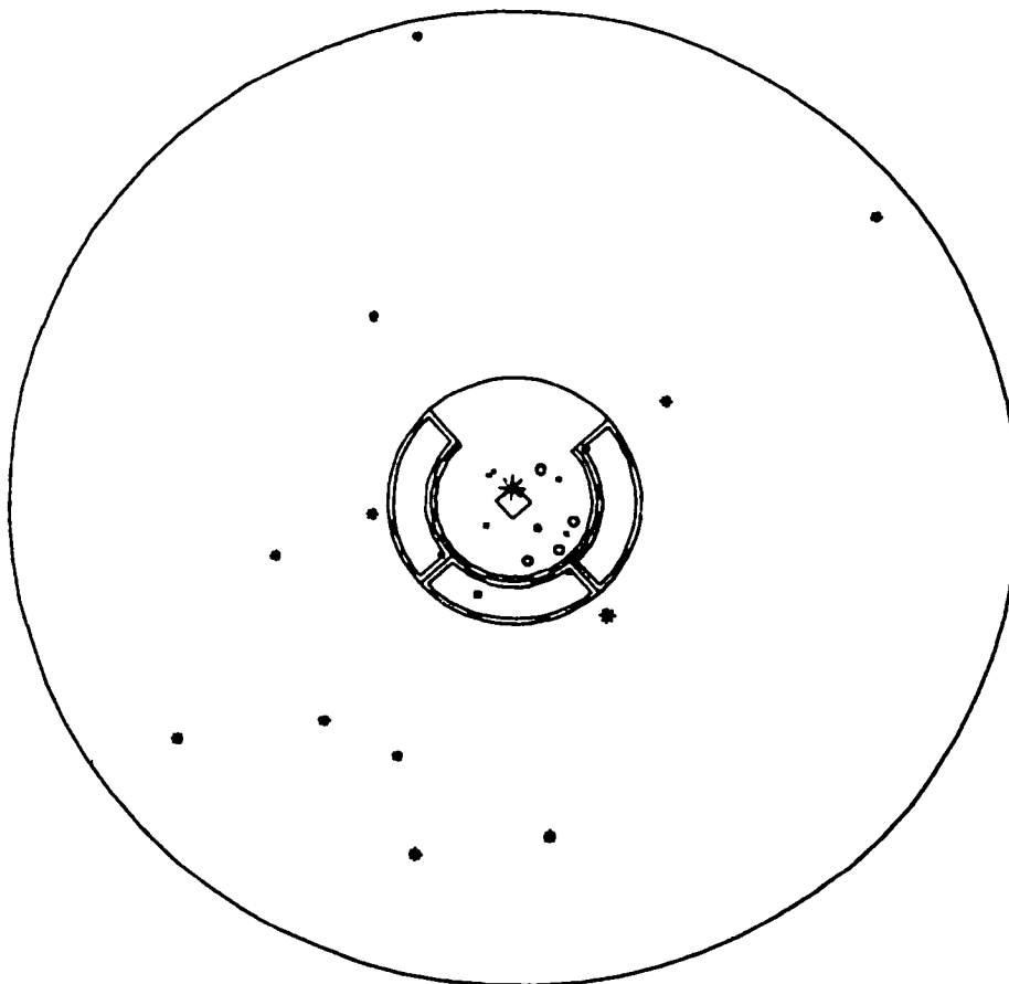
Figure 7a. Two degree FOV at RA of 27 deg, DL of 89 deg showing the 0.5 deg wide HST FOV.
