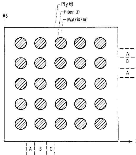
Figure 4.—Definitions of regions for ply microstress calculations.
