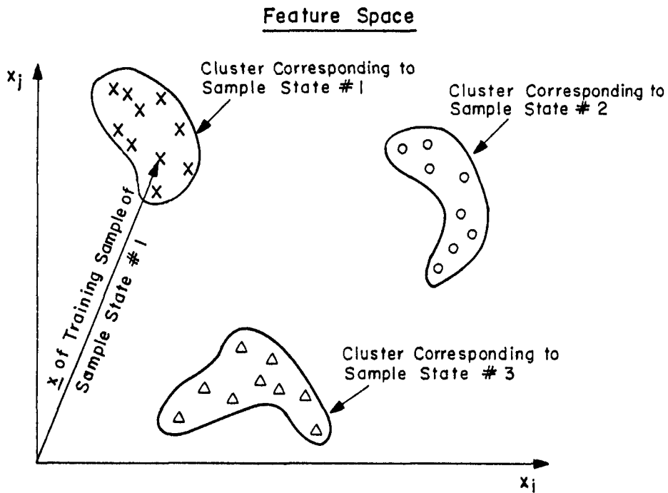
Fig. 2 Two-dimensional representation of feature space formed using i-th and j-th components of feature vectors, illustrating separate clusters of feature vectors \underline{x} of training samples having distinct sample states.
