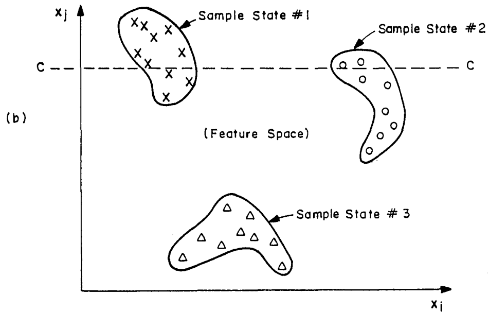
Fig. 3 Schematic illustrating (a) discriminant functions g_k(\underline{x}) along a line C-C in feature space shown in (b).
