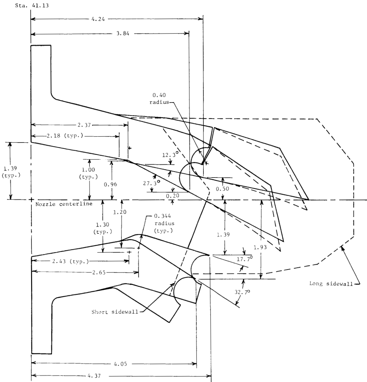
(c) Nozzles vectored 15° and 30° with 2.7° divergence angle.
