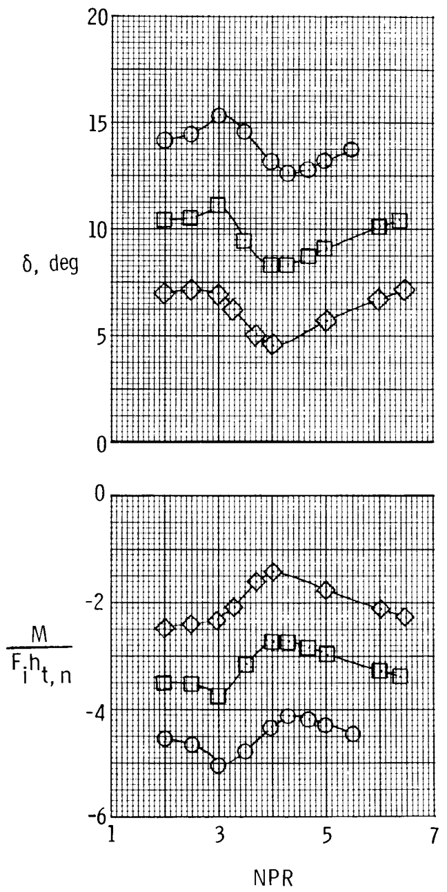
(b) Configuration A3CS, \delta_v = 4.15^\circ .
