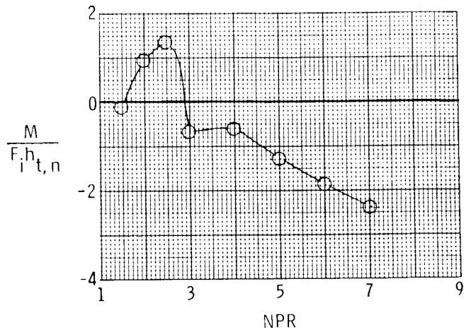
Figure 23.- Variation of nozzle performance parameters with nozzle pressure ratio for dry power thrust-reverser configuration.
