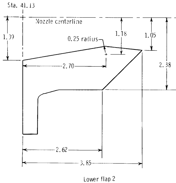
(b) Vertical takeoff or landing nozzle lower flaps.
