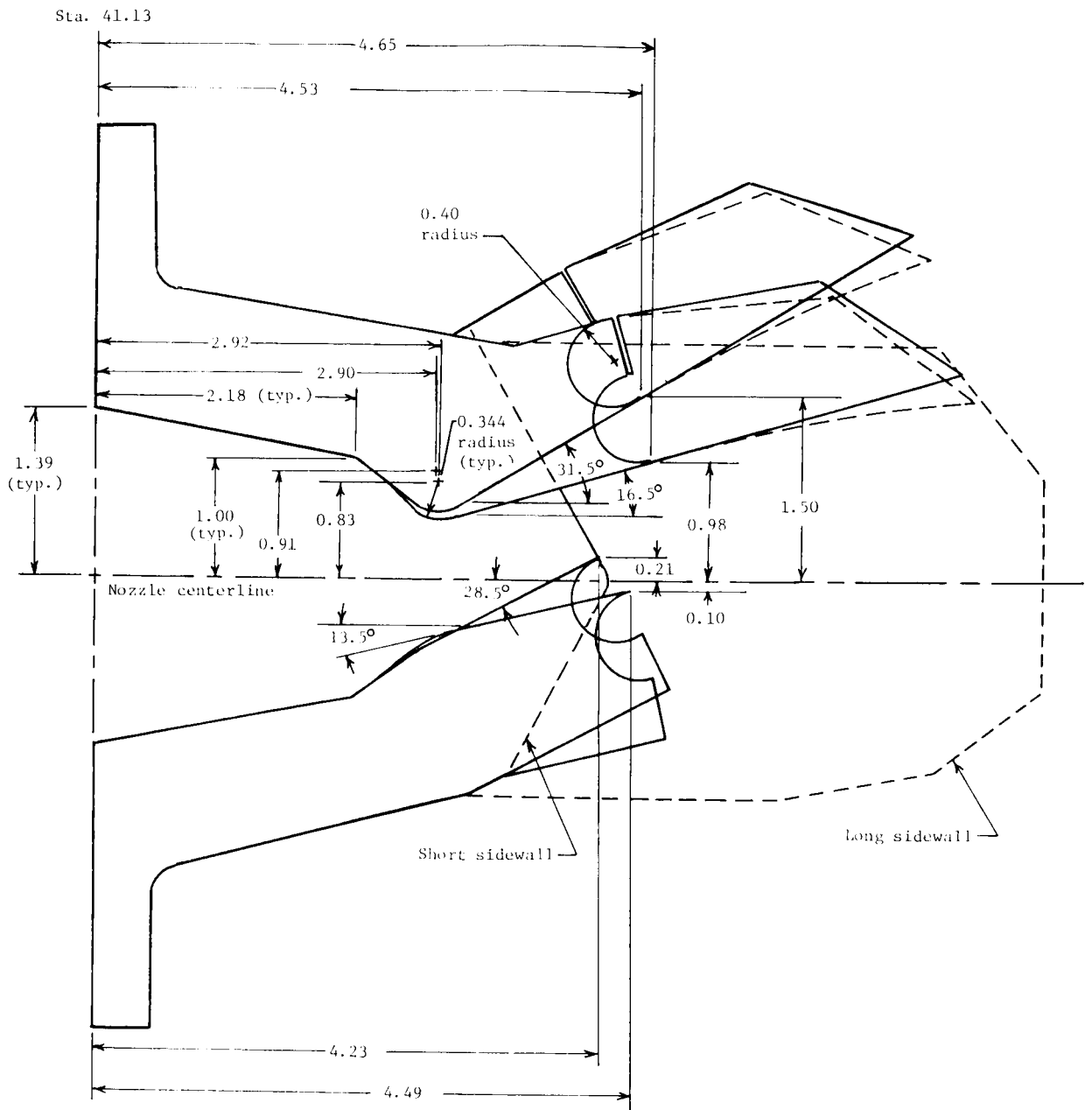
(b) Nozzles vectored -15^\circ and -30^\circ .
