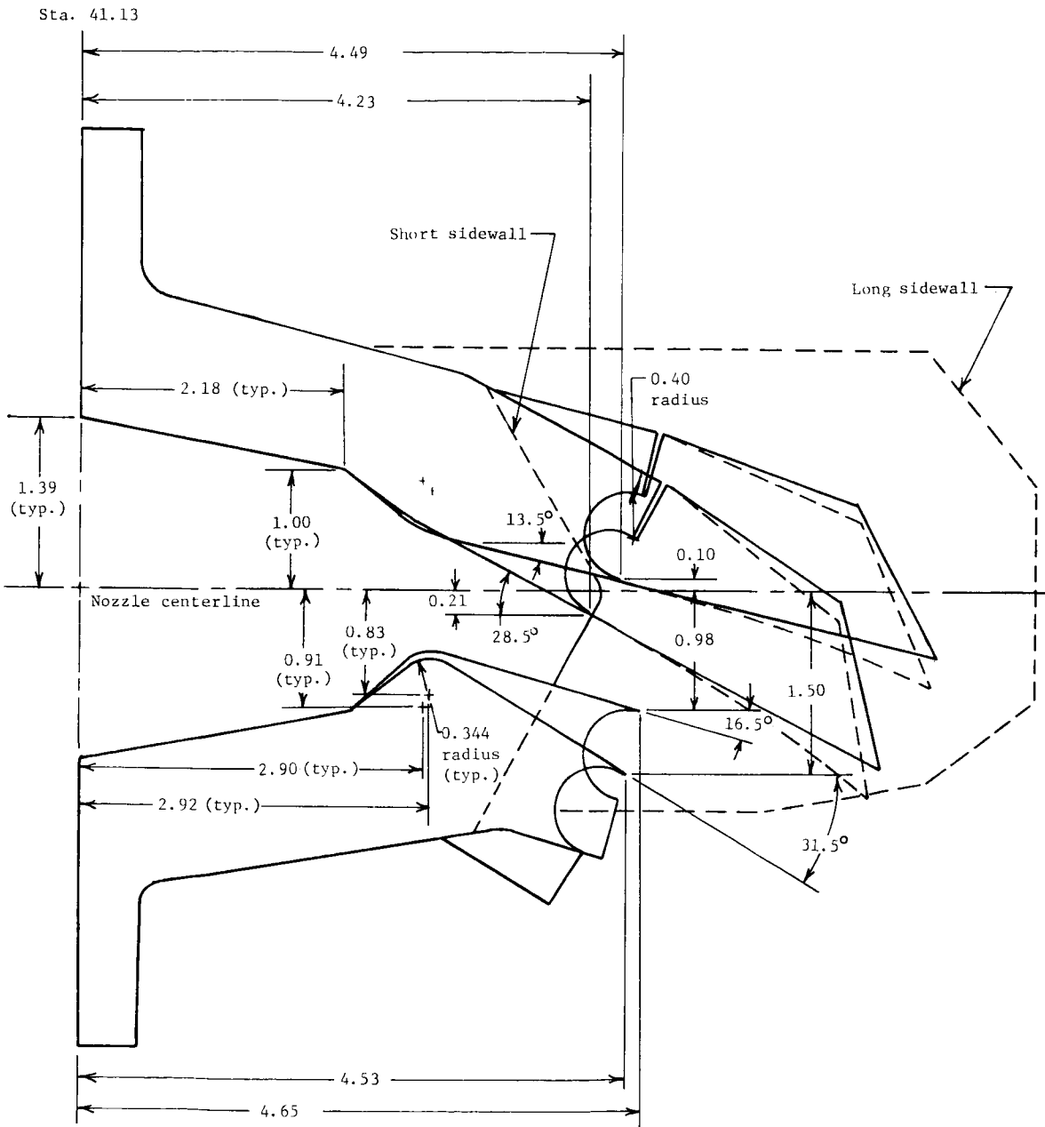
(c) Nozzles vectored 15° and 30°.
