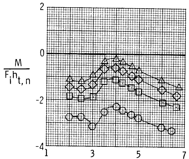
(c) Configuration A3FS, \delta_v = 4.15^\circ .
