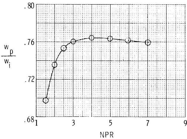
Figure 23.- Variation of nozzle performance parameters with nozzle pressure ratio for dry power thrust-reverser configuration.
