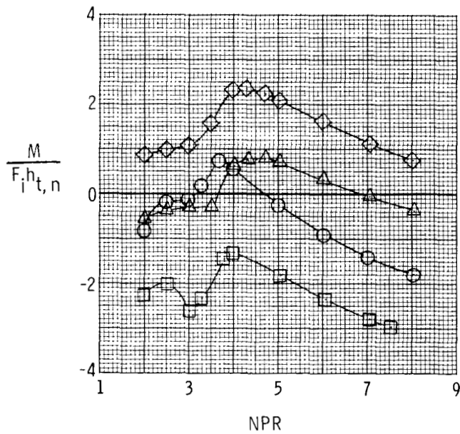
Figure 20.- Variation of nozzle performance parameters with nozzle pressure ratio for partial afterburning configurations with flat and curved aft flaps.
