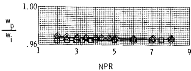
Figure 20.- Variation of nozzle performance parameters with nozzle pressure ratio for partial afterburning configurations with flat and curved aft flaps.
