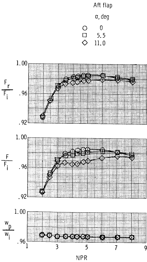
(b) Configuration P2FS, \delta_v = -4.75^\circ .
