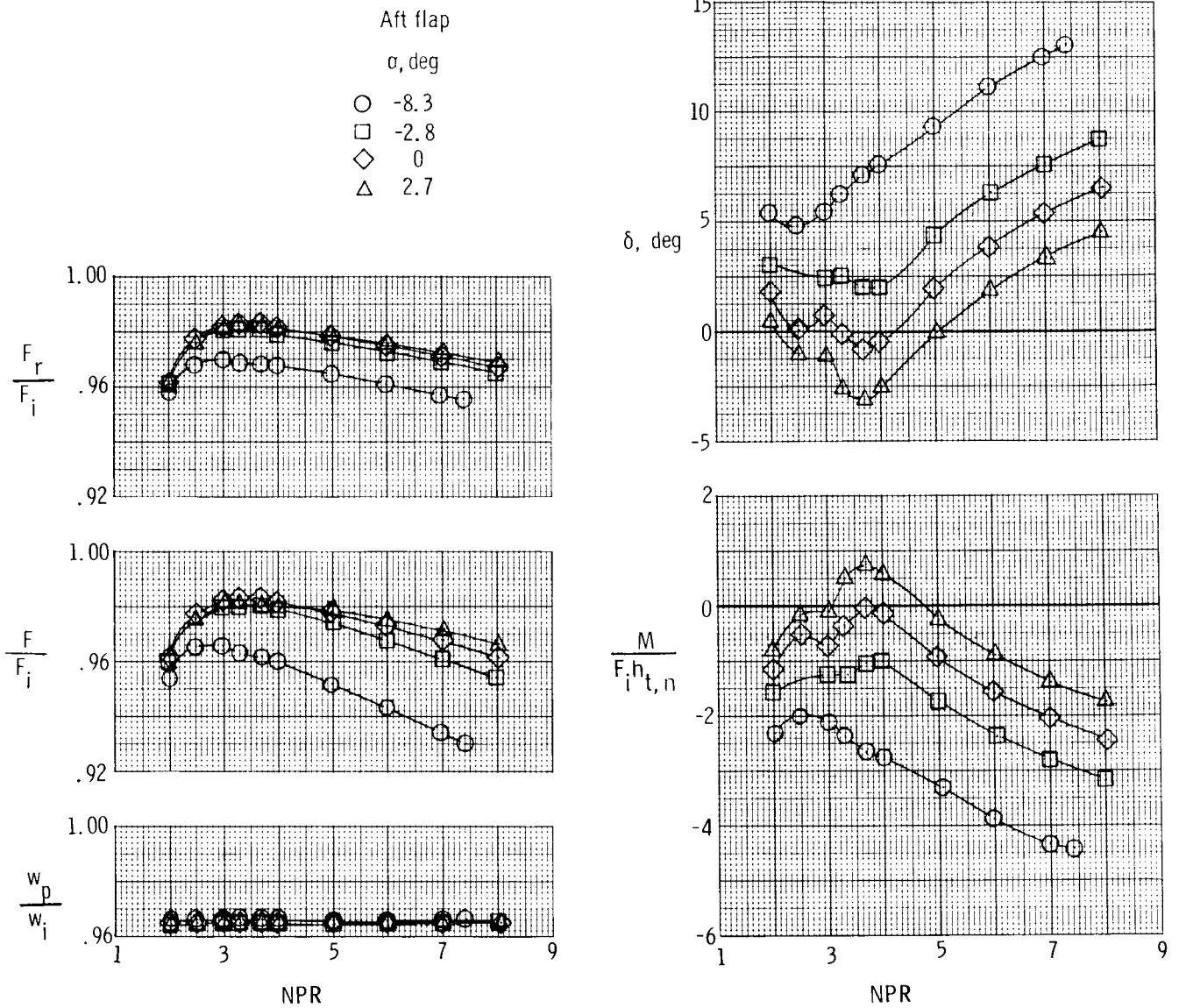
(a) Configuration P1FS, \delta_v = -0.60^\circ .
