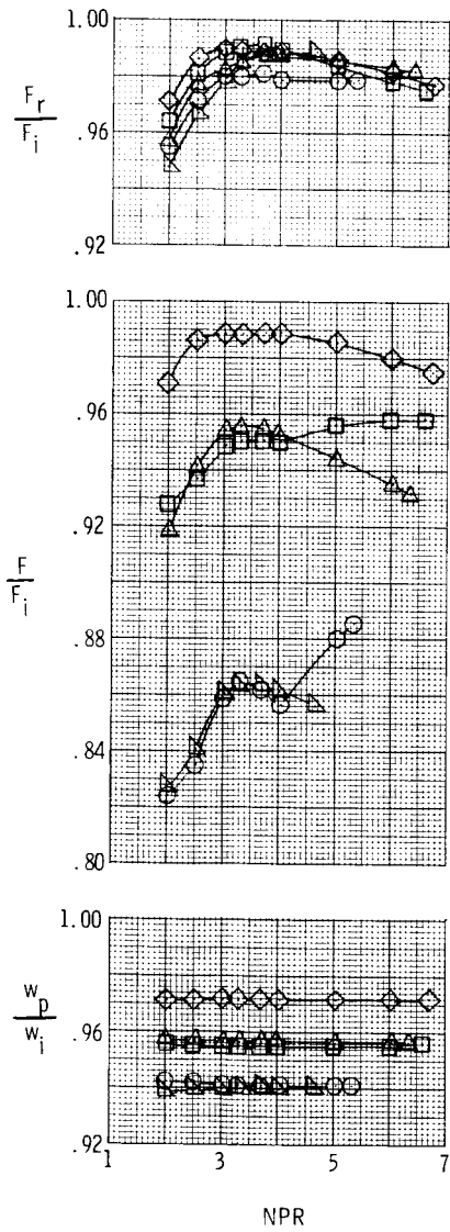
(a) Configuration A1FS.
