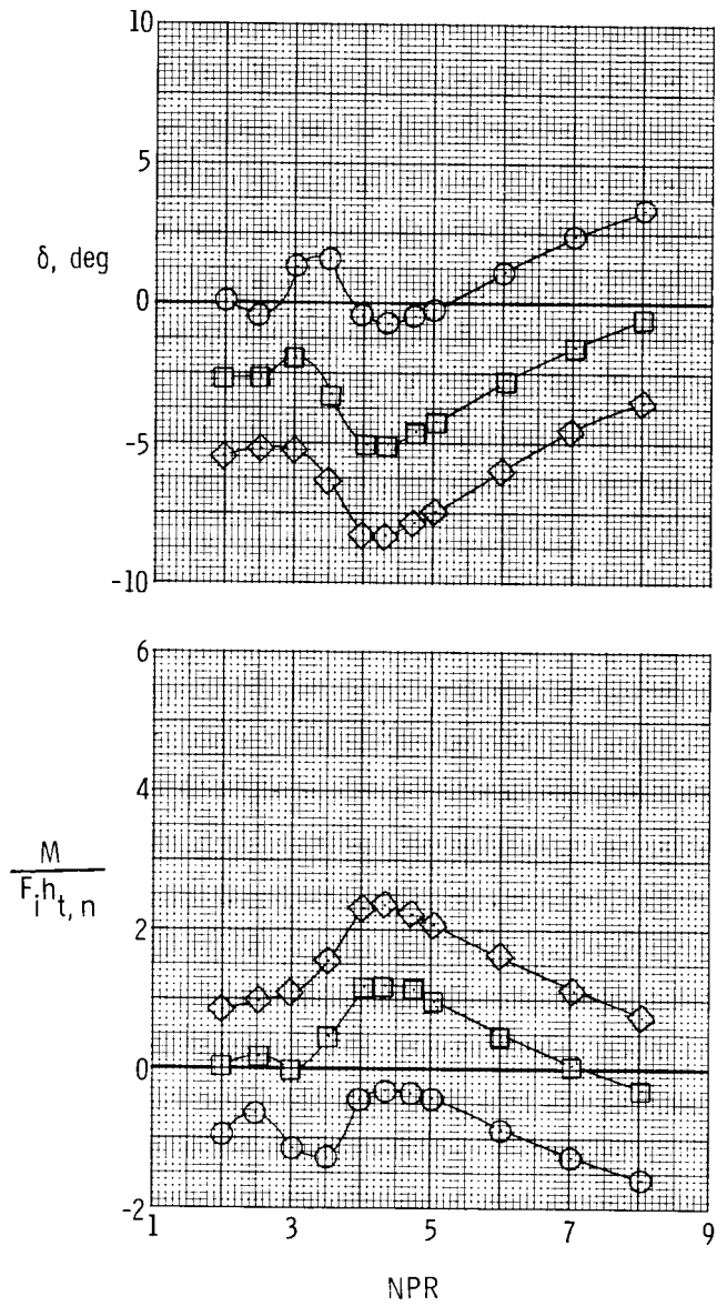
(b) Configuration P2FS, \delta_v = -4.75^\circ .
