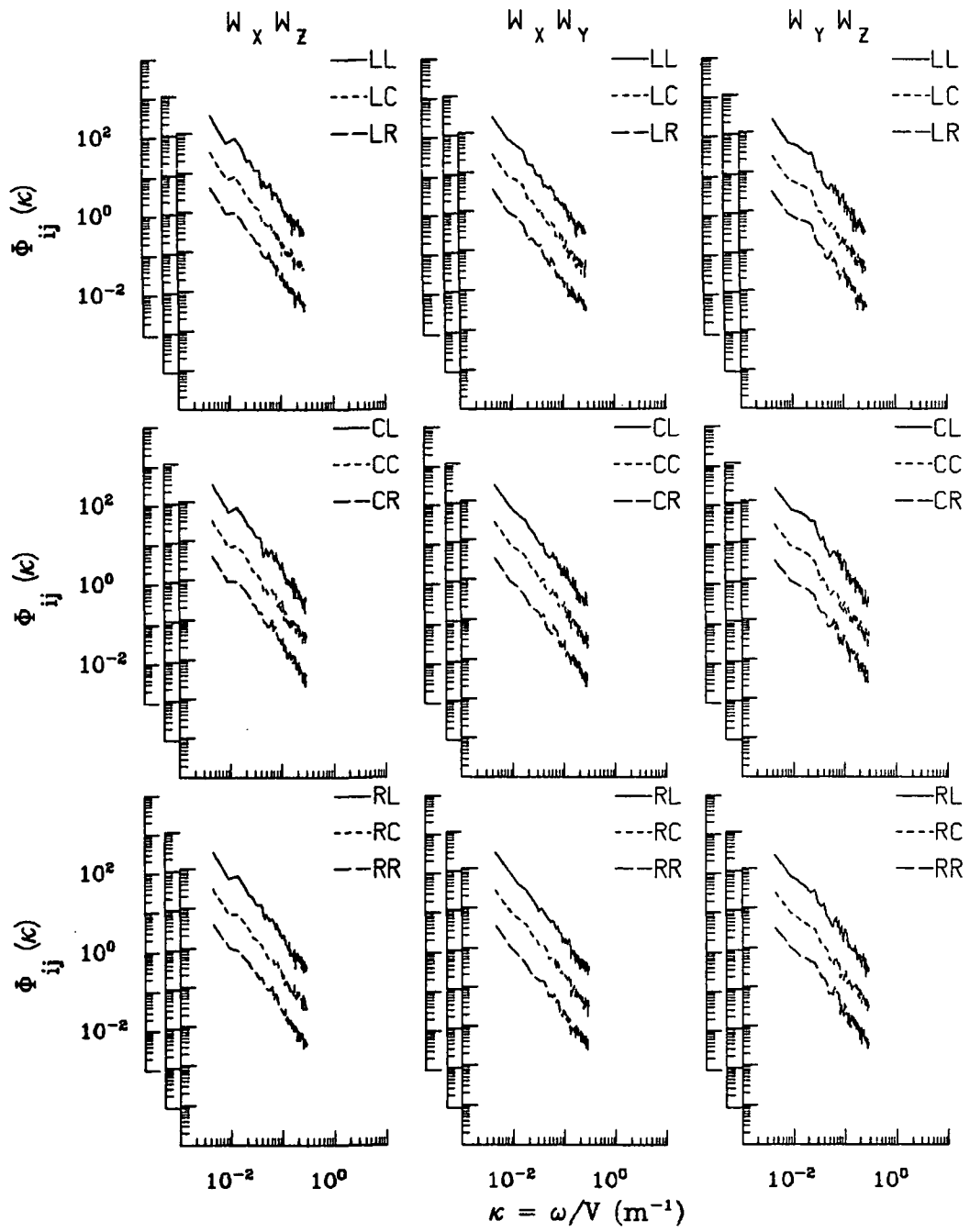
Figure A.320. Two-point cross-spectra of gust velocities, Flight 6, Run 42.
