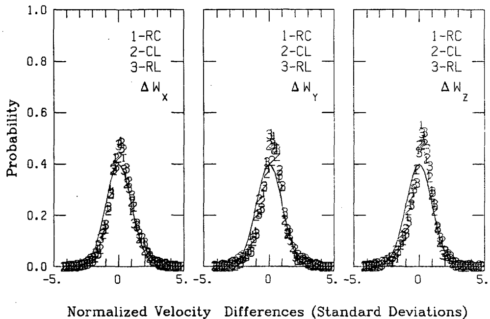
Figure A.299. Probability density function for gust velocities and gust velocity differences, Flight 6, Run 40.
