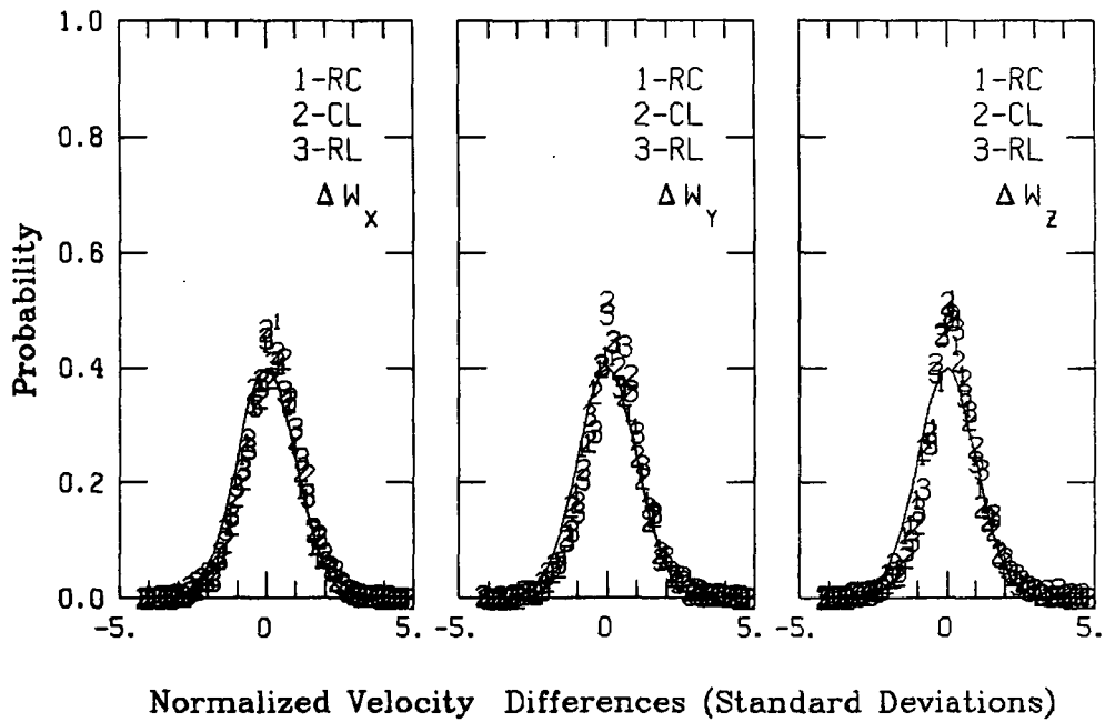
Figure A.83. Probability density function for gust velocities and gust velocity differences, Flight 6, Run 14.
