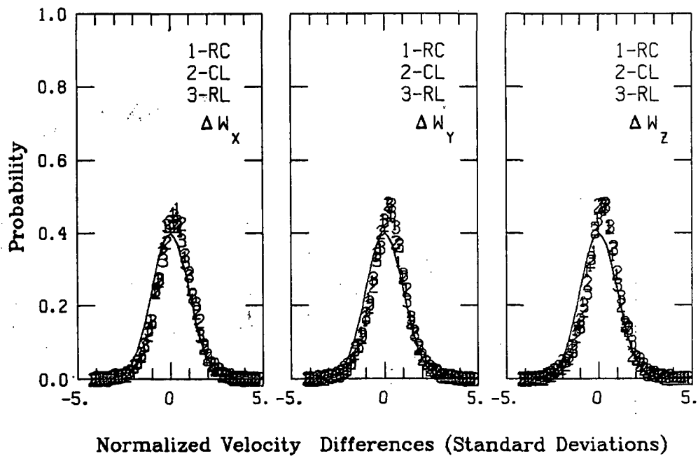
Figure A.315. Probability density function for gust velocities and gust velocity differences, Flight 6, Run 42.
