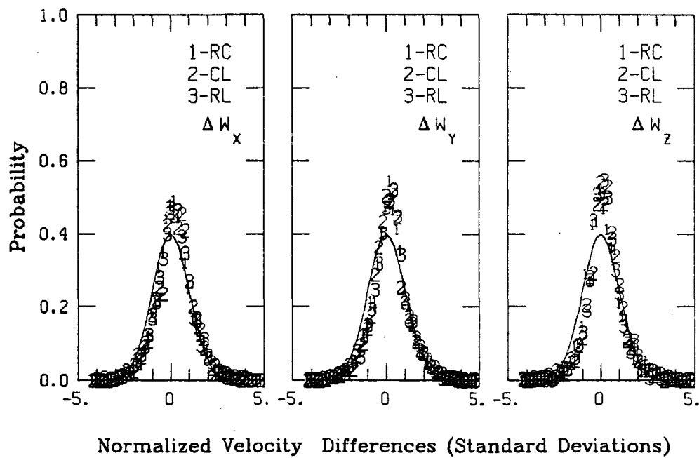
Figure A.267. Probability density function for gust velocities and gust velocity differences, Flight 6, Run 36.
