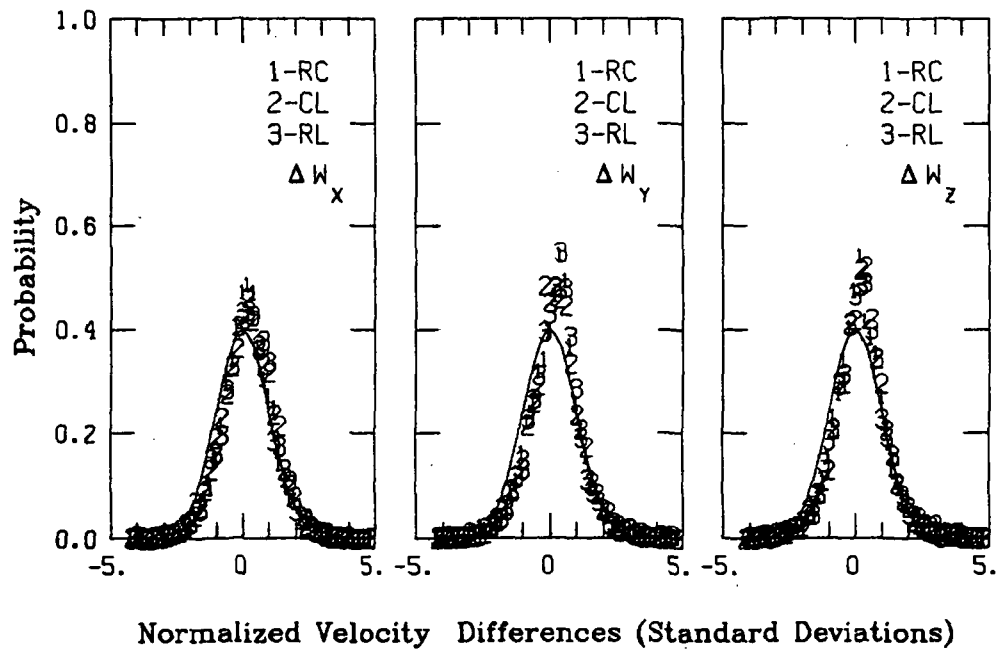
Figure A.91. Probability density function for gust velocities and gust velocity differences, Flight 6, Run 15.
