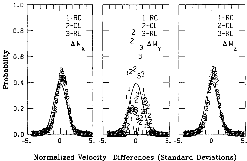
Figure A.187. Probability density function for gust velocities and gust velocity differences, Flight 6, Run 27.
