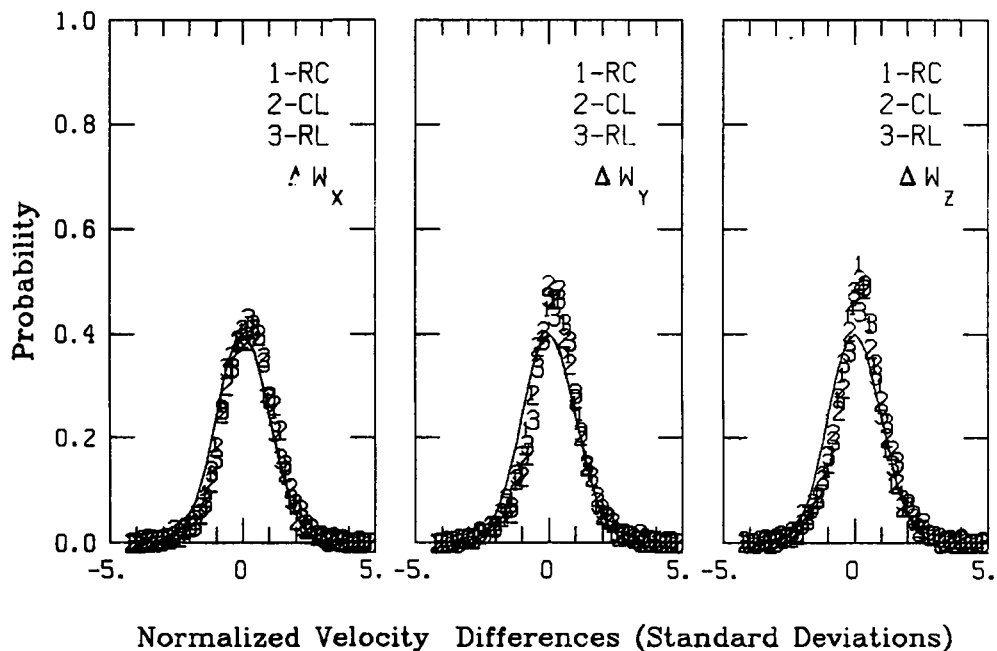
Figure A.35. Probability density function for gust velocities and gust velocity differences, Flight 6, Run 6.
