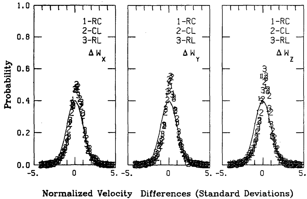
Figure A.171. Probability density function for gust velocities and gust velocity differences, Flight 6, Run 25.
