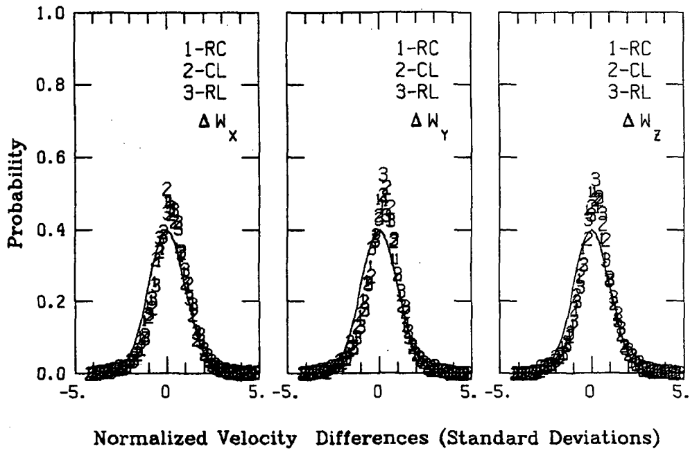
Figure A.253. Probability density function for gust velocities and gust velocity differences, Flight 6, Run 34.
