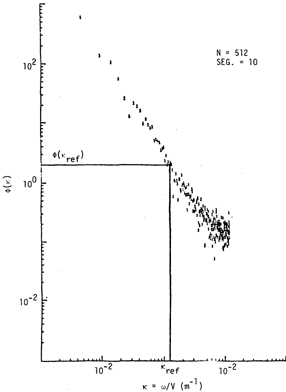
Figure 15. Illustration of selection of reference \phi(\kappa_{\text{ref}}) for normalized auto-spectra of W_{xR} velocity, Flight 6, Run 42.
