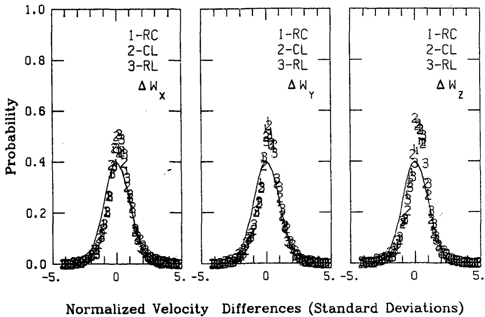
Figure A.275. Probability density function for gust velocities and gust velocity differences, Flight 6, Run 37.
