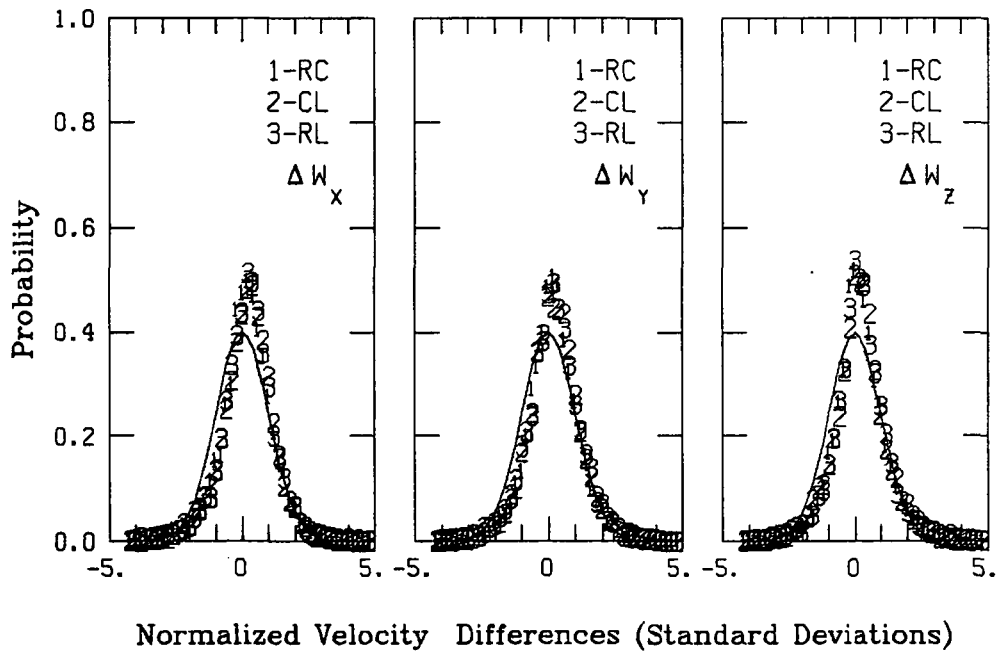
Figure A.245. Probability density function for gust velocities and gust velocity differences, Flight 6, Run 33.
