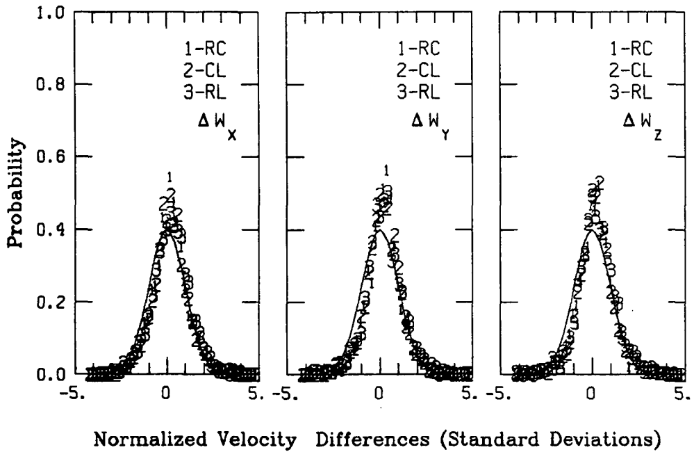
Figure A.67. Probability density function for gust velocities and gust velocity differences, Flight 6, Run 12.
