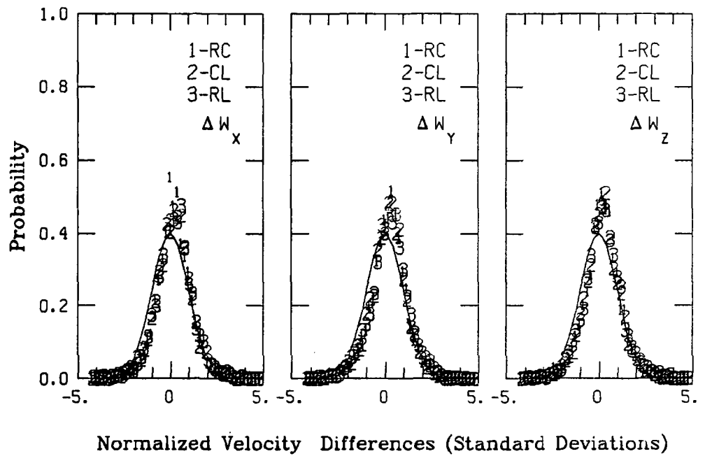
Figure A.283. Probability density function for gust velocities and gust velocity differences, Flight 6, Run 38.
