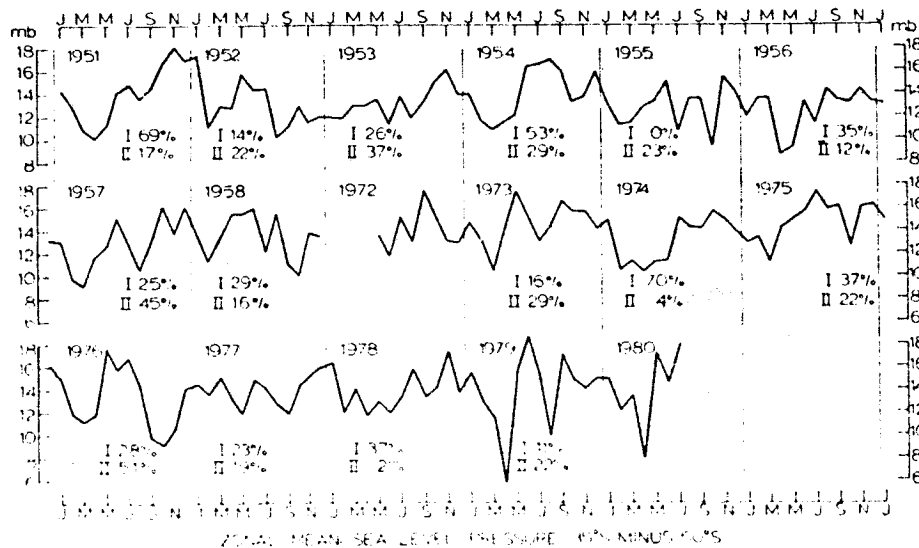
FIGURE 16 Differences in zonally averaged sea level pressure. I. The percentage of the annual variance explained by the yearly wave in the pressure difference. II. The percentage explained by the half-yearly wave. (a) 50°S minus 70°S. (b) 35°S minus 50°S.
