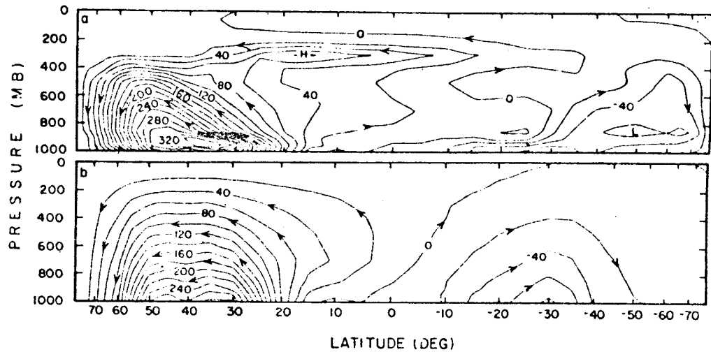
FIGURE 6 (a) Streamfunction ( \psi^* ) for the eddy induced residual mean meridional circulation. Winter is at positive latitudes; summer is at negative latitudes. Units are \text{m mb s}^{-1} ( \text{m mb s}^{-1} is equivalent to 0.41 \times 10^{12} \text{ g s}^{-1} mass flow). Data source: Oort and Rasmusson (1971). (b) Component of \psi^* induced by the poleward eddy flux of heat at the lower boundary.
