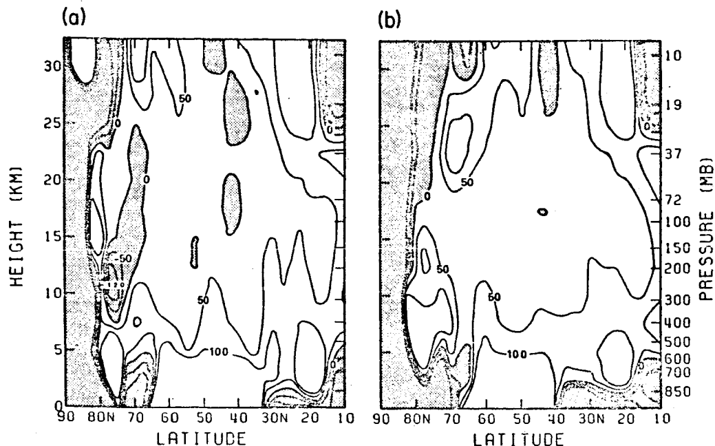
FIGURE 7 Refractive index squared Q_2 averaged over the period 0000 GMT February 23 to 0000 GMT February 25 with (a) the low-resolution version, and (b) the high-resolution version. Values larger than 100 or smaller than -100 are not contoured.
