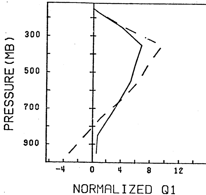
FIGURE 6 Apparent heat source for the 9,6 grid point in the full physics integration at hours 2 (solid) and 5 (dashed).
