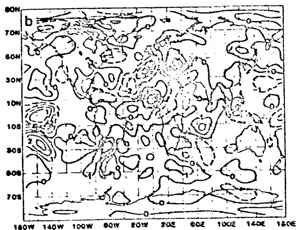
FIGURE 8 Time change (February minus January) of components of the 200 mb wind field from Paegle and Baker (1982). (a) Rotational zonal component, (b) Divergent meridional component.
