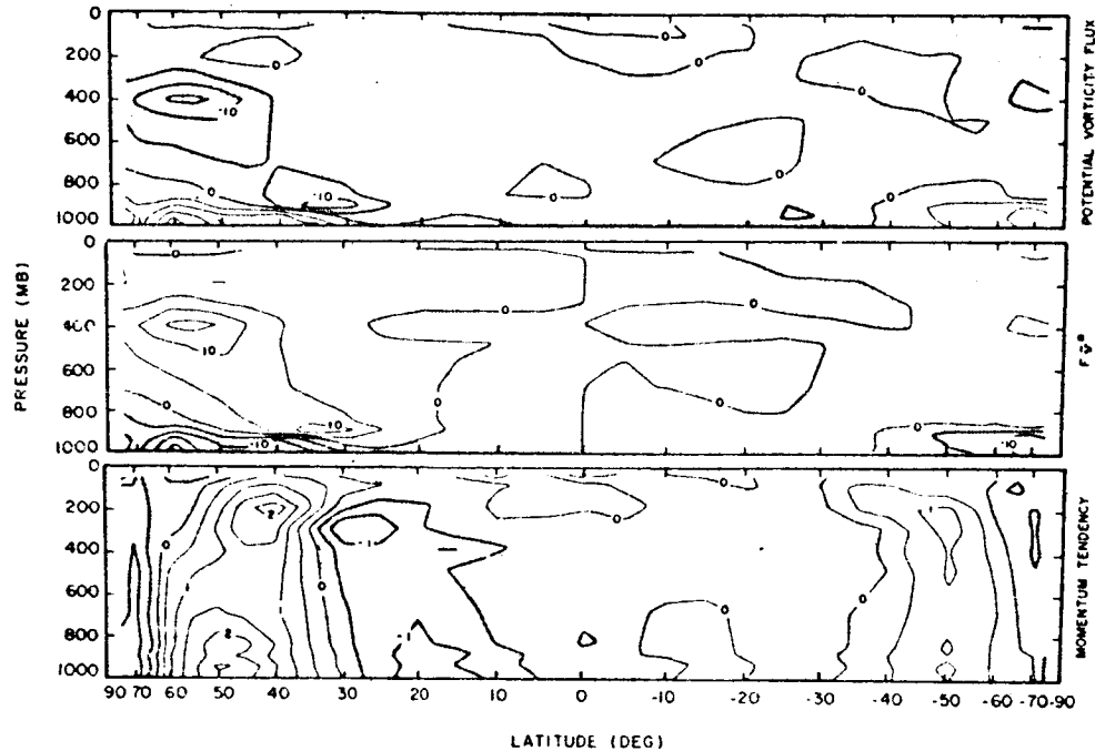
FIGURE 5 Winter (positive latitudes) and summer (negative latitudes) momentum budget due to eddy forcing using the transformed formalism of Andrews and McIntyre (1976). Units are 10^{-5} \text{ m s}^{-2} . The peak value of the momentum tendency in winter represents an acceleration of 2 \text{ m/s day}^{-1} . (Data source: Oort and Rasmusson, 1971.)
