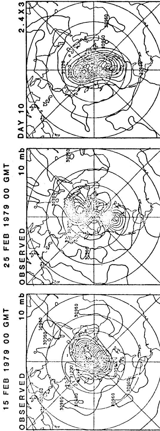
FIGURE 8 As in Figure 4, except for the forecast from February 15.
