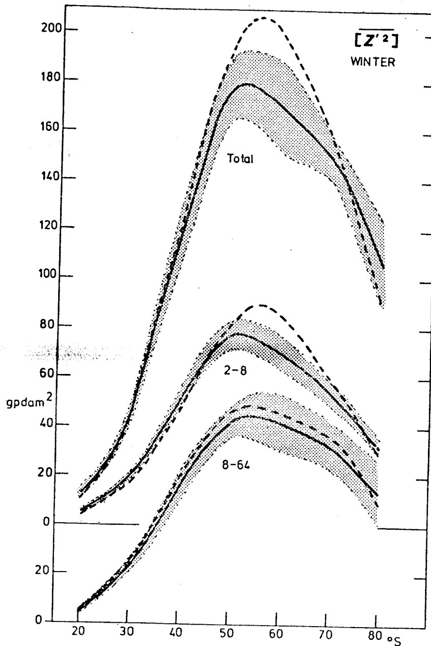
FIGURE 8 Meridional profile of the variance of geopotential height for winter, g p \text{ dam}^2 ; mean (solid curve), plus and minus one standard deviation (shaded), and the profile for GWE (dashed). Shown are the total variance and the contributions from the 2-8 day and 8-64 day period bands. The scale of the latter is offset.
