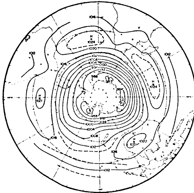
FIGURE 1 Mean sea level pressure in (a) January, (b) July (from van Loon and Rogers, 1984b).
