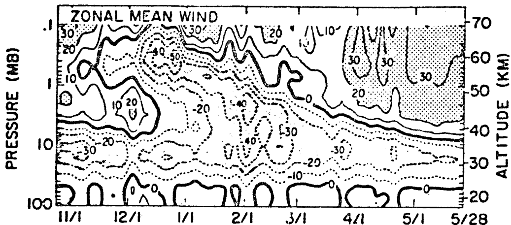
FIGURE 3 Zonally averaged zonal winds averaged over the latitude band 8^{\circ}\text{S} to 8^{\circ}\text{N} versus time and pressure level for the period October 25, 1978 to May 28, 1979.
