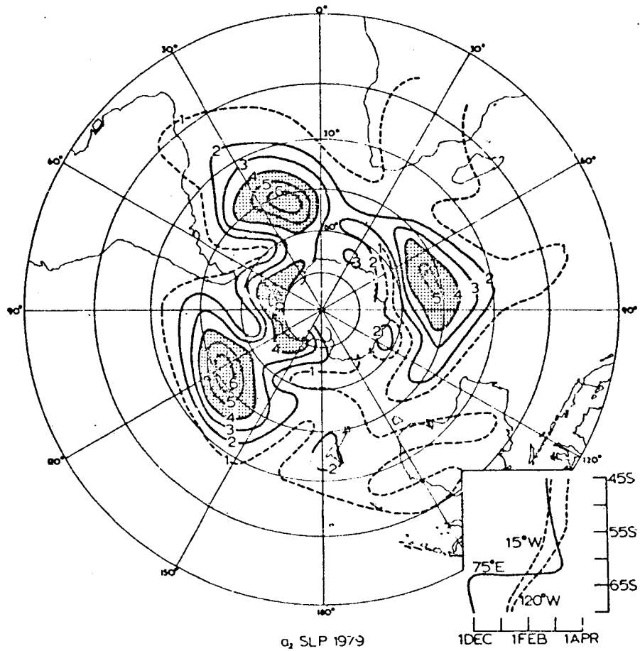
FIGURE 7 Amplitude (mb) of the half-yearly wave in sea level pressure in 1979. Inset shows phase at three longitudes (date of first maximum) (from van Loon and Rogers (1984a)).
