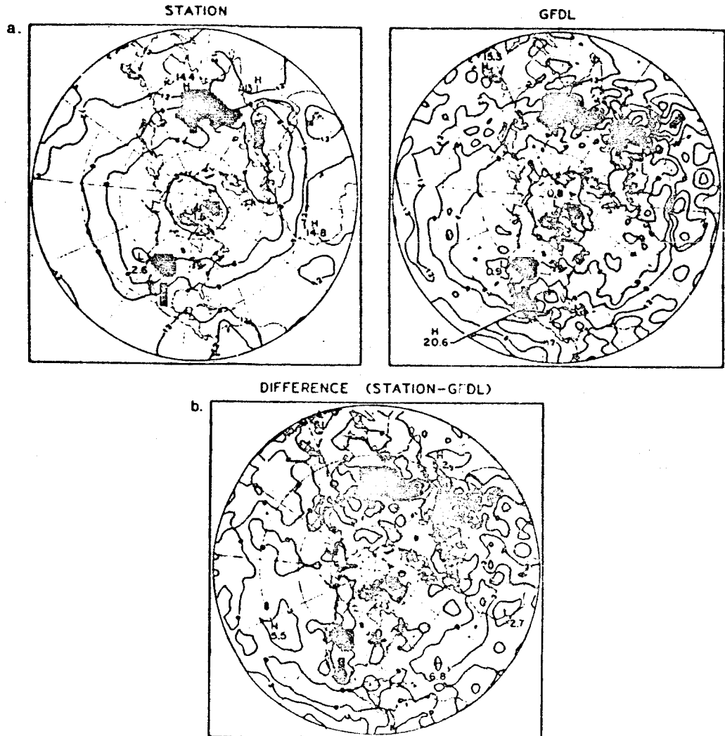
FIGURE 14 (a) Hemispheric maps of the specific humidity at 850 mb for June 1979 based on the station and the GFDL level IIIb analyses. Isolines are drawn at intervals of 3 \text{ g kg}^{-1} . Regions where the topography is at pressures less than 850 mb are indicated by the heavy shading. (b) Difference, station analysis minus GFDL analysis, of the two fields in a. Isolines are drawn at intervals of 3 \text{ g kg}^{-1} . Negative values are shaded and indicate higher values of specific humidity in the GFDL analysis.
