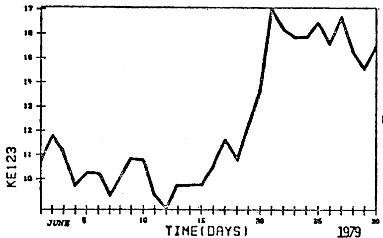
FIGURE 5 Time series from June 1 to 30, 1979 of planetary scale (sum of wavenumbers 1 to 3) energetics: (a) APE, and (b) KE.
