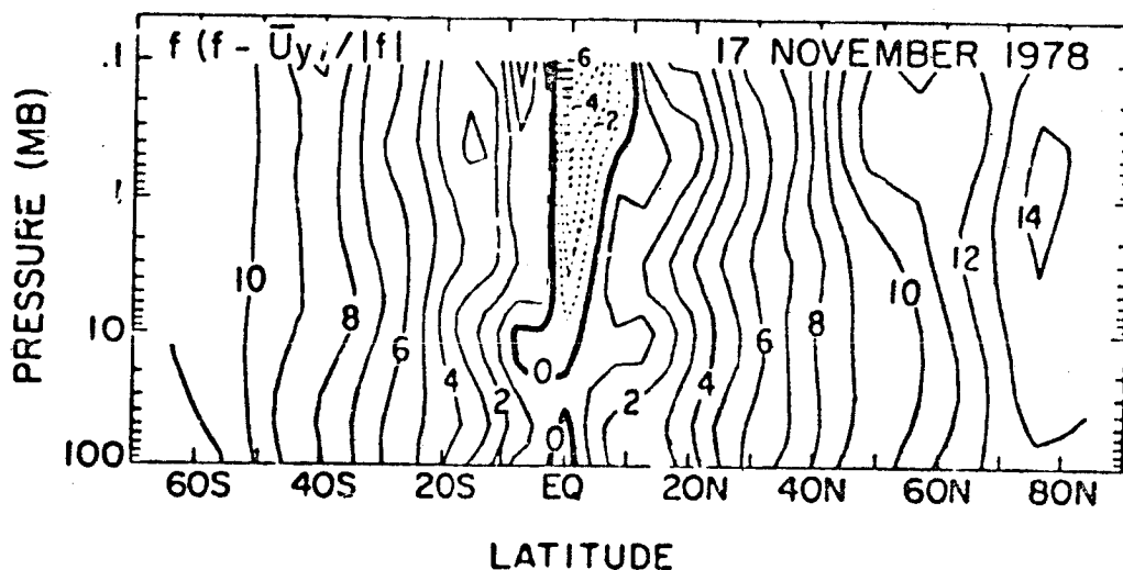
FIGURE 7 Inertial stability parameter expressed in terms of the coriolis parameter f and mean zonal wind shear u_y . The region of negative values is inertially unstable (units: 10^{-5} s^{-1} ).
