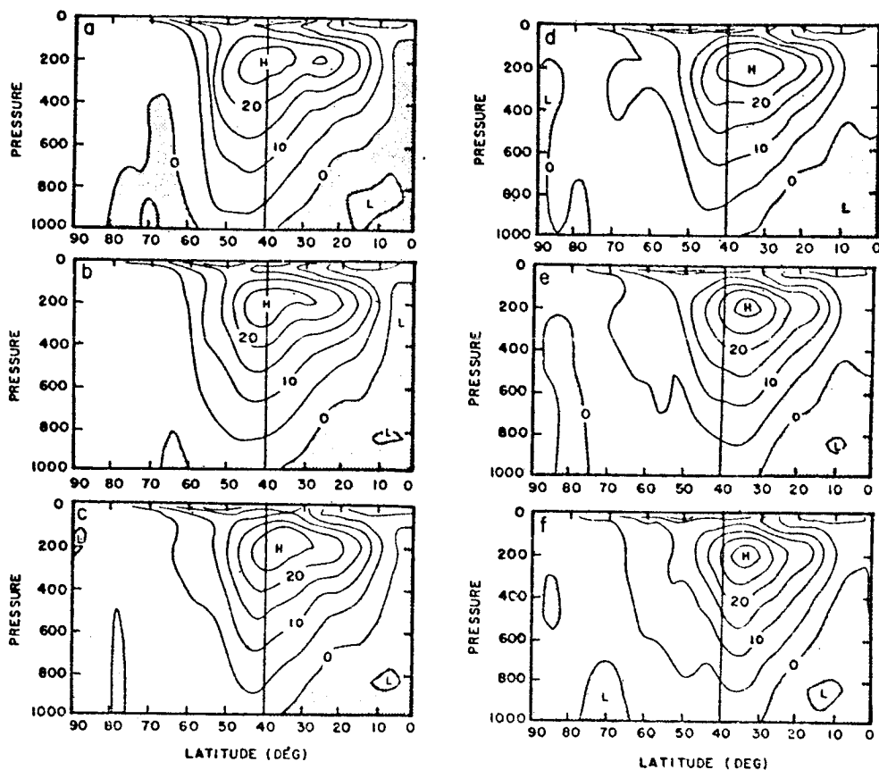
FIGURE 8. Sequence of distributions of u \cos in the meridional plane from December 15 through December 20, 1972 (Figure 8a to Figure 8f). The vertical line at 40^{\circ}\text{N} is for reference. Units are m/s. (Data source: ECMWF FGGE IIIb.)
