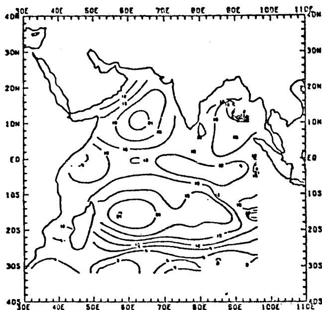
FIGURE 9 Mean flux of moist static energy from the sea into the air for July 1979. Units 10 \text{ W/m}^2 (Wylie and Hinton, manuscript in preparation).
