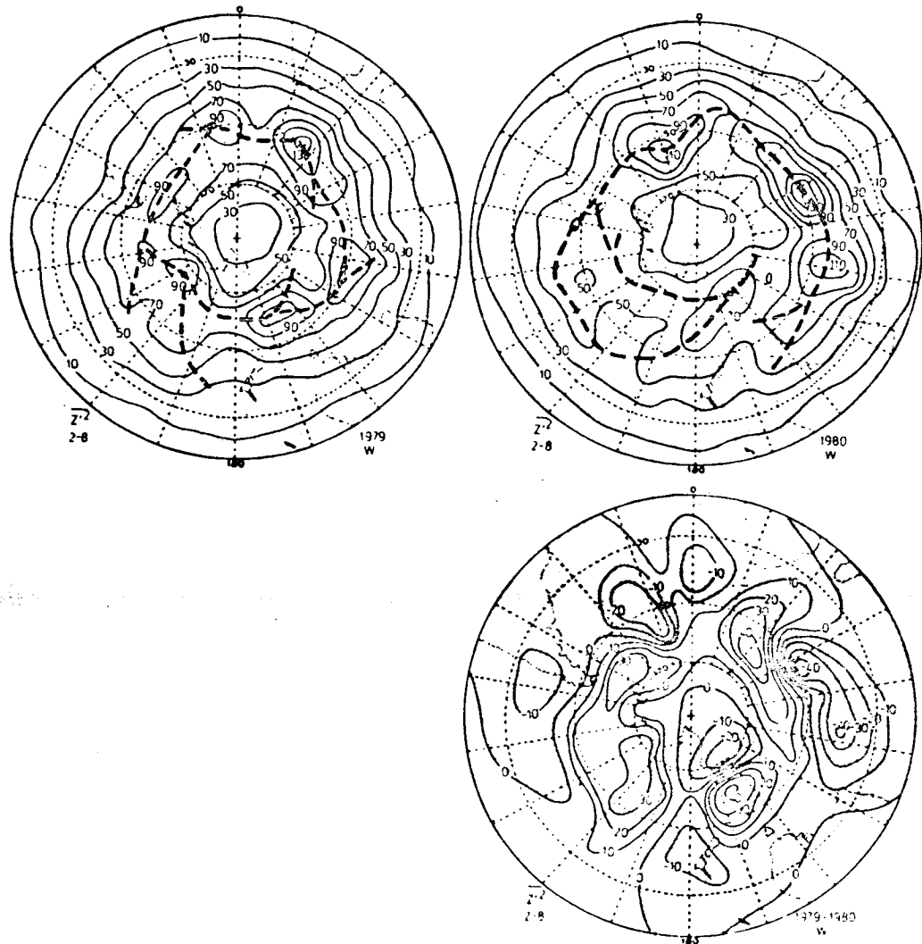
FIGURE 12 The 2-8 day period band contribution to the variance of geopotential height \bar{z}^2 (a) winter 1979, (b) winter 1980, and (c) their difference 1979-1980; in g p \text{ dam}^2 . The heavy dashed lines denote the locus of the maxima and thus the main storm tracks.
