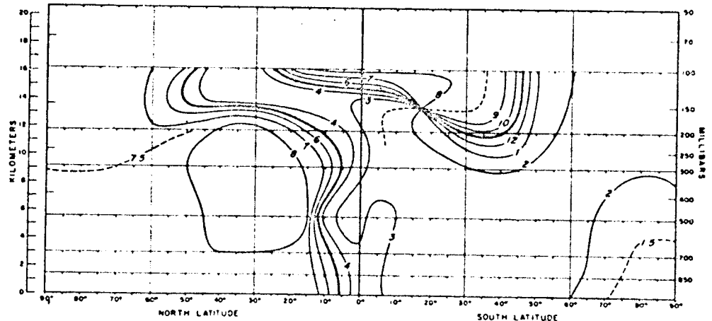
TEMPERATURE - 1ST HARMONIC - PHASE (MONTH)
