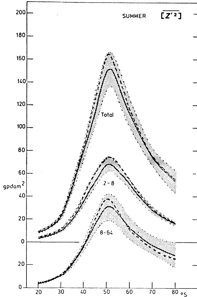
FIGURE 9 Meridional profile of the variance of geopotential height for summer, g p \text{ dam}^2 ; mean (solid curve), plus and minus one standard deviation (shaded), and the profile for GWE (dashed). Shown are the total variance and the contributions from the 2-8 day and 8-64 day period bands. The scale of the latter is offset.
