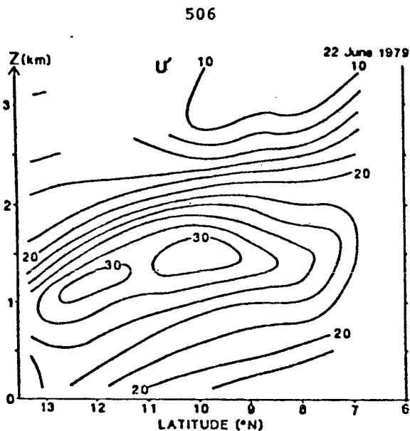
FIGURE 11 Somali jet wind structure from June 22, 1979 aircraft penetration (m/s) (Nordgarden and Young, 1984).
