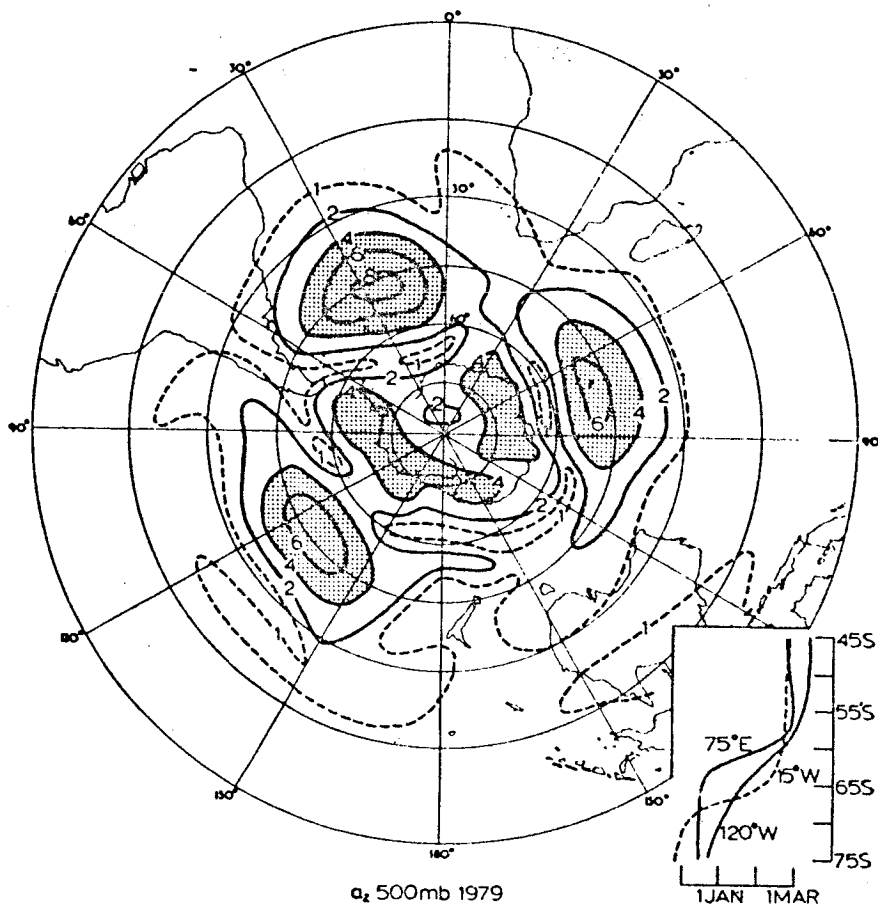
FIGURE 19 Amplitude (dkm) of the half-yearly wave in the 500 mb height of 1979. Inset shows the phase (date of first maximum) at three meridians (van Loon and Rogers, 1981b).
