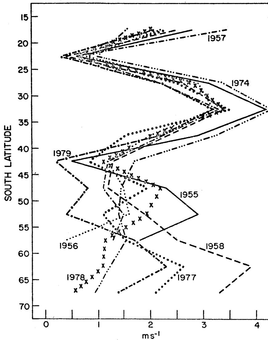
FIGURE 11 Meridional vertical section of the amplitude ( \text{m/s} ) of the yearly wave in the zonally averaged geostrophic wind at sea level in eight single years (van Loon and Rogers, 1984b).
