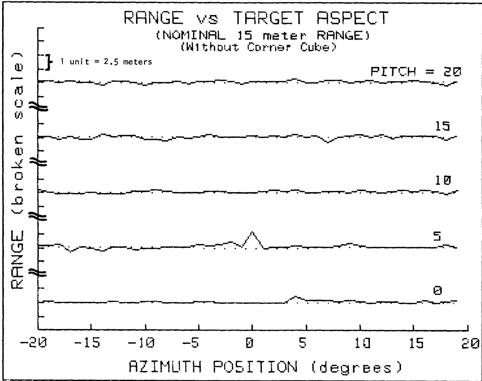
Figure 13. Range vs. Target Aspect (Nominal Range of 15 meters; WITHOUT Corner Reflector).
