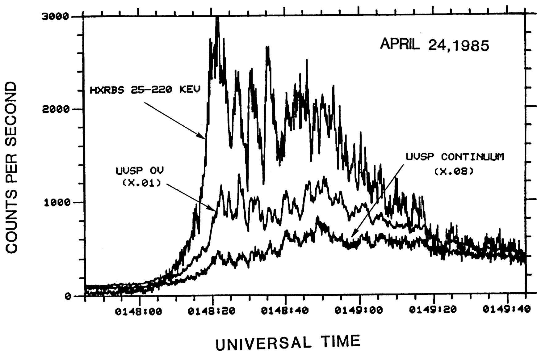
Figure 10. UVSP and HXRBS time profiles for the flare on 24 April 1985 at 01:48 UT. The top profile is the hard X-ray counting rate between 25 and 220 keV, the center profile is the counting rate in the O V line, and the bottom profile is the counting rate in the continuum 17 Å from the O V line. The time resolution for all three profiles is 128 ms.
