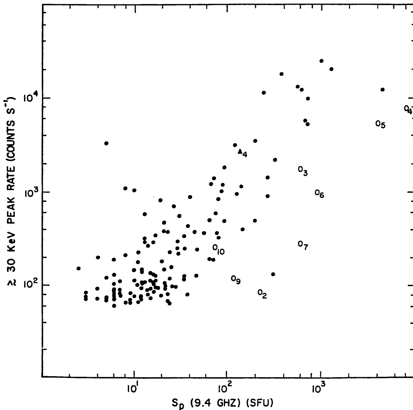
Figure 16. Scatter plot of HXRBS > 30 keV peak hard X-ray count-rate versus the peak 9.4 GHz flux-density for impulsive ( \Delta ) and gradual ( \circ ) components of the GHBs analyzed by Cliver et al. (1985). For comparison, the data points for \sim 130 impulsive events observed both by SMM and Toyokawa Observatory during April, August, and December 1981 are also plotted ( \bullet ). For the comparison sample, we considered events to be impulsive if the 9.4 GHz emission peak occurred within \pm 0.5 min of the HXRBS > 30 keV maximum. The \sim 40 counts s^{-1} HXRBS background counting rate was not subtracted from the > 30 keV peak rates.
