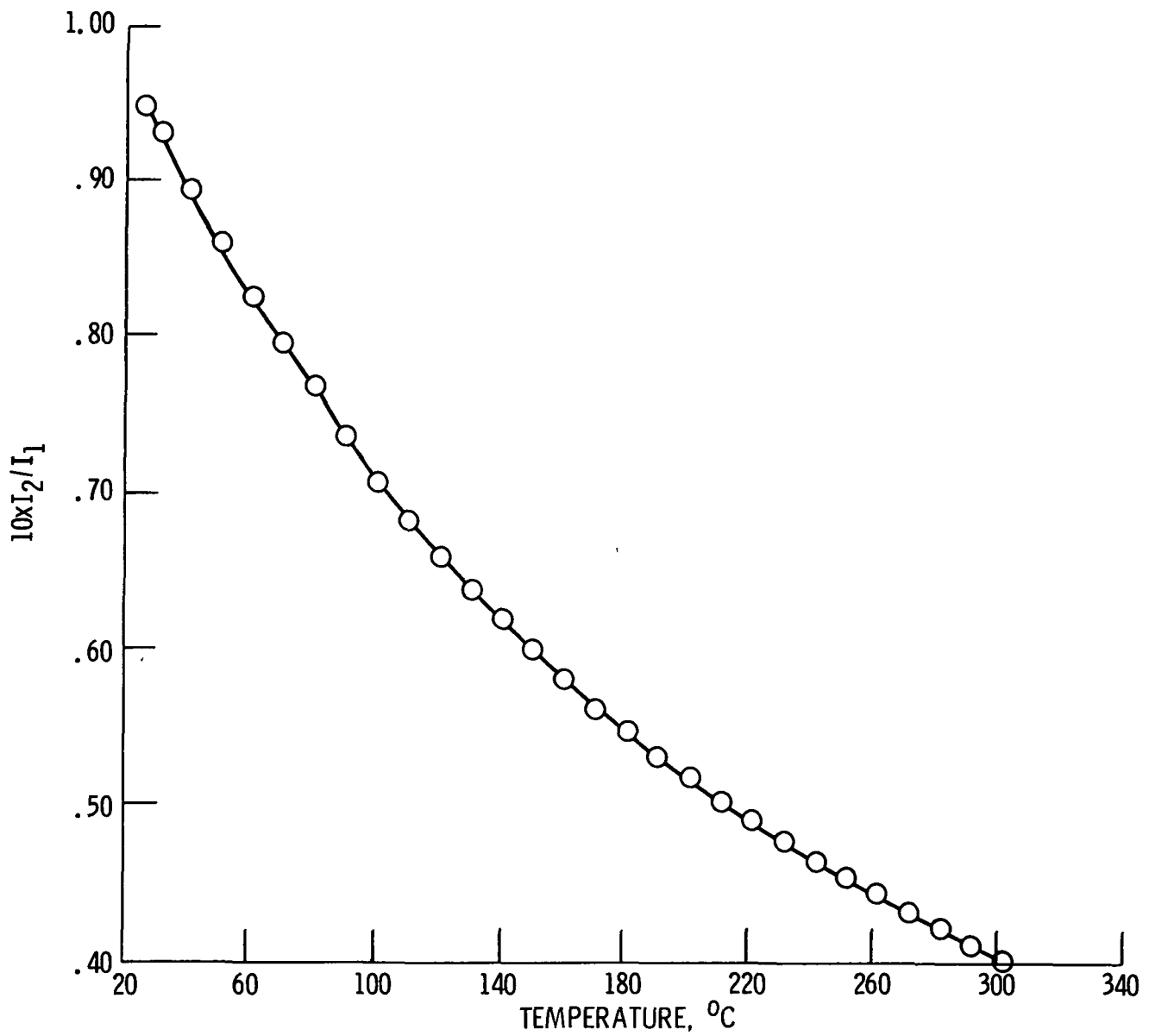
Figure 3. - Experimentally obtained power ratio I_2/I_1 as a function of temperature using Nd^{+3} doped glass as a temperature sensor.
