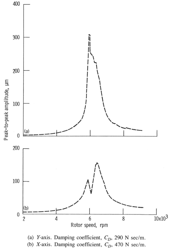
Figure 10.—Experimental damped response for damper design B. Unbalance, 10.8 g cm.
