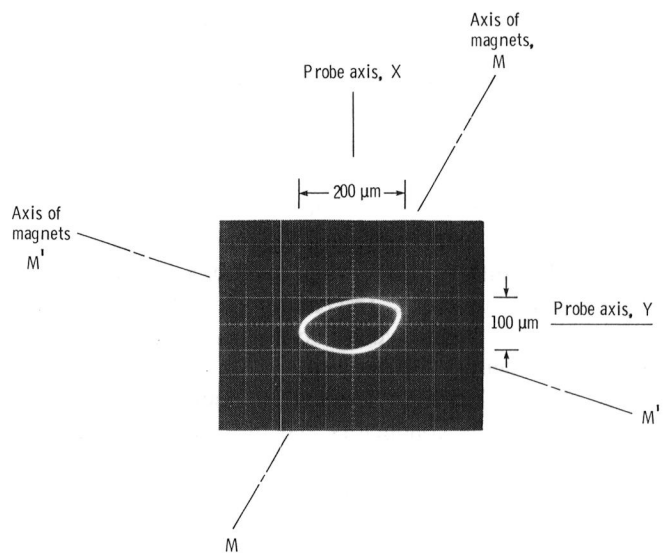
Figure 11.—Damped orbital motion of rotor near resonant frequency of 6000 rpm. Magnet design B; scale factor, V/cm; calibration factor, 78.7 V/cm (200 V/in.).
