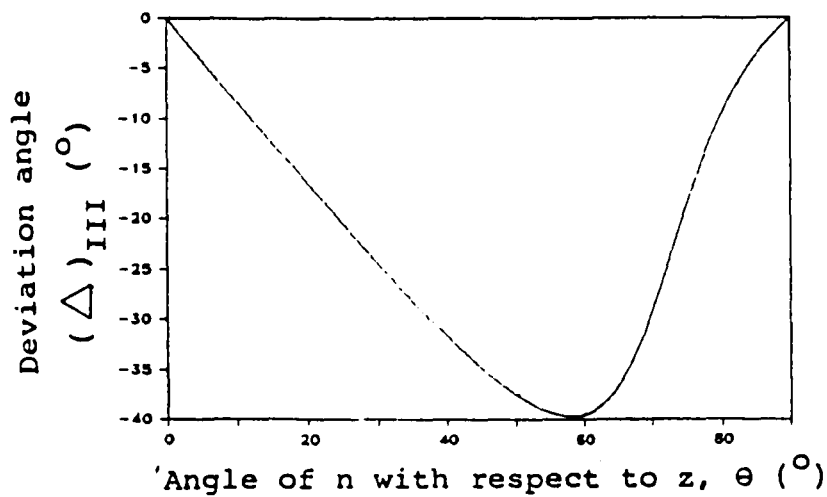
Fig.5 Deviation angles (\Delta)_{I,II,III} between phase velocity and group velocity directions for phase velocities V(SH), V(SV) and V(P).
