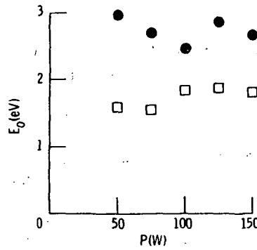
Figure 4. - Optical energy gap E_0 versus deposition power P for plasma deposited \alpha -C:H on quartz using CH_4 ( \square ) and C_4H_{10} ( \bullet ). The chamber pressure is 170 m Torr.
