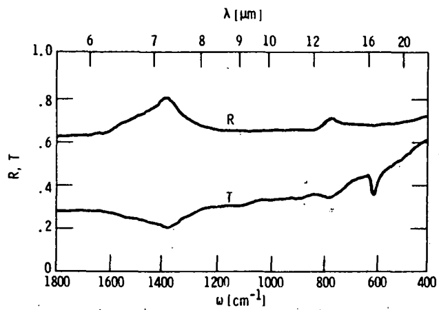
Figure 7. - Reflection R and transmission T versus wavenumber \omega for ion beam deposited BN film on Si. Deposition temperature 200 °C, ion beam energy 150 eV.
