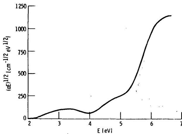
Figure 8. - Tauc plot (\alpha E)^{1/2} versus E for ion beam deposited BN film on quartz, Deposition temperature 200 °C; ion beam energy 150 eV.
