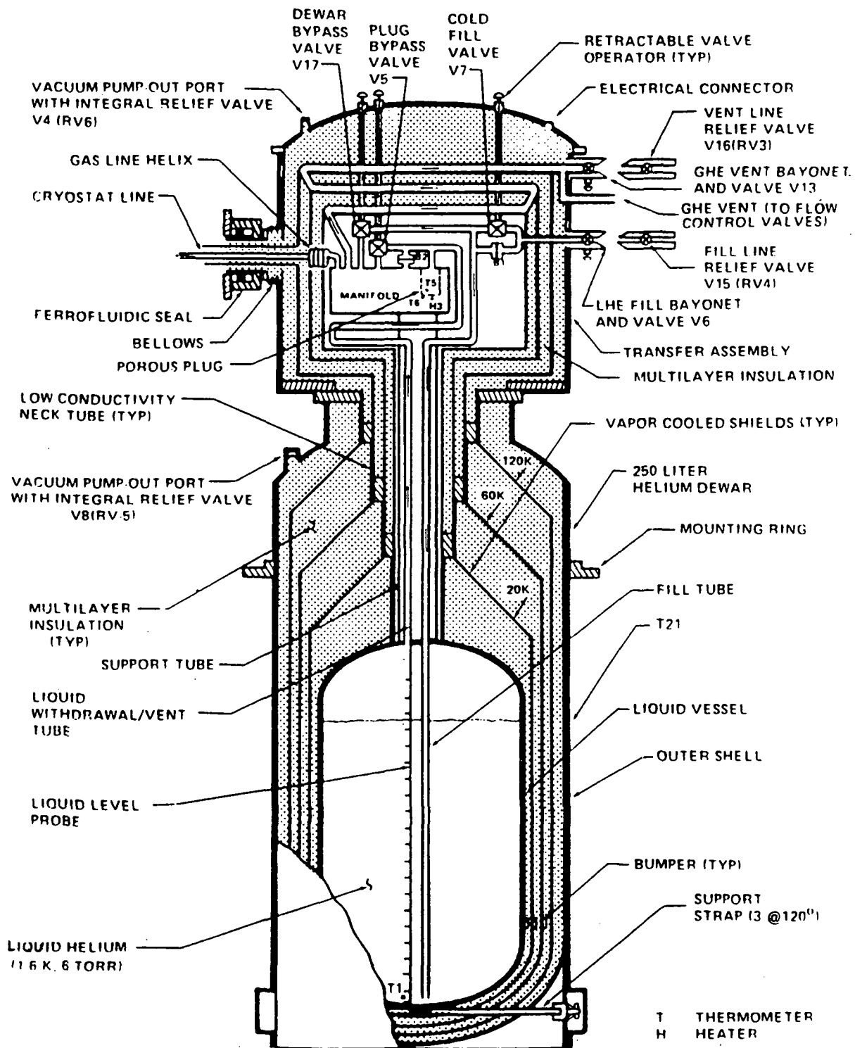
Figure 1. Schematic of IRT dewar subsystem, TPEs I-V.
