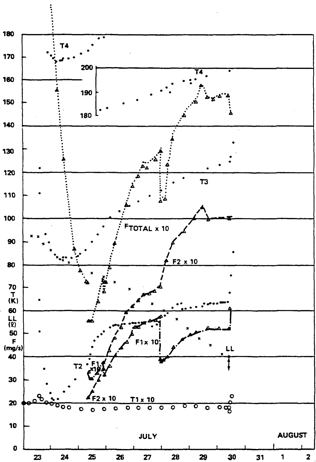
Figure 37. Graphical summary, TPE VI, second phase.
