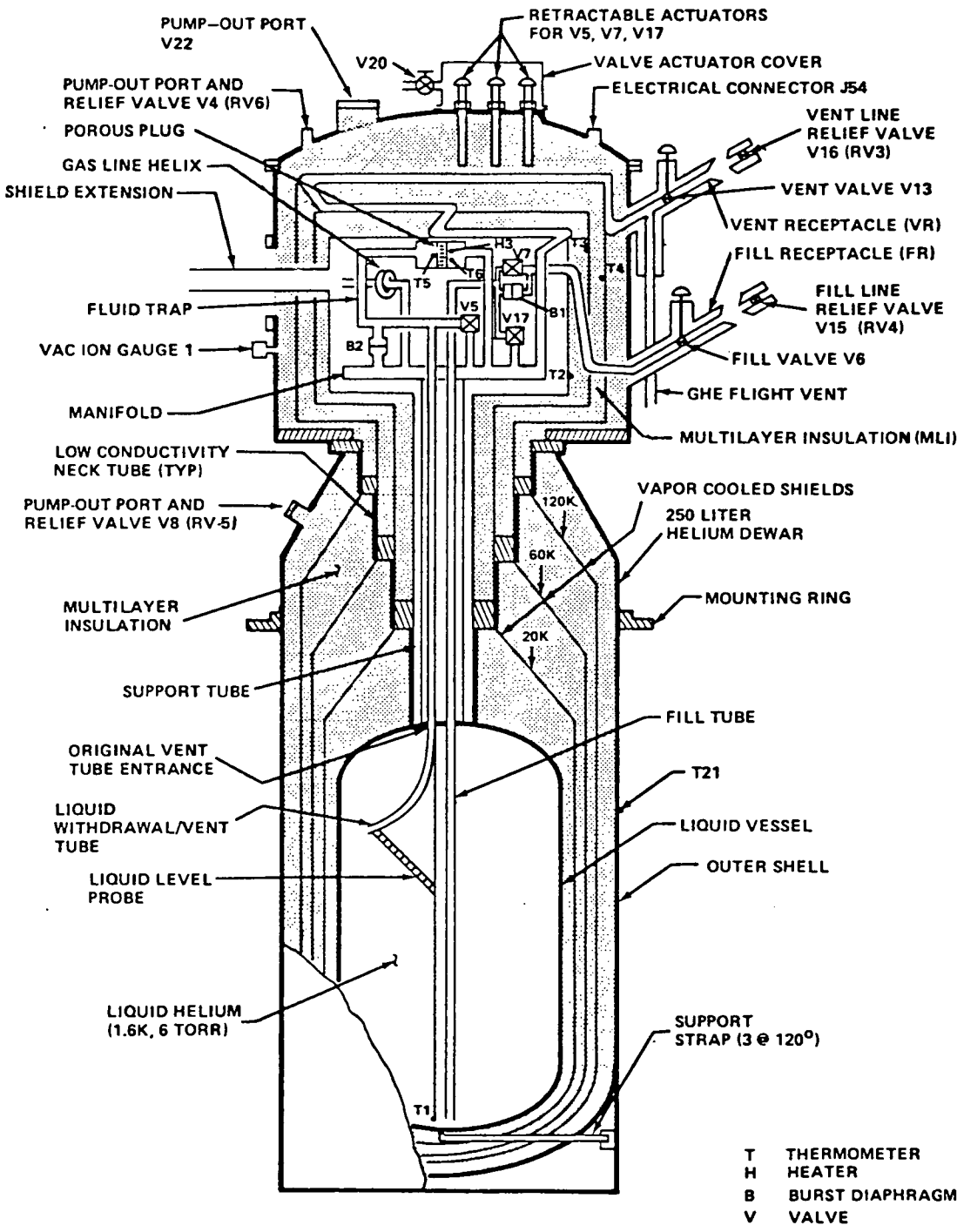
Figure 34. Schematic of IRT dewar subsystem, TPEs VI-VII.
