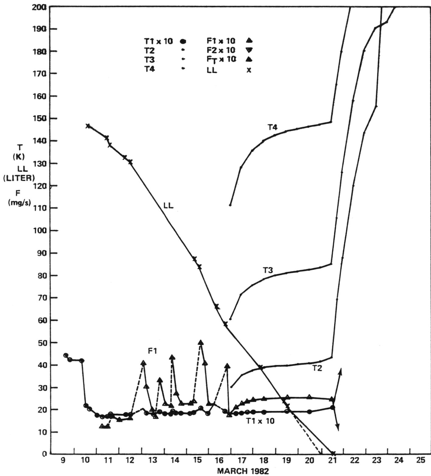
Figure 17. Graphical summary of TPE V.
