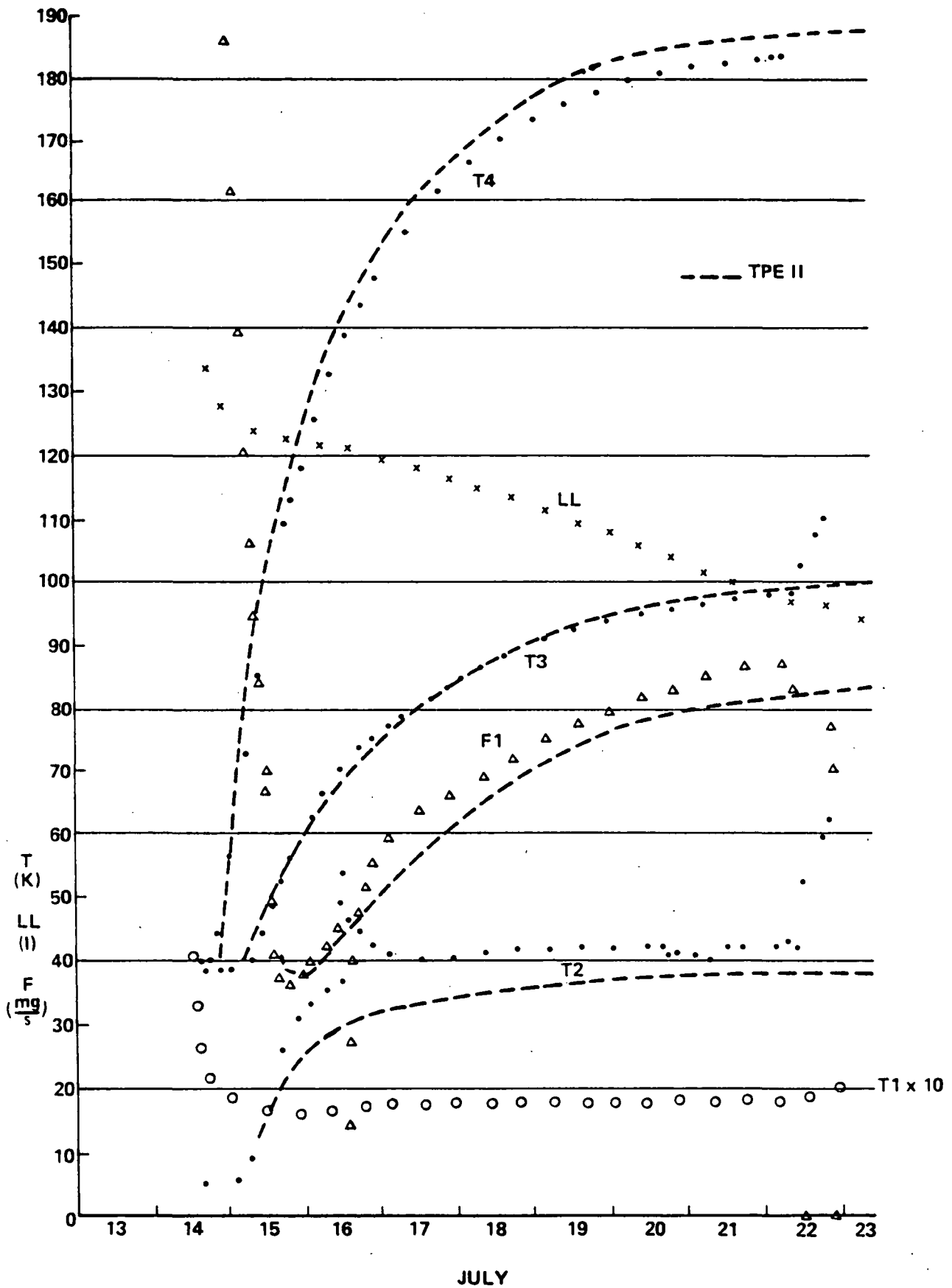
Figure 36. Graphical summary, TPE VI, first phase.
