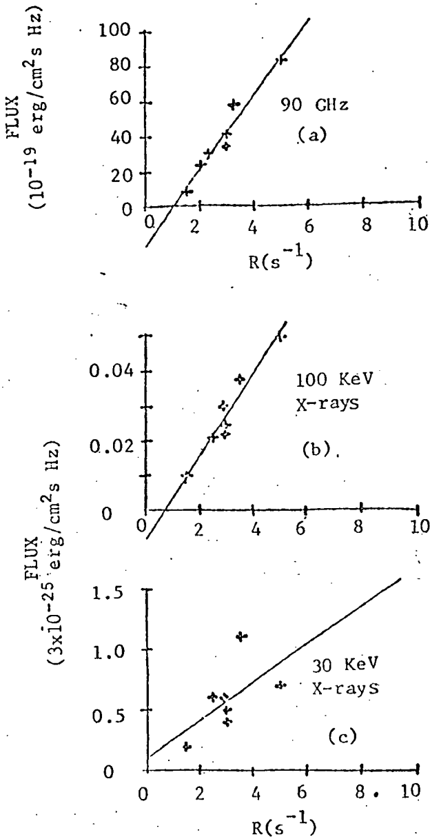
Figure 6 - Scatter diagrams: (a) Pulse repetition rates and fluxes at 90 GHz, (b) repetition rates at 90 GHz and fluxes at hard X-rays ( > 100 KeV), and (c) repetition rates at 90 GHz and fluxes at hard X-rays ( > 30 KeV), for all the seven structures.
