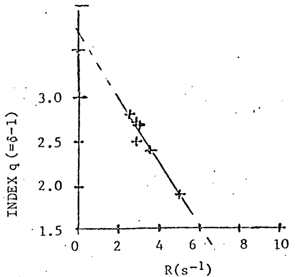
Figure 7 - Scatter diagram between pulse repetition rates and X-ray spectral index, for the last six burst structures.
