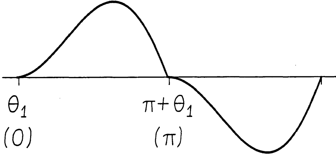
Figure 31: Inductor current waveform for the resonant input filter in continuous conduction mode.
