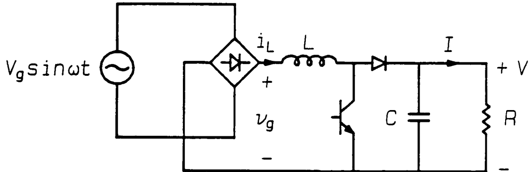
Figure 10: Boost topology.
