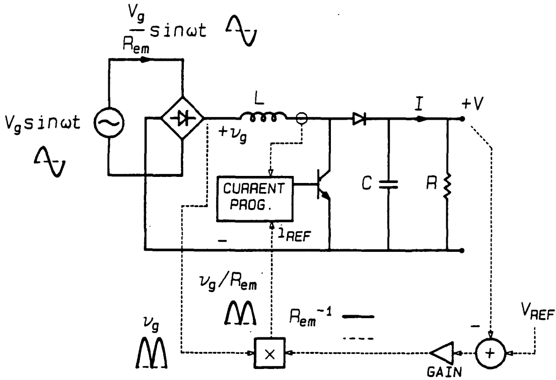
Figure 12: Control of the boost resistor emulator.
