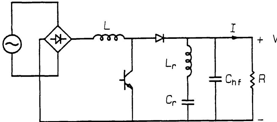
Figure 23: Resonant filter in a boost current shaper.
