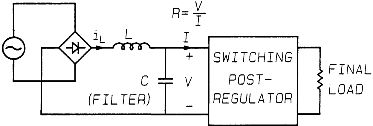
Figure 3: Inductor input filter followed by a voltage post-regulator.
