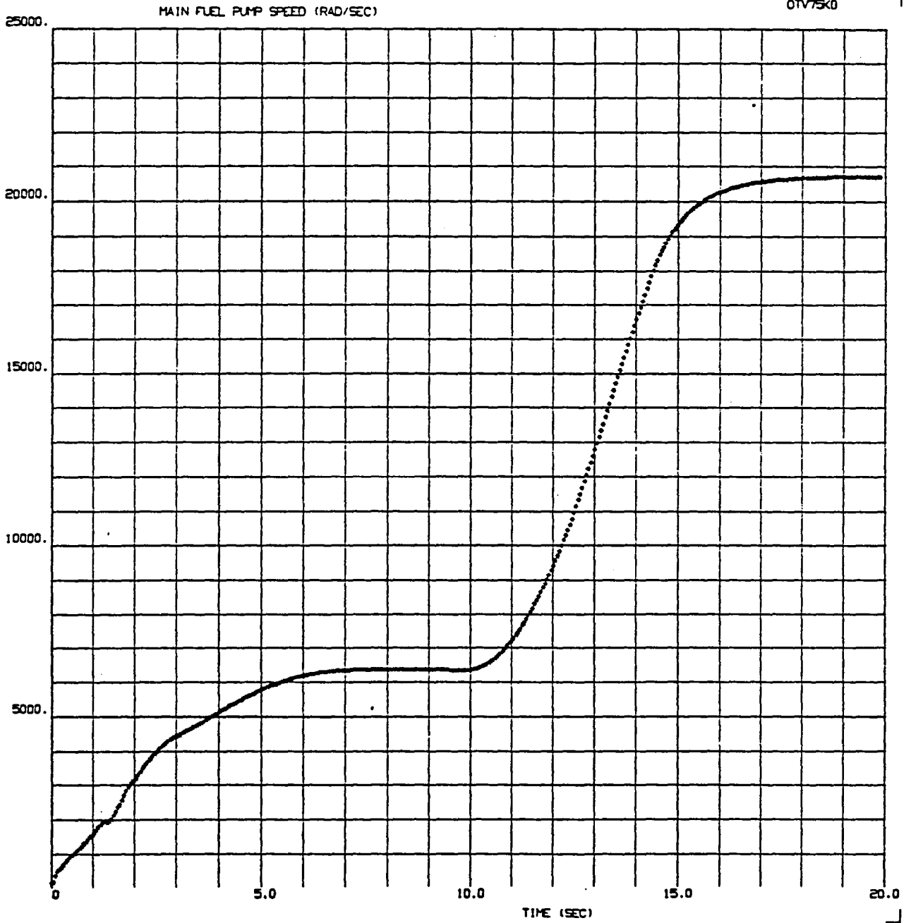
Figure 6-5 Main Fuel Pump Speed - 7.5K Engine Start
