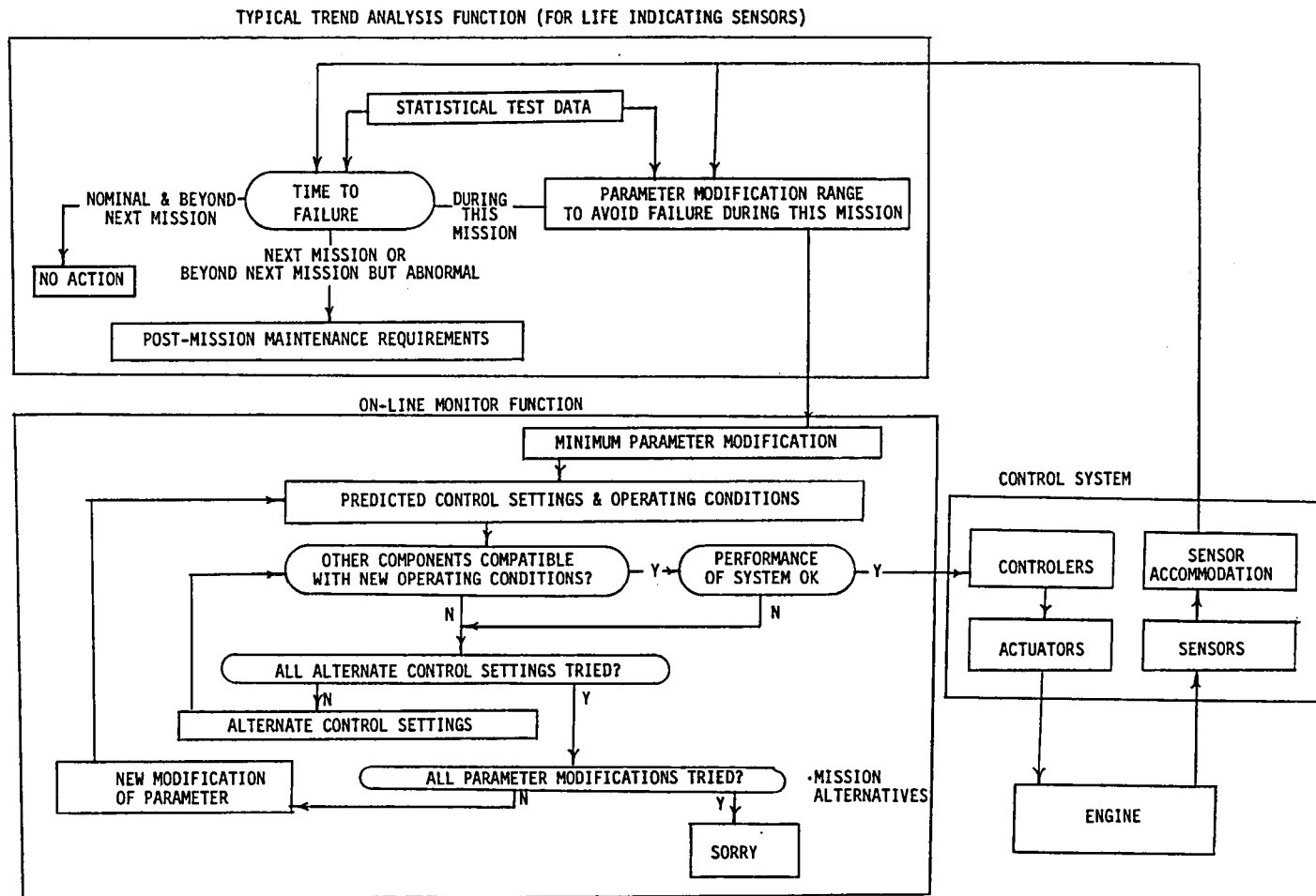
FIGURE 20. ICHM FUNCTION ALLOCATIONS AND LOGIC DIAGRAM
