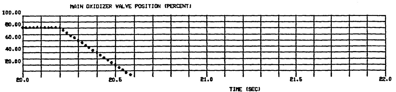
Figure 7-7 Valve Sequences - 7.5K Engine Shutdown with TSV Located Upstream of HPFT
