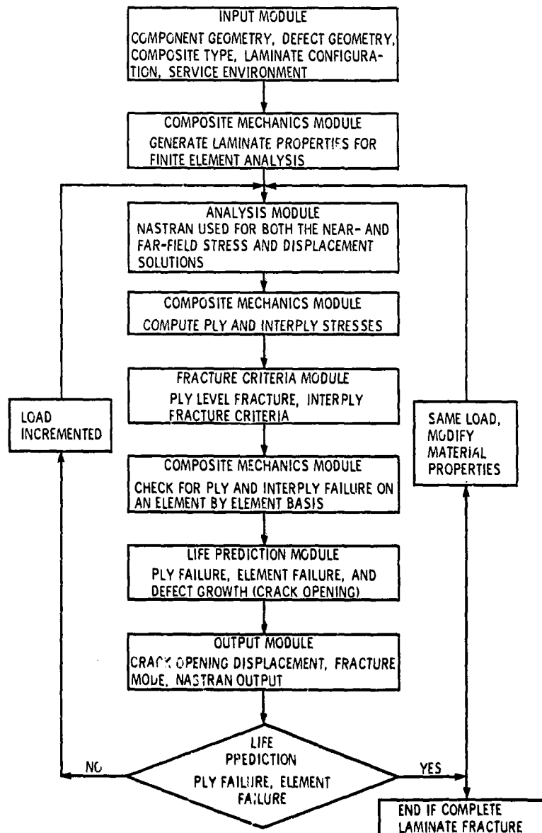
Figure 2. - CODSTRAN flow chart: computational simulation of progressive fracture.
