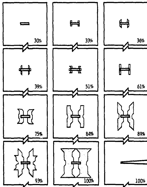
Figure 5. - Computationally simulated progressive fracture at various percentages of the fracture load (15 402 lb; Gr/EID+30/0/-30/0)_2 ).
