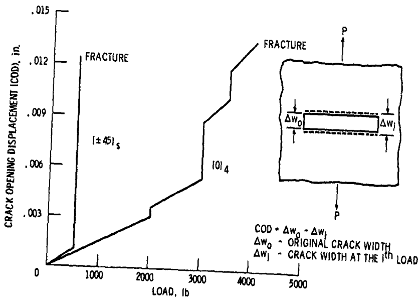
Figure 7. - Computationally simulated laminate behavior to fracture ( G/E \approx 8 ).
