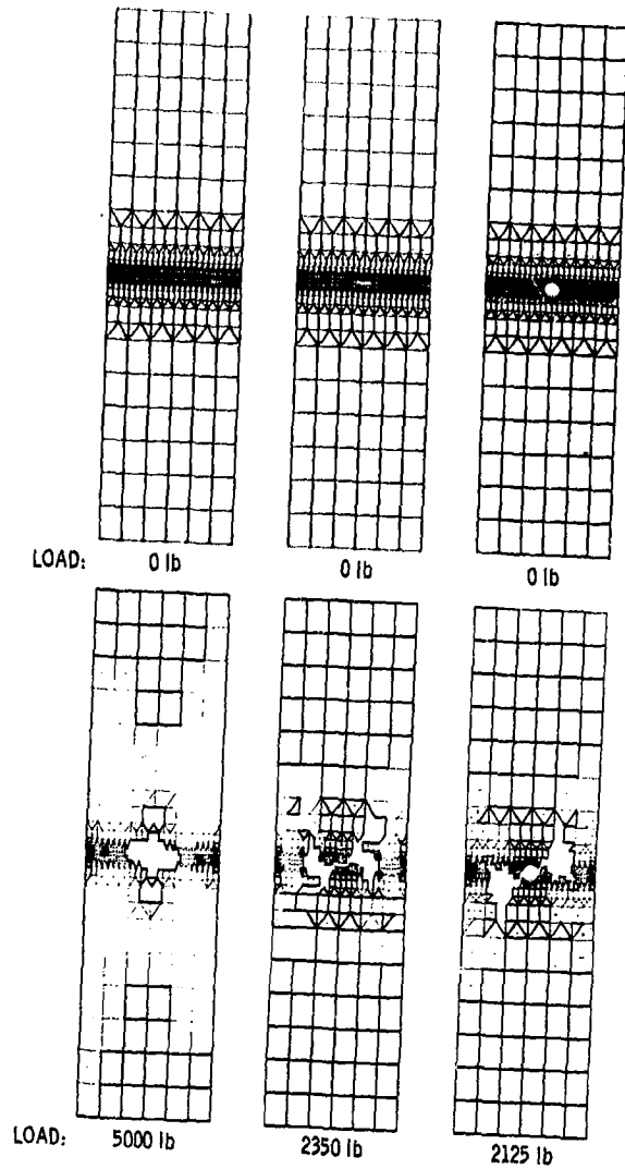
Figure 6. - Computationally simulated progressive fracture of laminates with different types of defects ( G/E \approx 2.5 ).
