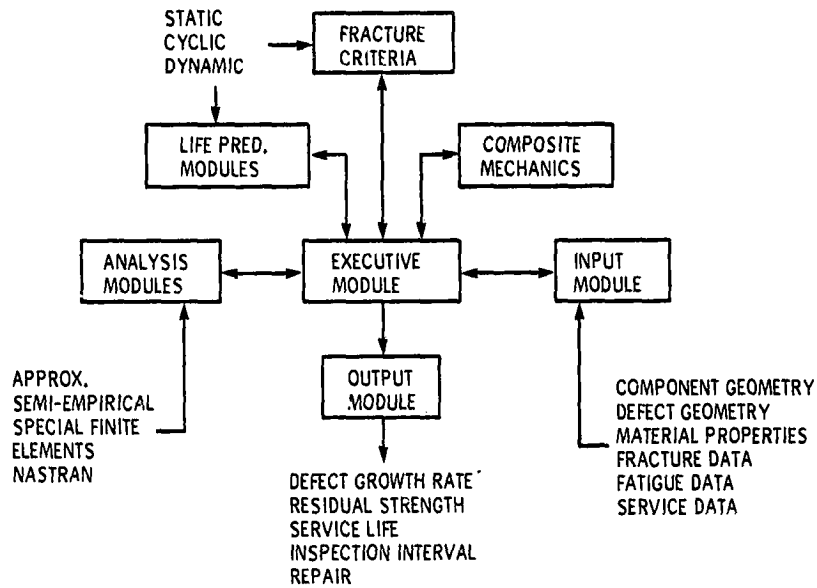
Figure 1. - CODSTRAN computer code schematic.
