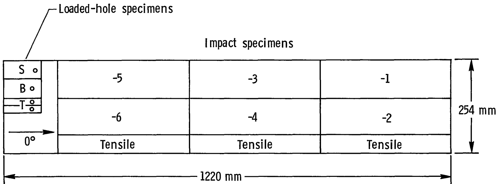
Figure 1 Composite panel layout 24 plies
