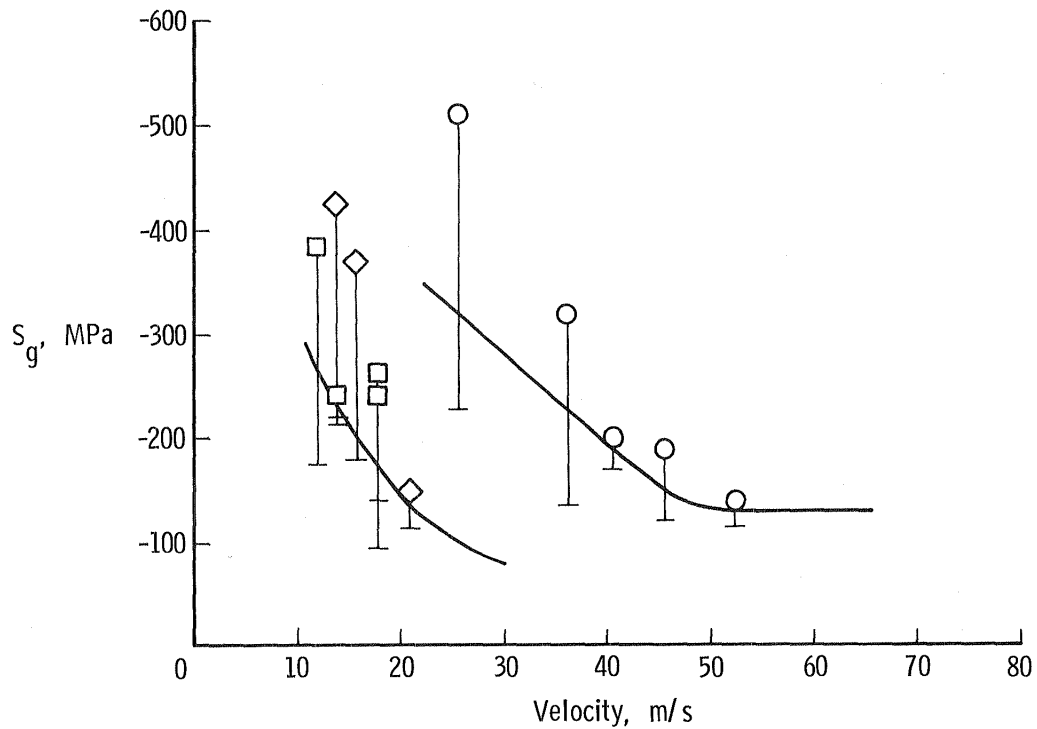
(b) Compression.
