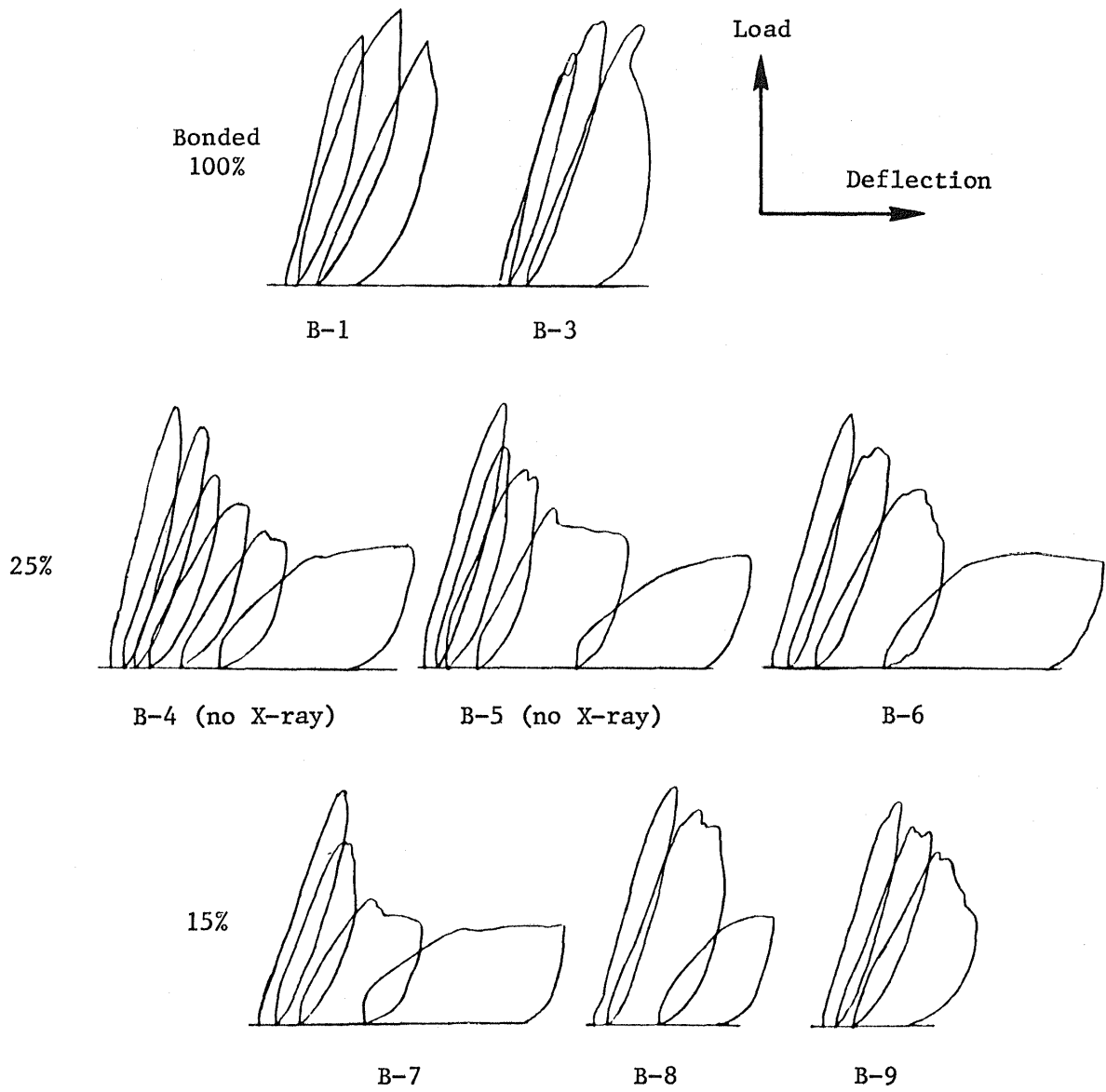
Figure 19. Traces of load-deflection curves for loaded-hole specimens.
