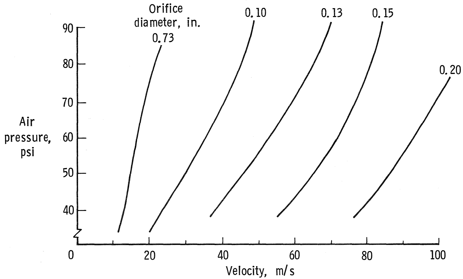
Figure 6. Calibration of air-driven impact gun.
