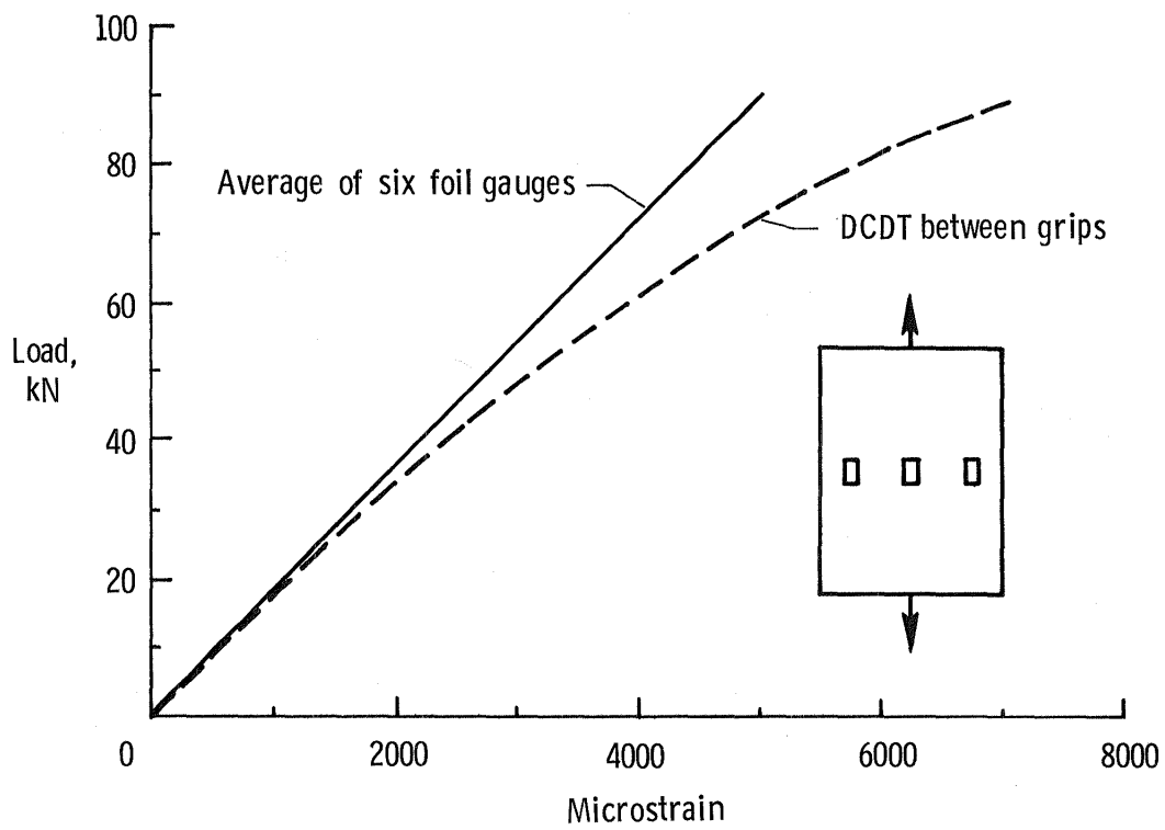
(a) Tension.
