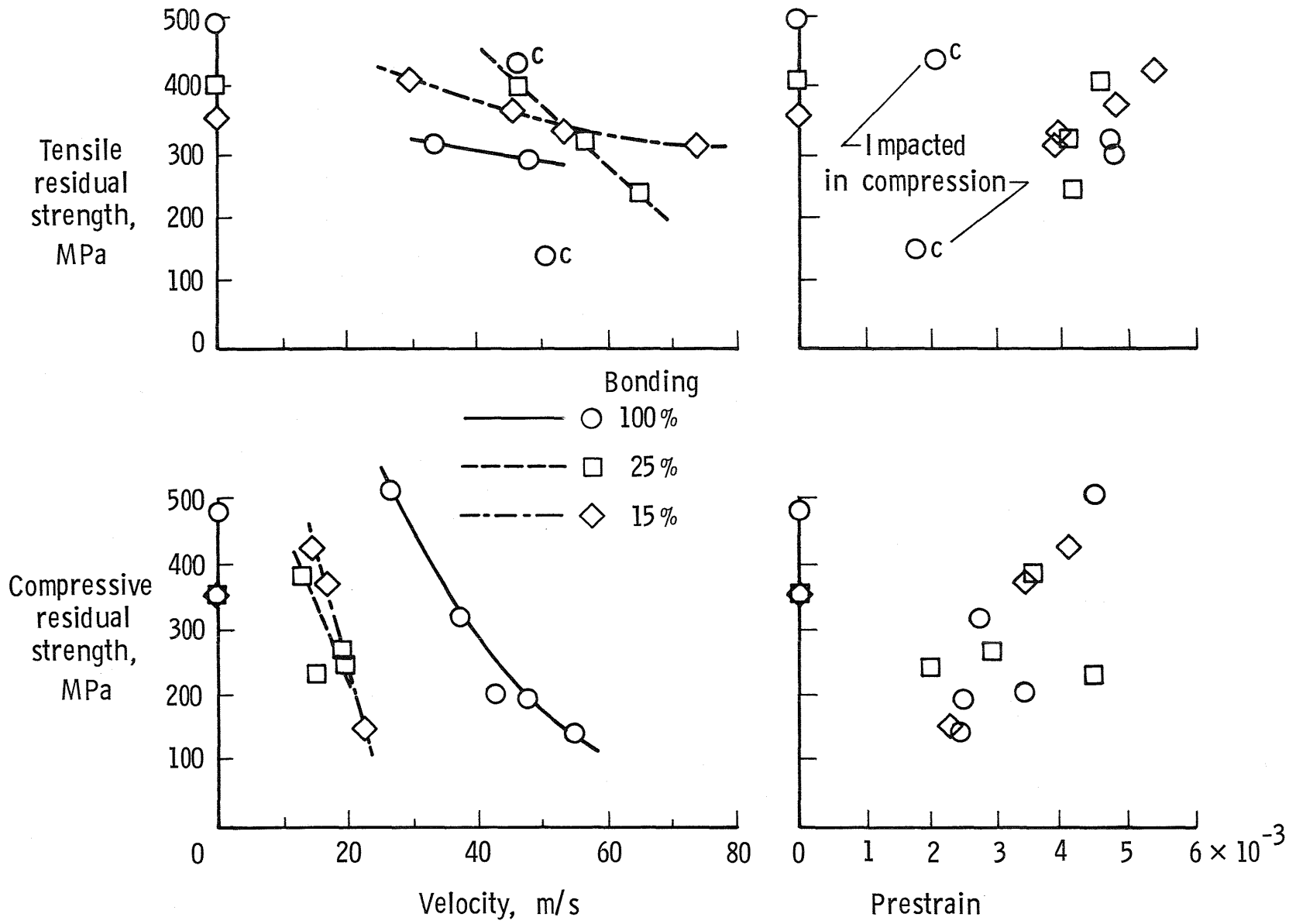
Figure 18. Correlations of residual strength with velocity and prestrain.
