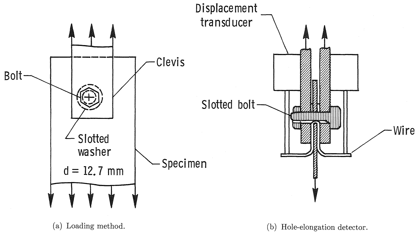
Figure 7. Test apparatus for loaded-hole specimens.
