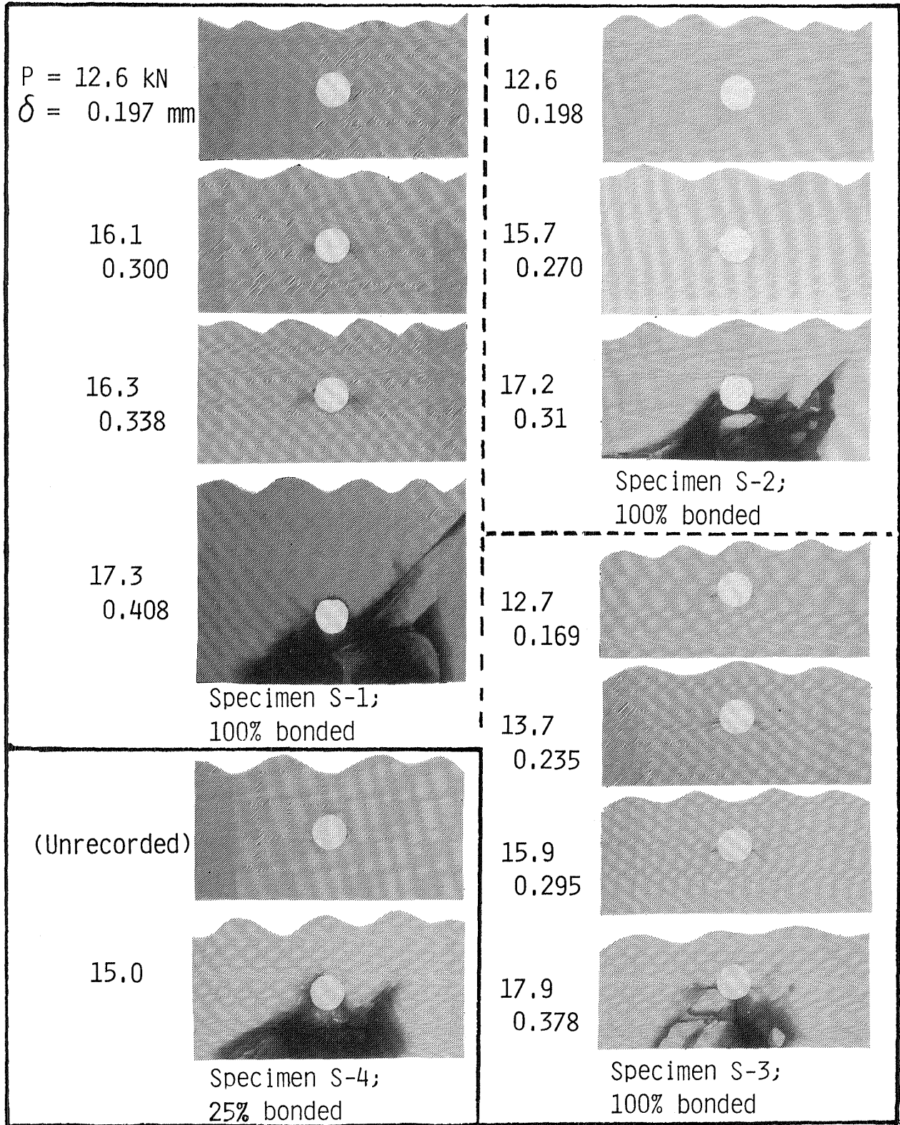
Figure 22. Radiographs of shear-critical specimens. Pin loaded toward bottom; zinc iodide was used as enhancer.
