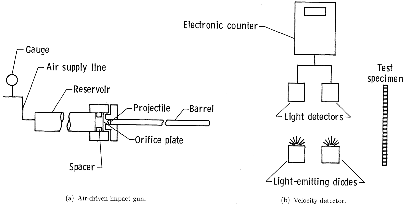
Figure 4. Schematic diagram of air-driven impact gun and velocity detector.
