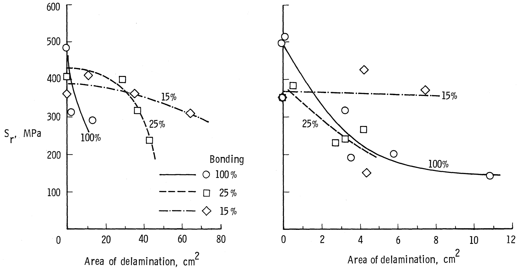
(a) Tension.
