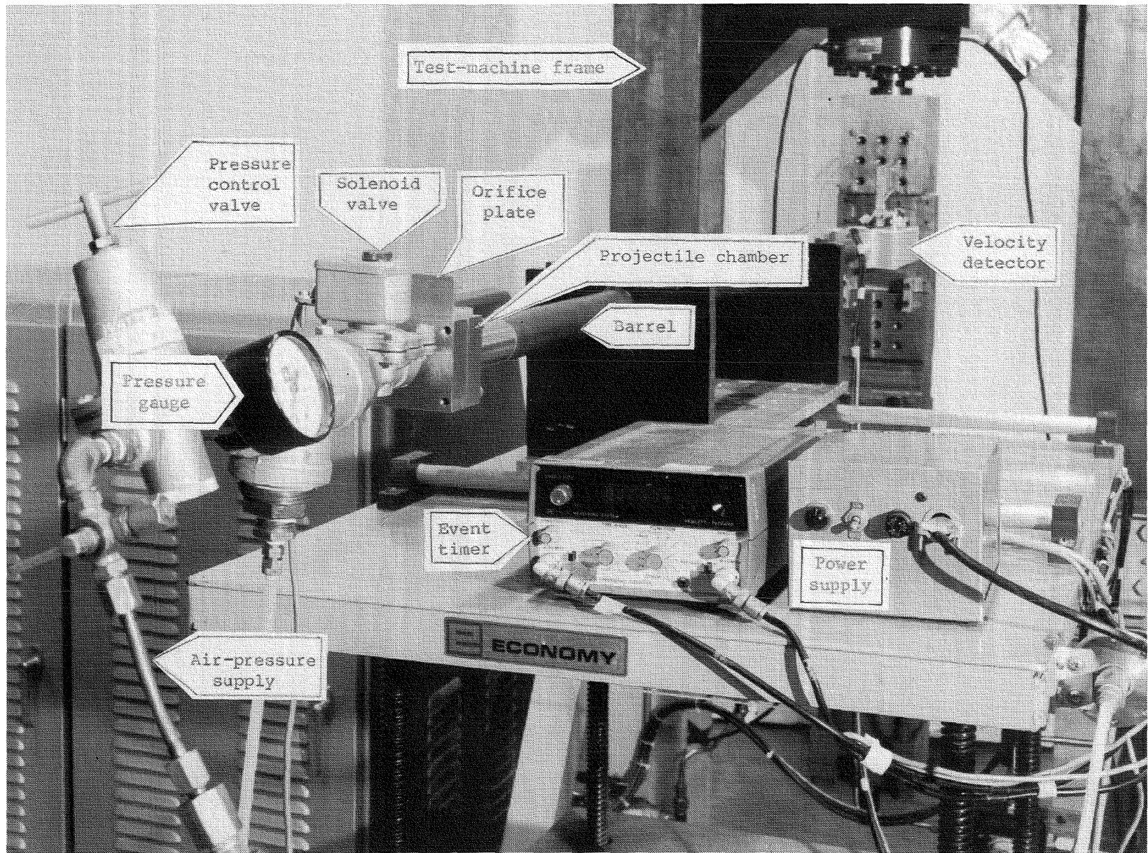
(a) Air-driven impact gun.
