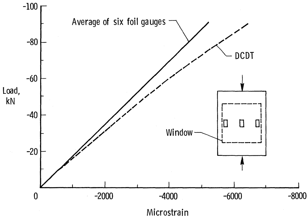
(b) Compression.
