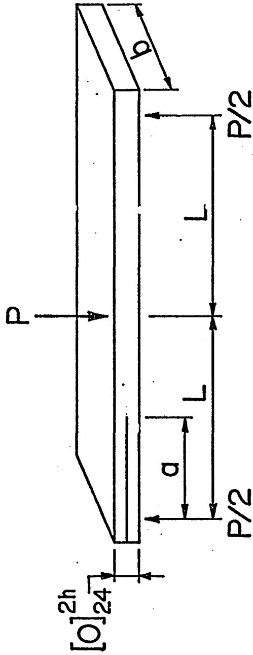
Fig. 1. End Notch Flexure Specimen
