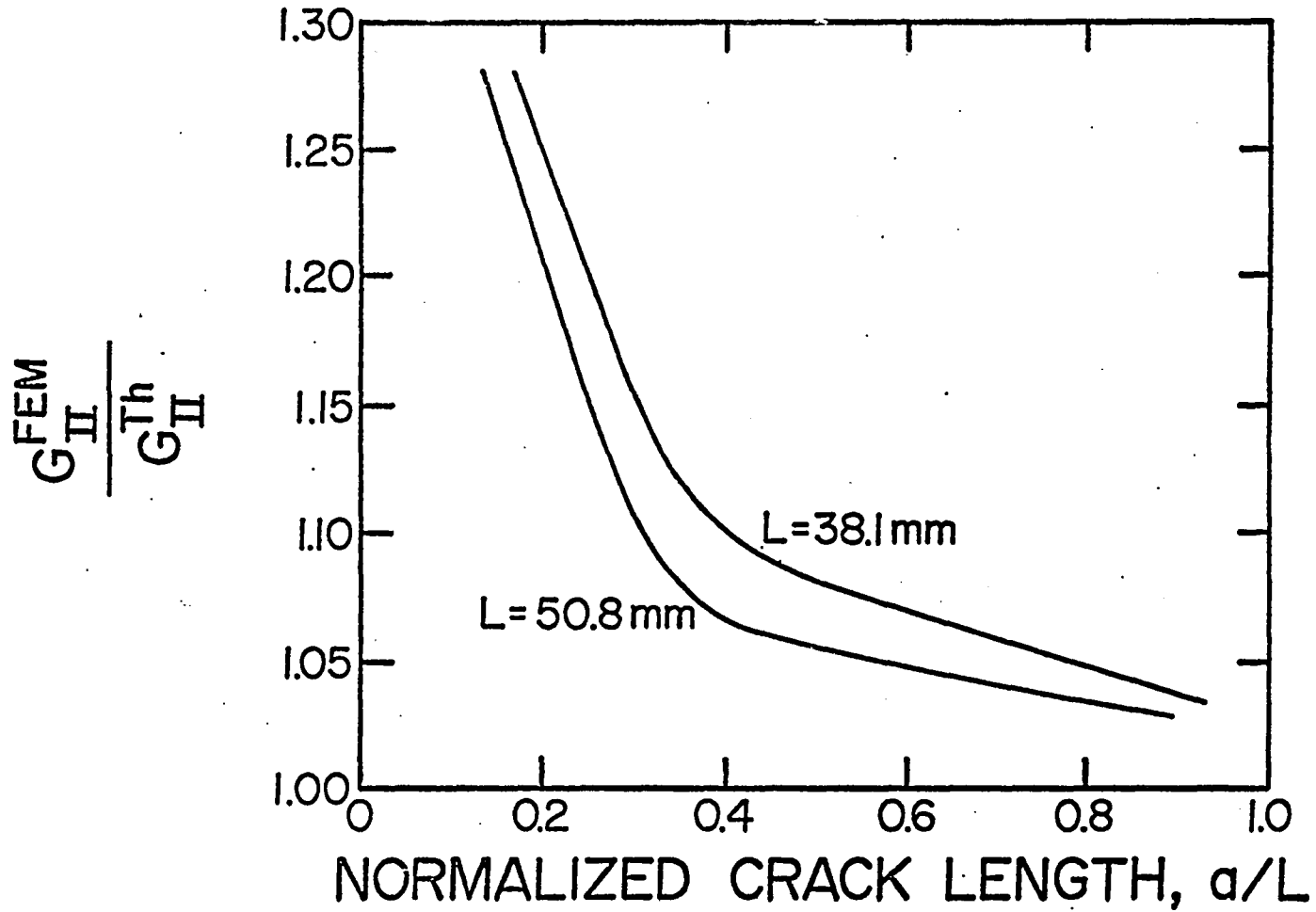
Fig. 3. Ratio of G_{II} from FEM analysis to G_{II} from Eq. (1) as a function of normalized crack length.
