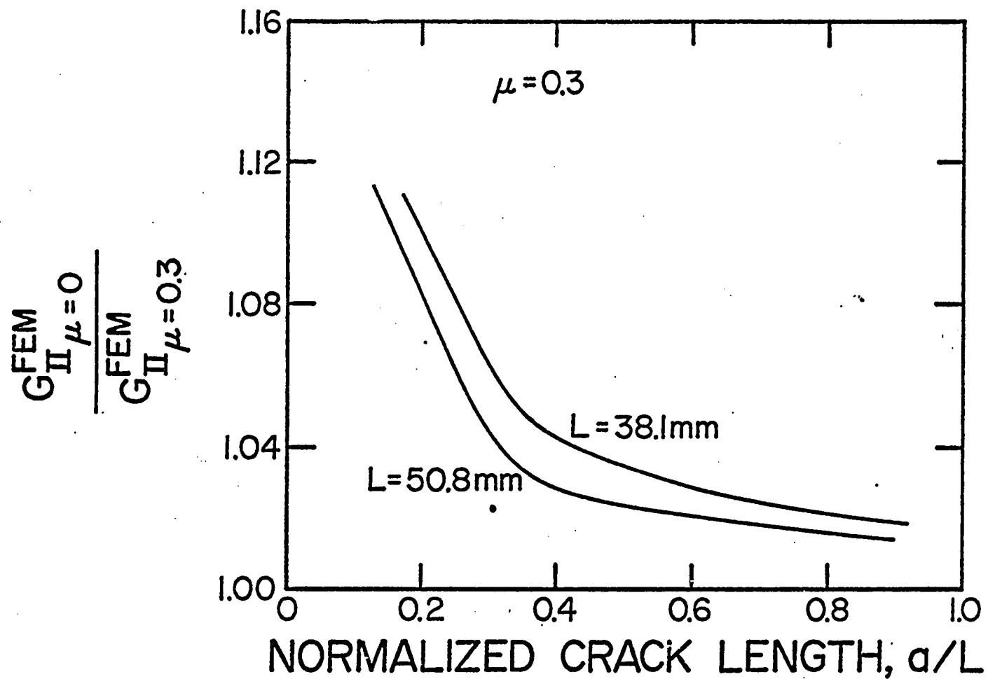
Fig. 4 (b). Ratio of G_{II} with \mu = 0.0 to G_{II} with \mu = 0.3 from FEM analysis as a function of normalized crack length.
