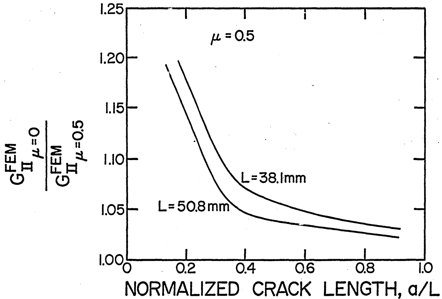
Fig. 4 (c). Ratio of G_{II} with \mu = 0.0 to G_{II} with \mu = 0.5 from FEM analysis as a function of normalized crack length.
