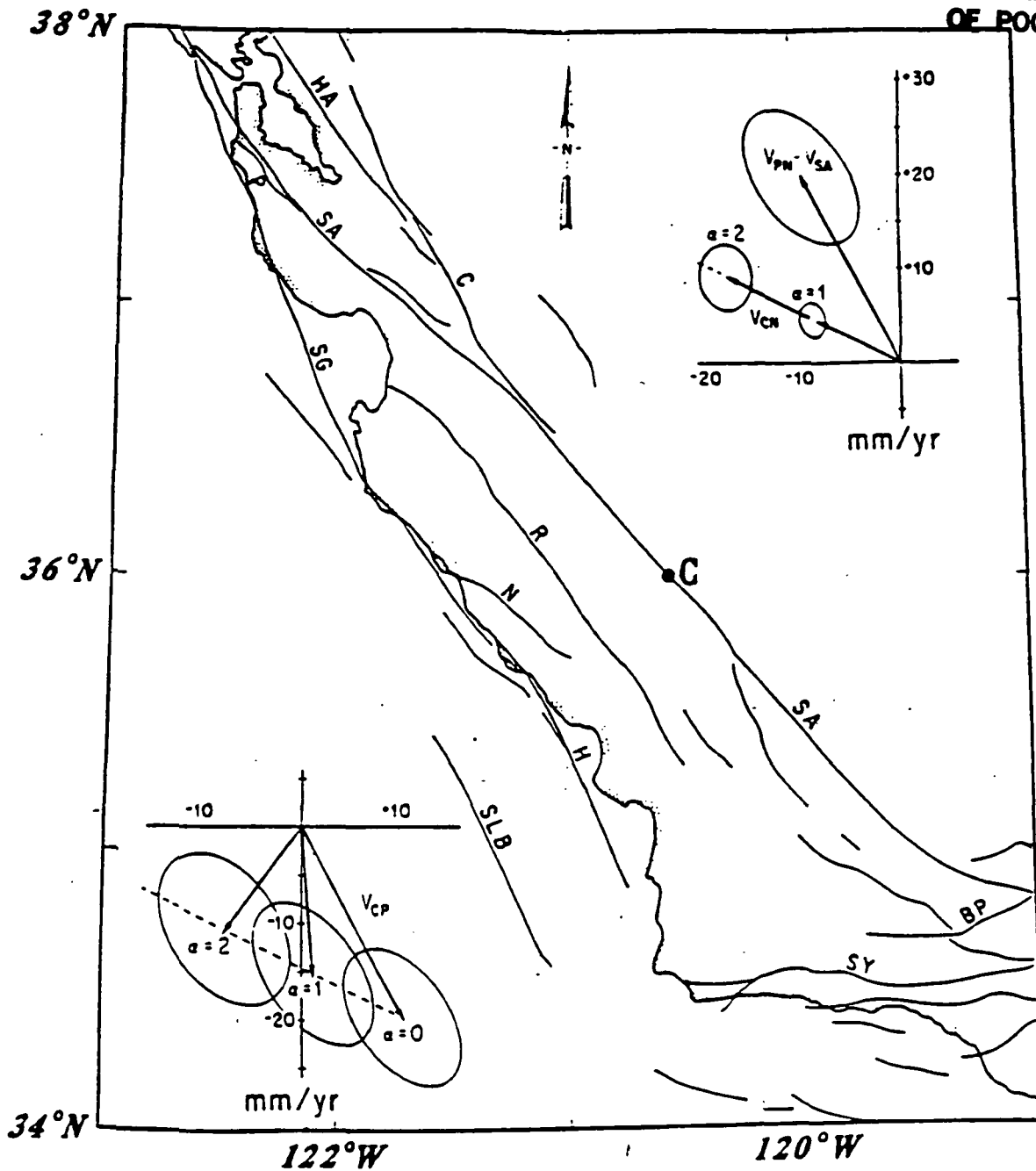
Fig. 2: Map: Lambert conformal conic projection of central California showing major zones of Quaternary faulting (S). Lettered fault zones are the Big Pine (BP), Calaveras (C), Hosgri (H), Nachimiento (N), Pilarcitos (P), Rinconada (R), San Andreas (SA), San Gregorio (SG), Santa Lucia Bank (SLB), and Santa Ynez (SY). C is the fiducial point at 36°N on the San Andreas used in vector calculations. Upper inset: Velocity diagram in the tangent plane at C showing discrepancy vector V_{PN} - V_{SA} and vector V_{CN}(\alpha) describing Basin-and-Range deformation; \alpha = 1 corresponds to an opening rate of exactly 10 mm/yr across the Great Basin along line AB in Fig. 1. Error ellipses are two-sigma. Lower inset: Velocity diagram at C showing V_{CP} , which describes deformation west of the San Andreas. Dashed line is locus parameterized by \alpha . Error ellipses are two-sigma.
