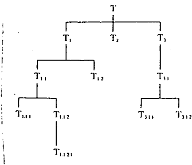
Figure 2. Synthesis tree
