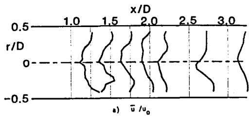
Fig. 4. Time-Mean Velocity with \phi = 45 Degrees, Traverse Angle \theta = 0 Degrees
