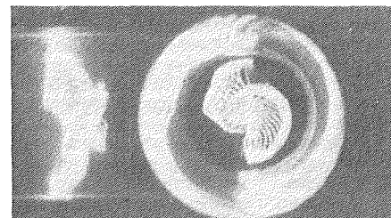
Fig. 3 Spark-gap flow visualization for jet/cross-flow velocity ratio = 4.0
