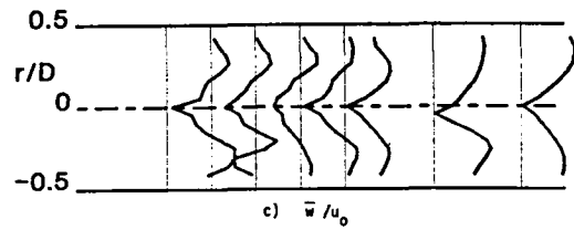
Fig. 5. Time-Mean Velocity with \phi = 45 Degrees, Traverse Angle \theta = 330 Degrees
