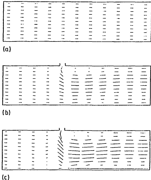
Fig. 6 Velocity vectors showing magnitude and direction in rx-plane through lateral jet with nonswirling main flow and velocity ratio R = v_j/u_0 of: (a) 0 (b) 2 (c) 4.
