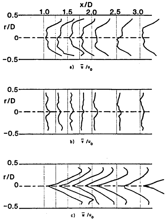
Fig. 13. Time-Mean Velocity with \phi = 70 Degrees, Traverse Angle \theta = 270 Degrees
