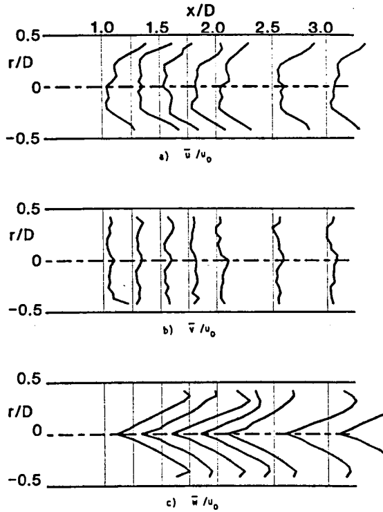
Fig. 10. Time-Mean Velocity with \phi = 70 Degrees, Traverse Angle \theta = 0 Degrees
