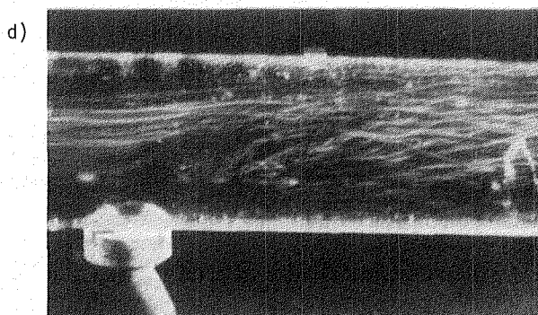
Fig. 10 Neutrally-buoyant helium-filled soap bubble visualization with velocity ratio R of: (a) 0 (b) 2 (c) 3 (d) 4 (e) 6 (f) 8
