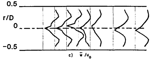
Fig. 7. Time-Mean Velocity with \phi = 45 Degrees, Traverse Angle \theta = 270 Degrees
