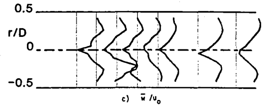
Fig. 6. Time-Mean Velocity with \phi = 45 Degrees, Traverse Angle \theta = 300 Degrees
