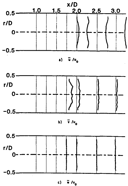
Fig. 9. Time-Mean Velocity with \phi = 0 Degrees (Swirler Removed) Traverse Angle \theta = 270 Degrees.
