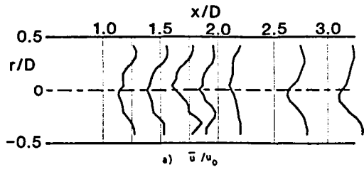
Fig. 6. Time-Mean Velocity with \phi = 45 Degrees, Traverse Angle \theta = 300 Degrees
