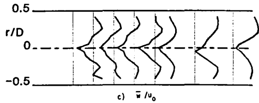
Fig. 4. Time-Mean Velocity with \phi = 45 Degrees, Traverse Angle \theta = 0 Degrees
