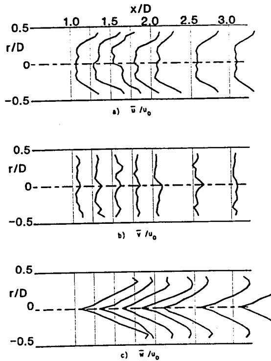
Fig. 11. Time-Mean Velocity with \phi = 70 Degrees, Traverse Angle \theta = 330 Degrees
