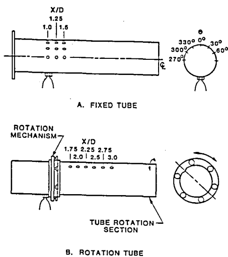
Fig. 3. Test Sections
