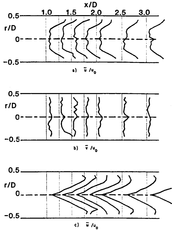
Fig. 12. Time-Mean Velocity with \phi = 70 Degrees, Traverse Angle \theta = 300 Degrees
