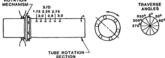
Fig. 2. Test Section
