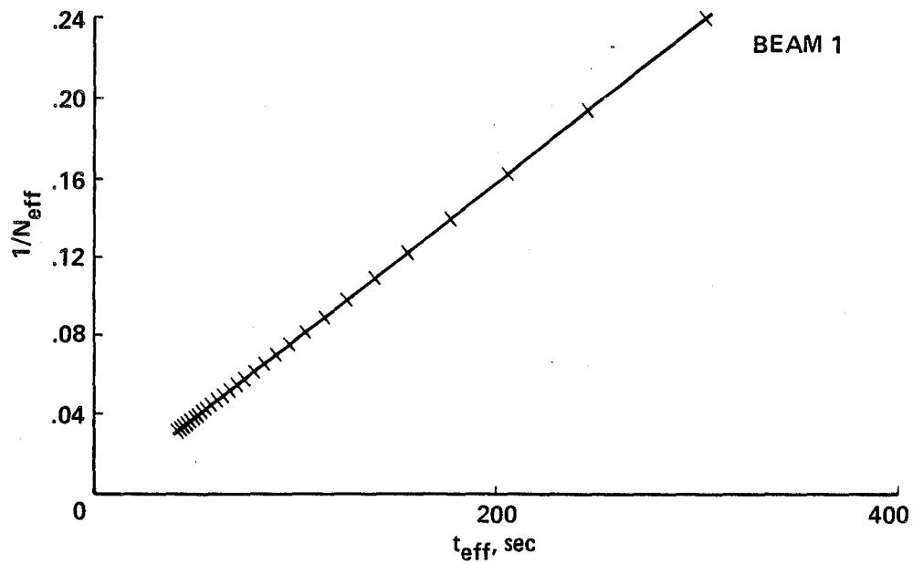
(c) Fit of fringe-time history to lubrication theory, from fringes identified in figure 6b, using subroutine SCCFIT.
