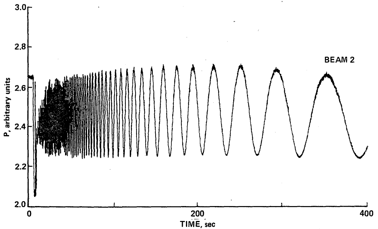
(a) Before processing. Note that the signal quality on each beam is equal, as provided by this design.
