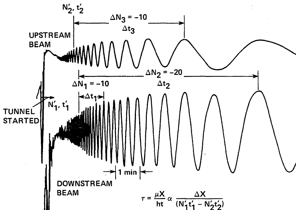
Figure 3.- Monson's oil film interferometer. (a) Monson's optical system (fig. 1 from ref. 14) showing major components. (b) Typical signal from Monson's instrument (fig. 2) from ref. 14), with data-reduction equations.
